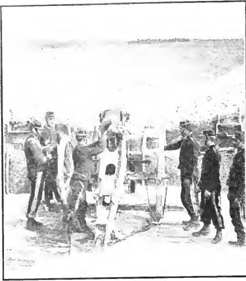
FRENCH FORTRESS ARTILLERY. Charging a 95 mm. gun.
