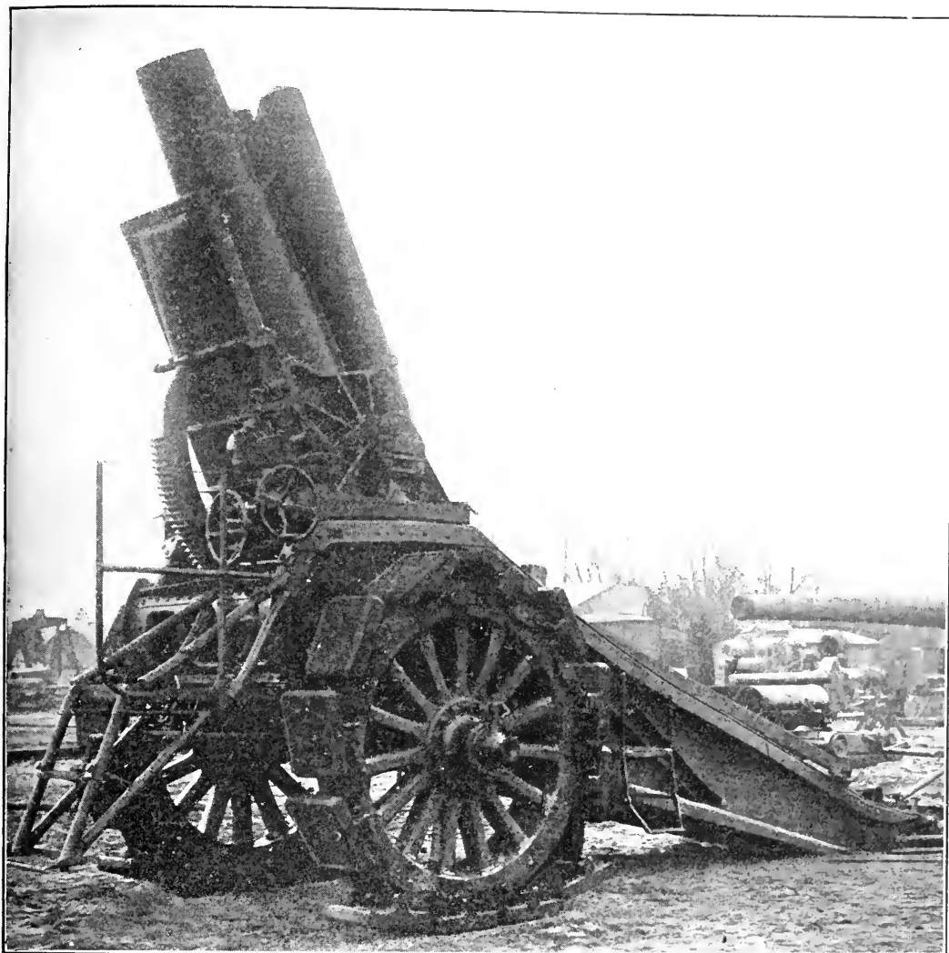
GERMAN SIEGE HOWITZER.
