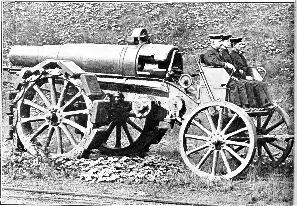
AN 11-in. GERMAN MORTAR.
