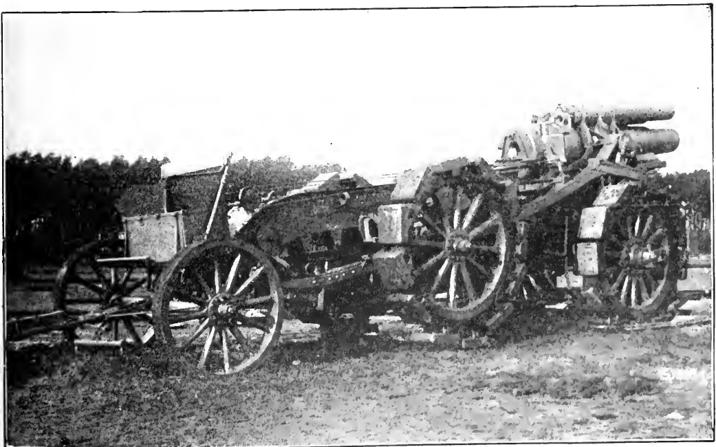
GERMAN SIEGE GUN IN TRANSIT.
