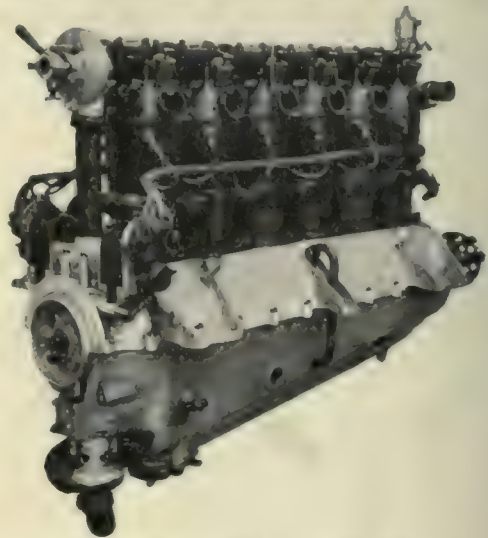
MERCEDES 180-h.p. ENGINE.
