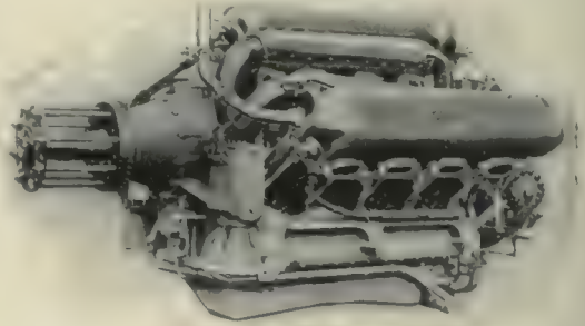
NAPIER LION 450-h.p. ENGINE.
