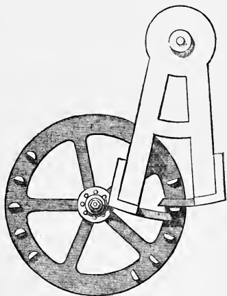
French Single-Pin Escapement.
