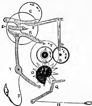
Rack Striking Work.
