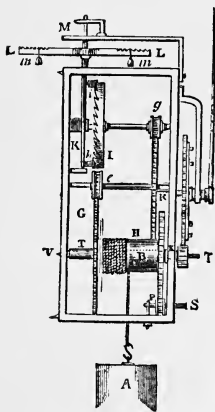
Old Balance-Clock.
