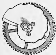
Hour-Wheel and Snail.
