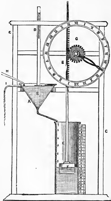
The Clepsydra, or Water-Clock of the Greeks.
