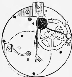
Back of French Clock.
