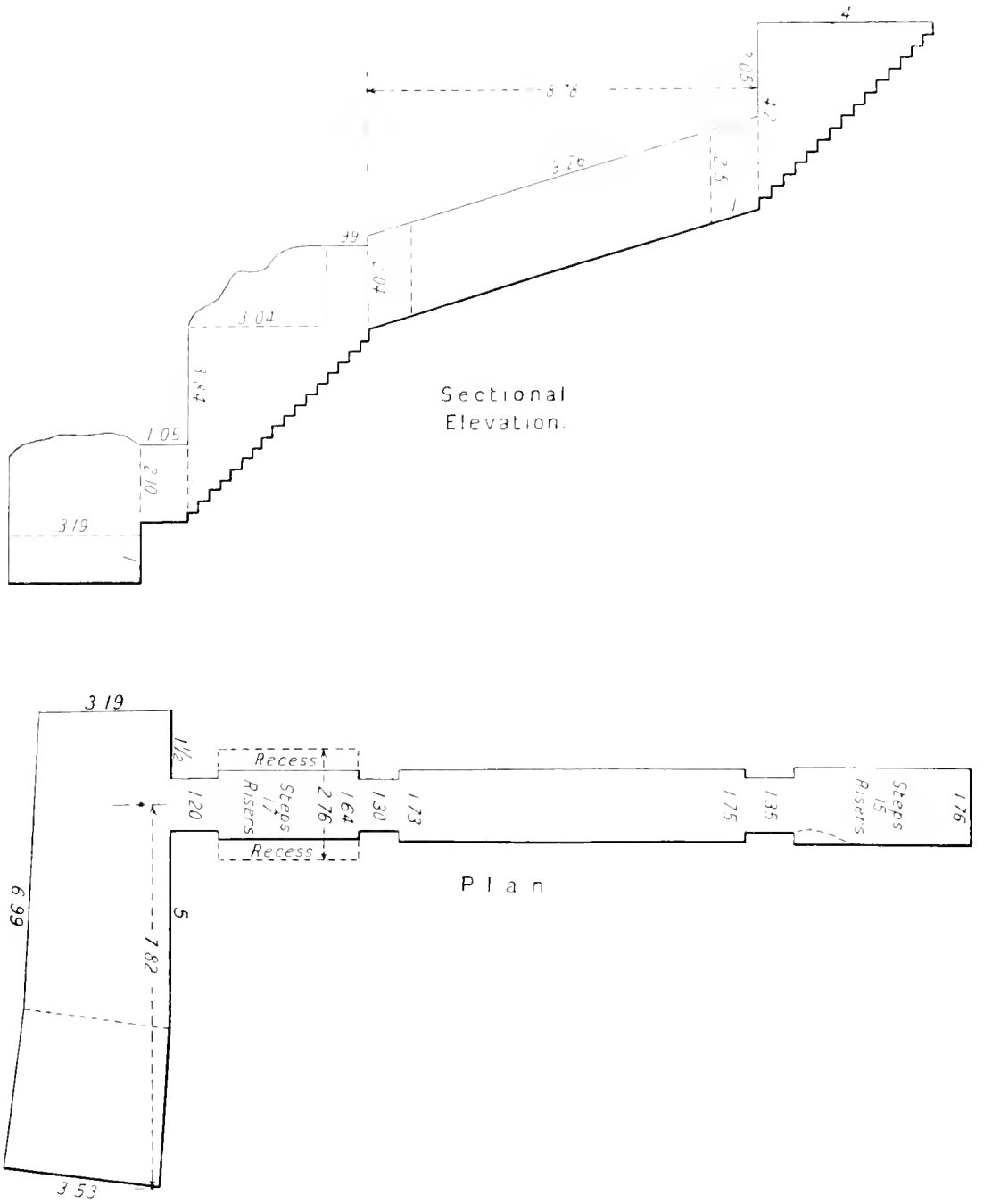
PLAN AND SECTIONAL ELEVATION OF THE TOMB.
