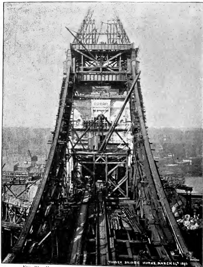
FIG. 34. PROGRESS OF ERECTION OF MAIN CHAINS. LONG SEGMENT.
