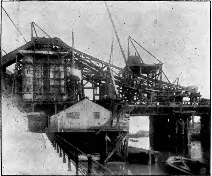
FIG. 33. PROGRESS OF ERECTION OF MAIN CHAINS. SHORT SEGMENT.]
