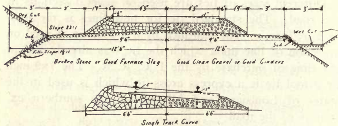
Lehigh Valley Track Section.
