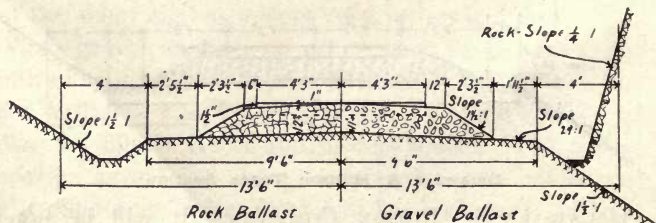
Rock Ballast Gravel Ballast Erie Track Section.
