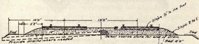
Crushed Rock and Slag—Class A.
