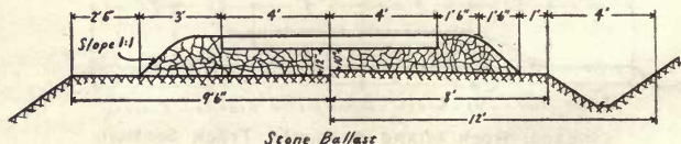
Stone Ballast Chicago, St. Paul, Minneapolis & Omaha Track Section.
