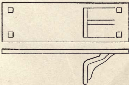
Fig. 13. Stop Rail Brace.
