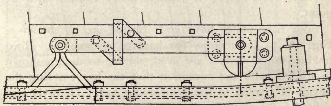
Fig. 5. Combination Anti-Creep Hold-Down and Stop.
