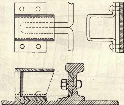
Fig. 8. Holding Down Device.
