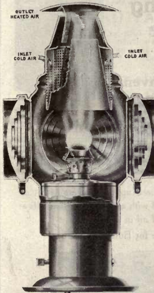
Sectional view of Adlake Non-Sweating Ventilation Showing Direction of Air Currents.
