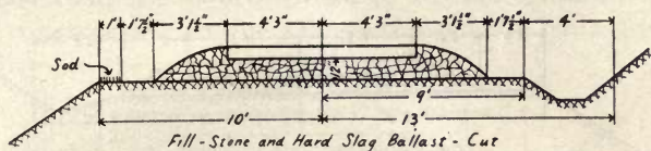
Baltimore & Ohio Track Section.
