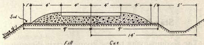
Wabash Track Section.
