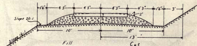
Delaware & Hudson Track Section.
