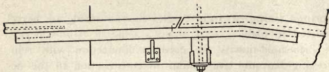
Fig. 6. Anti-Creeper Hinge Rail.
