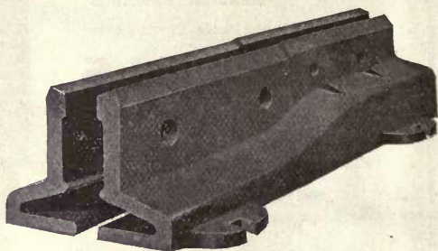
Continuous Step or Compromise Joint
