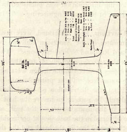
Series A—Proposed 80-lb. Rail Section.
