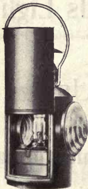
Interior View Semaphore Lamp Showing Prism Glass Reflector.
