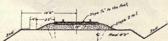
Crushed Rock and Slag—Class A.
