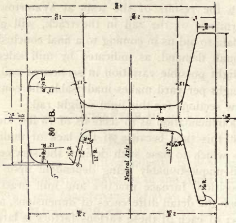
Series B—Proposed 80-lb. Rail Section.
