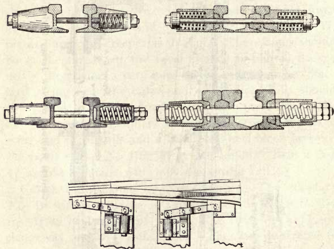
Fig. 2. Springs.
