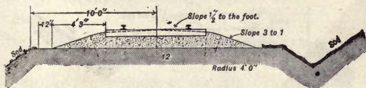
Gravel, Cinders, Chats, etc.—Class A.
