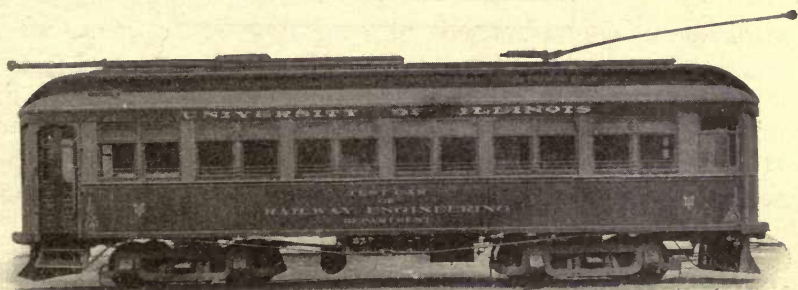
FIG. 1. THE TEST CAR
