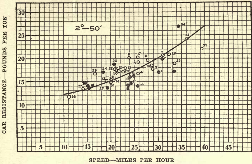
FIG. 5. THE RELATION OF RESISTANCE TO SPEED ON THE 2^{\circ}-50' CURVE
