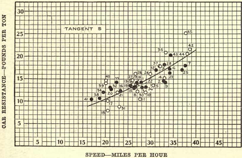
FIG. 6. THE RELATION OF RESISTANCE TO SPEED ON TANGENT S, WHICH PERTAINS TO THE 2^{\circ}-50' CURVE
