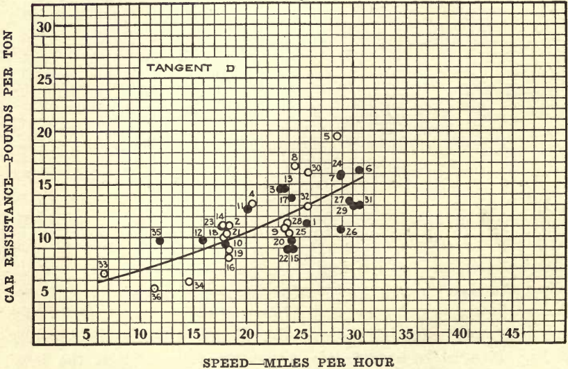
FIG. 11. THE RELATION OF RESISTANCE TO SPEED ON TANGENT D, WHICH PERTAINS TO THE 6°-30' CURVE
