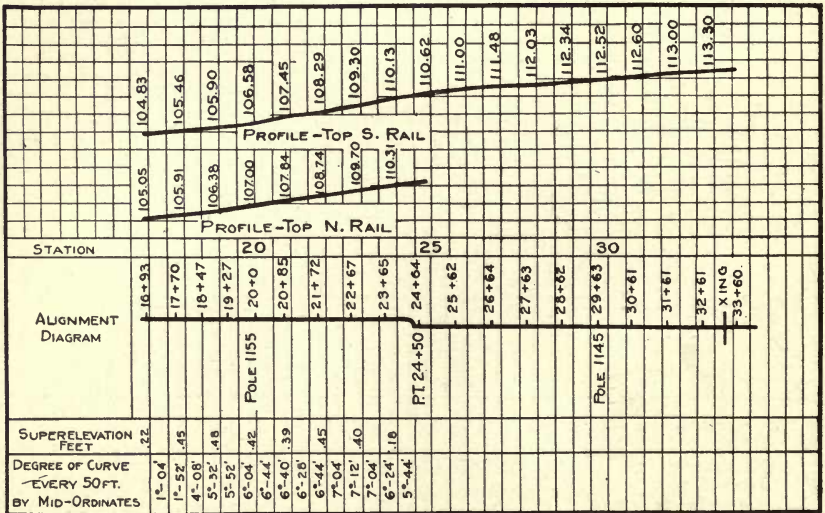
FIG. 23. PROFILE AND ALIGNMENT DIAGRAM OF THE TRACK ON THE 6°-30' CURVE
