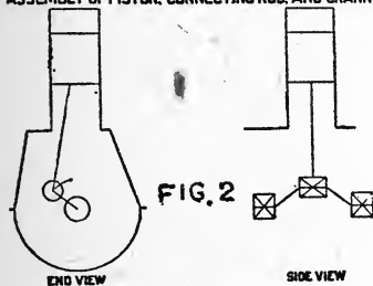
Fig. 2. The heat engine resolved into its simplest elements.
