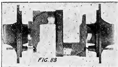
Fig. 113. Crank shaft, showing how the oil is carried to the bearings on Leader tractor engine.
