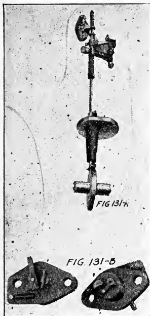
Fig. 131. Low tension igniter on Rumely tractor.
