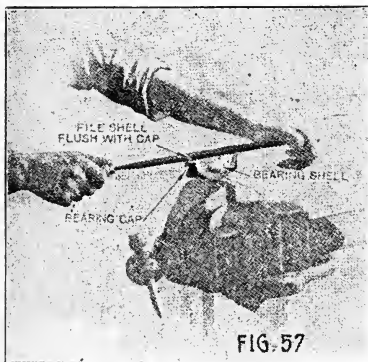
Fig. 57. Method of adjusting bearing by filing off cap slightly.
