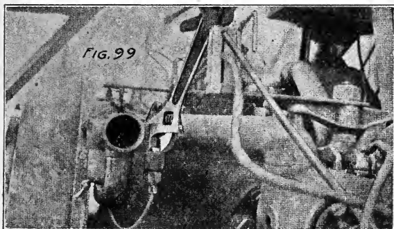
Fig. 99. Adjusting leaky carburetor.
