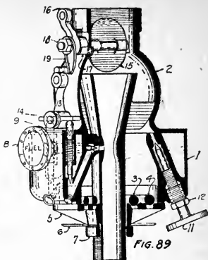
Fig. 89. Sectional view of Linga Vaporizer.
