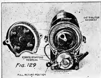
Fig. 129. Distributor construction.
