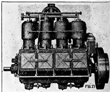
Fig. 21. 7\frac{1}{4} \times 9 four-cylinder Twin City oil engine.
