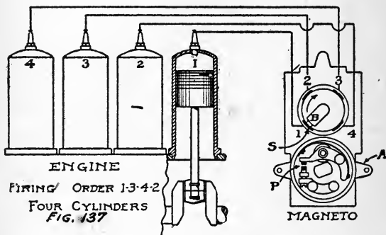
Fig. 137. Timing K-W magneto to a four-cylinder engine.
