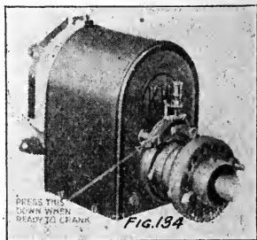
Fig. 134. Impulse starter on K-W magneto.
