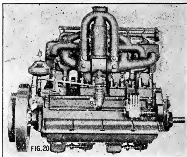
Fig. 20. 7\frac{1}{4} \times 9 , four-cylinder Twin City oil engine. Valve side.
