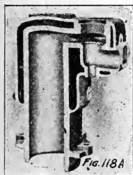
Fig. 118-A. Section showing cylinder jacket.
