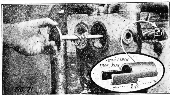
Fig. 71. 2d. Remove valve spring by turning engine over until the spring is compressed to its utmost. Place a short piece of gas pipe (sawed as per illustration) between the spring and crank case to hold spring in a compressed condition, then turn motor over until the key can be removed from the valve stem. It is not necessary to remove the spring when grinding.
