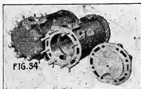
Fig. 34. Rumely cylinders and cylinder head.
