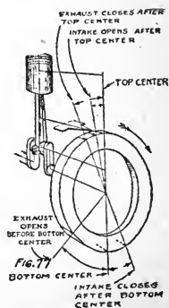
Fig. 77. Timing engine by flywheel markings (Twin City).
