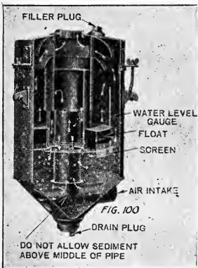
Fig. 100. A typical tractor air washer.
