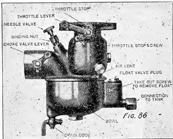
Fig. 86. Carburetor from Case 10-18 tractor.
