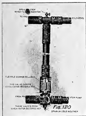
Fig. 120. Syphon regulator showing path of circulation.
