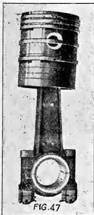
Fig. 47. Typical piston and connecting rod assembly for tractor.
