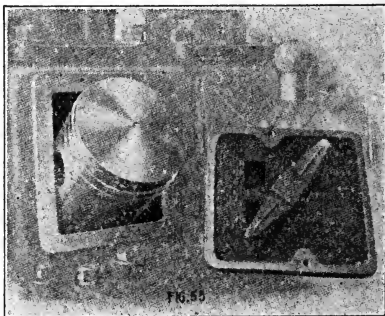
Fig. 55. Removing piston and rod assembly through inspection opening on Best engine.
