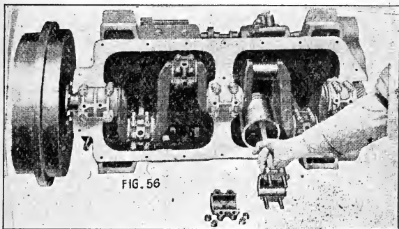
Fig. 56. Lower crank case removed, showing main bearings, connecting rod and bearing, and the ease with which piston is removed in Waukesha engine.
