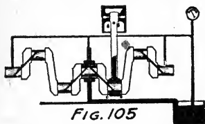
Fig. 105. Force feed system.
