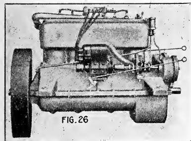
Fig. 26. Kermath engine used in Light-foot tractor.
