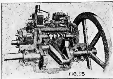
Fig. 15. Crank-case with cover removed from Rumely 14-28 engine.
