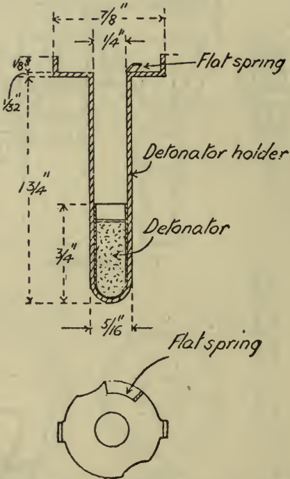
FOR NO. 1 (SERVICE HAND GRENADE).
