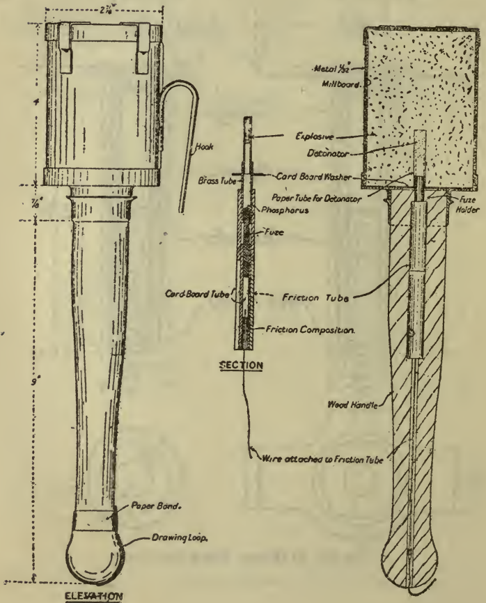
Fig. 2. Section.
