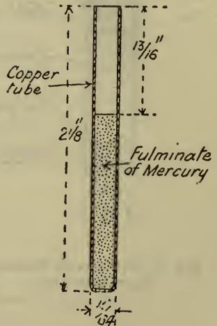
Fig. 8. No. 8 Detonator.
