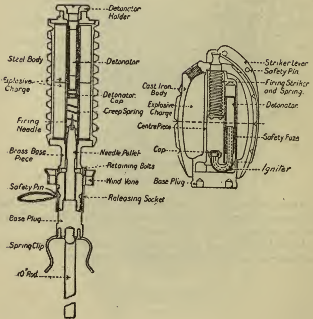
GRENADE, HAND. No. 5. FIG. 2.
