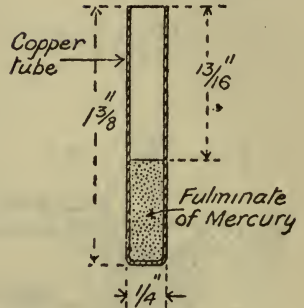
Fig. 8. No. 8 Detonator.
