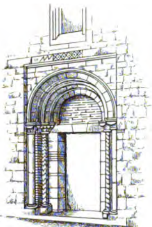
North and South Doorway at A.B. 1/2 Scale.
