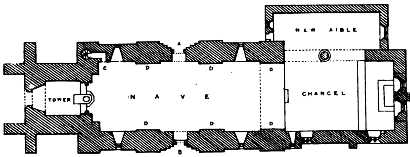
P l a n 32 Feet to an Inch
