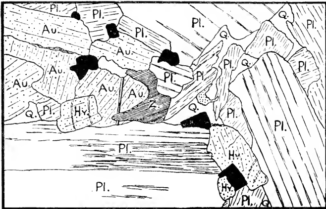
DIAGRAMMATIC SKETCH ( \times 45 ) ILLUSTRATING RELATIONS OF ZOISITE TO OTHER MINERALS, AND GENERAL STRUCTURE. (See Plate XXVIII, fig. 1.)
