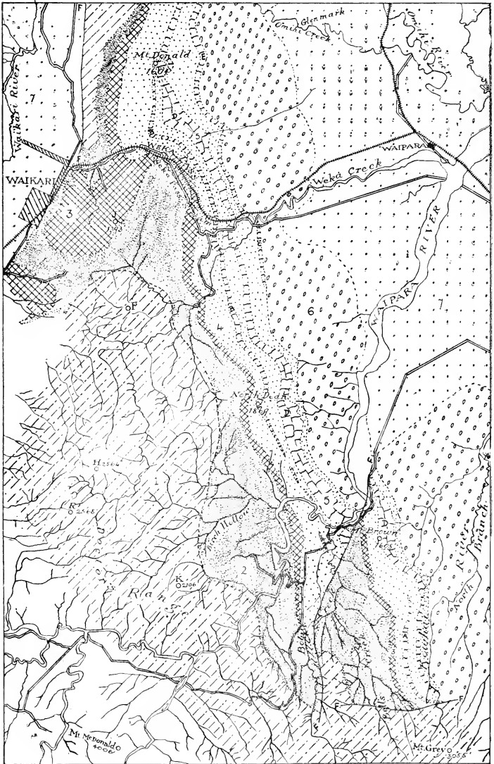
FIG. 1.—Geological map of the Middle Waipara and Weka Pass district. Scale, \frac{1}{2} in. to one mile. The sides of the map are N. 71 E. 1, Pre-Notocene. 2, Piripauan. 3, Amuri limestone and Weka Pass stone. 4, "Grey marls" and sands interbedded with 5, Mount Brown limestones. 6, Greta and Kowhai beds. 7, Notopleistocene (alluvial plains).
