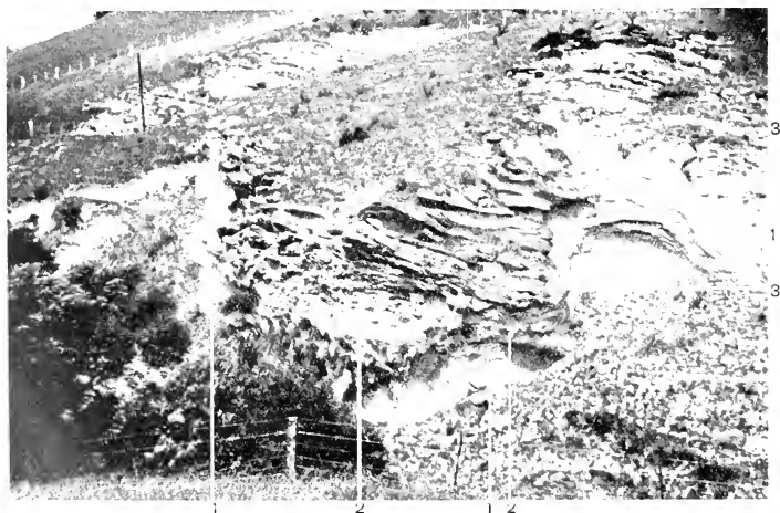
FIG. 2.—Cliff in Weka Pass Stream, below railway-cutting, 43\frac{3}{4} miles from Christchurch. A fault with downthrow to the left intersects the cliff. 1, grey sandstone (top of "grey marls"); 2, hard calcareous conglomerate with shells; 3, lower Mount Brown limestone (B).
