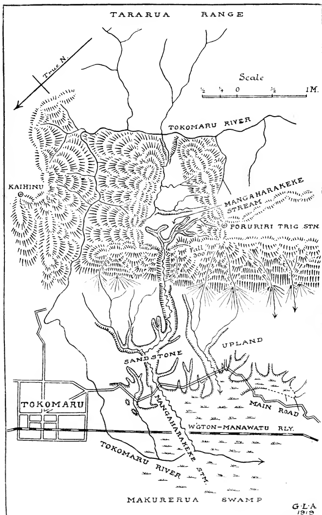
FIG. 3.—The topography of the present and former catchment areas of the Mangaharakeke Stream, near Tokomaru.
