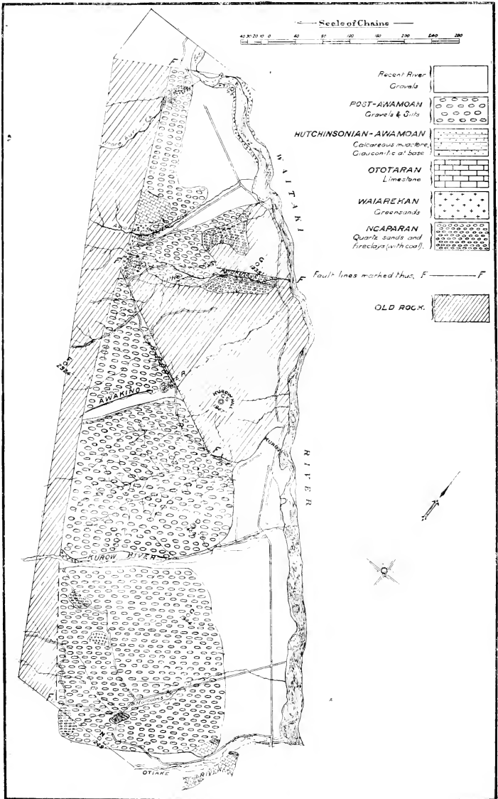
FIG. 1.—Geological map of the Waitaki Valley between Wharekuri and Otiake River, North Otago.
