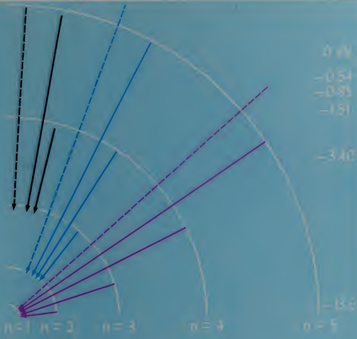
Lyman Series
