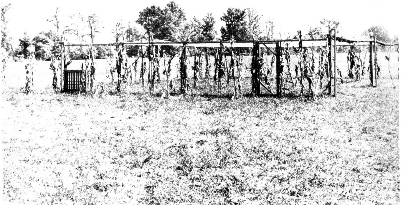
Fig. 2.--Section type drop-curtain trap in use at the Horseshoe Lake Game Refuge. Top netting shown here is made of twine, thereby eliminating the need for support posts inside the trap.
