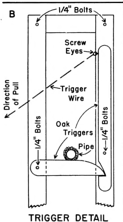
Fig. 3.--Construction details for drop-curtain type section trap and for holding box.
