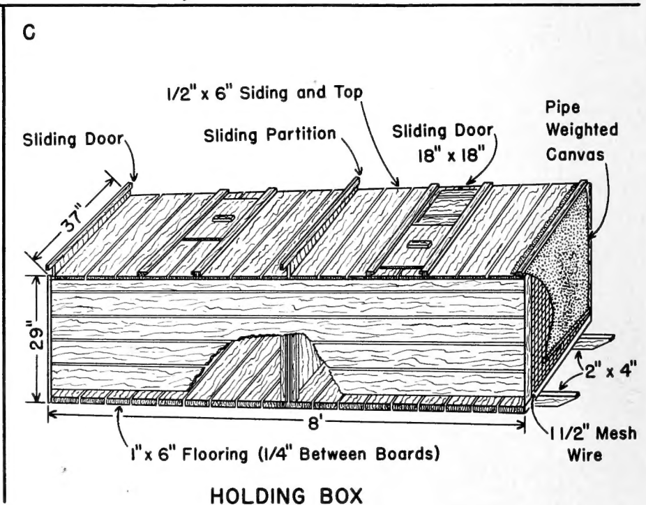
Fig. 3.--Construction details for drop-curtain type section trap and for holding box.
