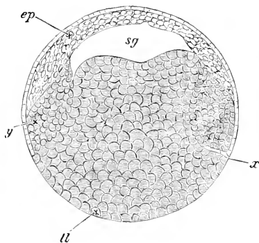
FIG. 41. SECTION THROUGH FROG'S OVUM AT THE CLOSE OF SEGMENTATION. sg , segmentation cavity. ll , large yolk-containing cells. ep , small cells at formative pole (epiblast).
