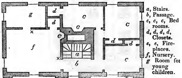
Fig. 24. Second Story.
