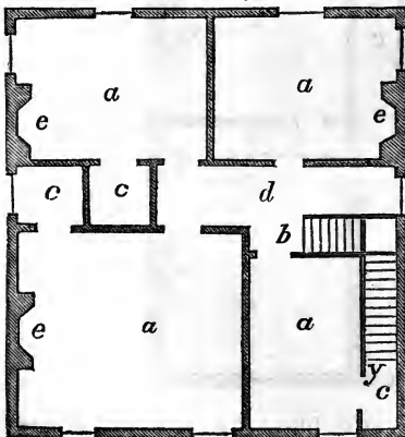
Fig. 28. Second Story.
