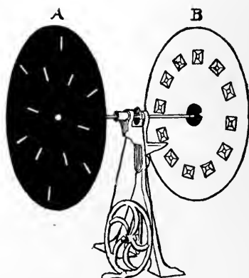
Fig. 54.—The Stereostroboscope.
