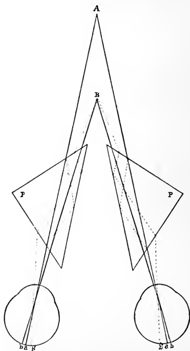
Fig. 55.—Wheatstone's Pseudoscope.
