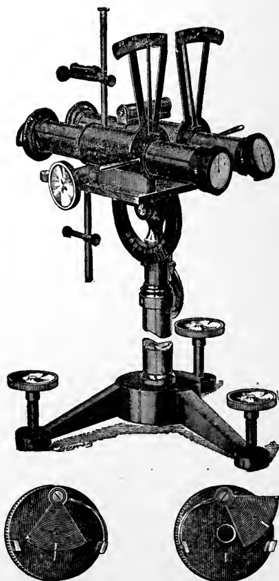
Fig. 95.—The Clinoscope.
