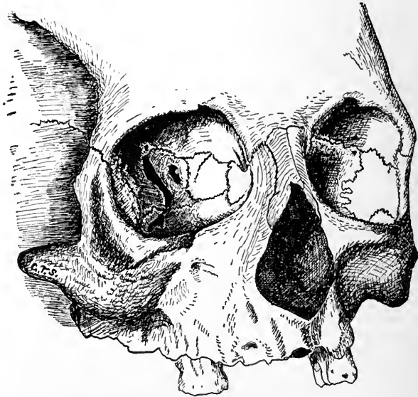
Fig. 5.—The Orbits.
