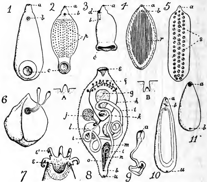
FIG. X.—Some Malacocotyleans.
