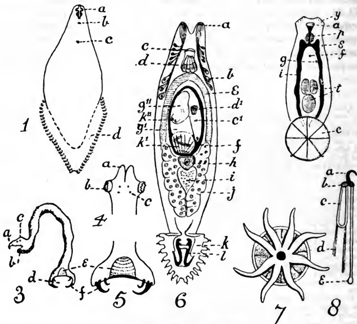
FIG. III.—Heterocotyleans.
