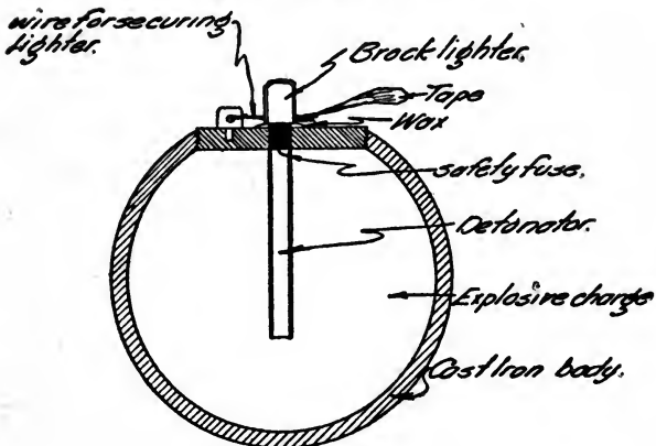
SECTION. Diameter of Grenade 3" BALL HAND GRENADE.
