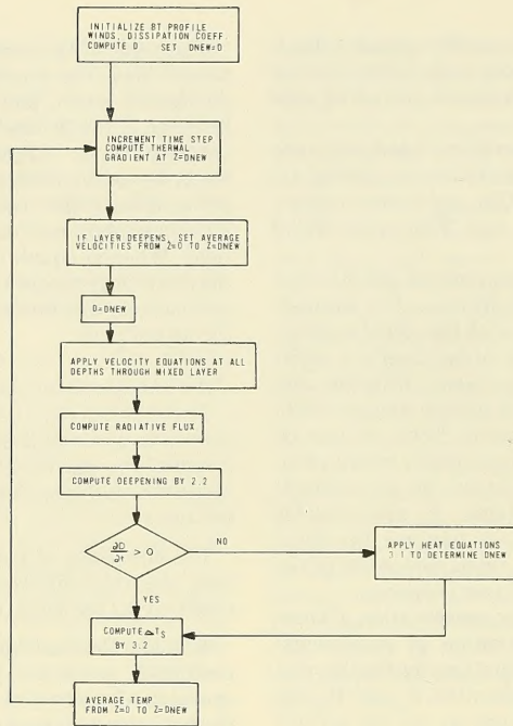
Figure 3.1 Flowchart of the Model Computational Scheme.
