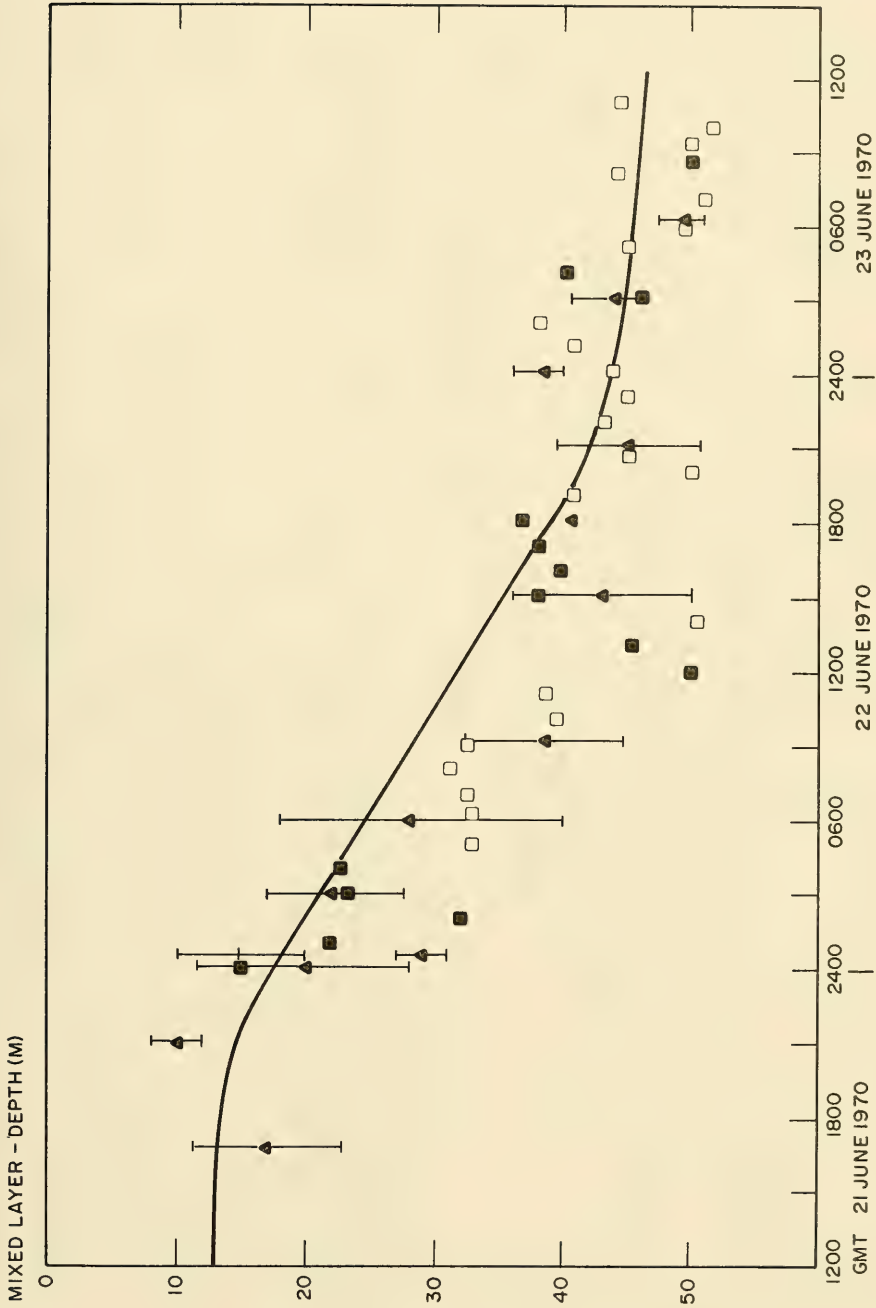
Figure 4.1 Deepening of the mixed layer during a Gaussian shaped storm.
