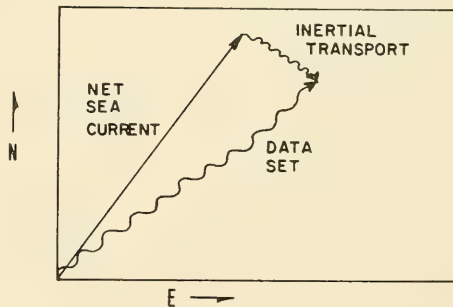
Figure 4.5 Lagrangian view of solution for Net Sea Current.
