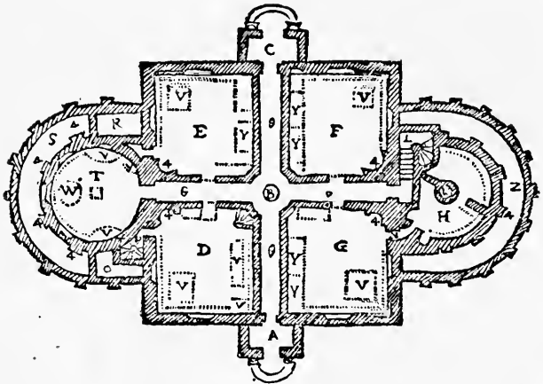
PLAN OF THE GROUND FLOOR OF URANIBORG.
