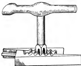
Hempel iron quoin with its turnkey.
