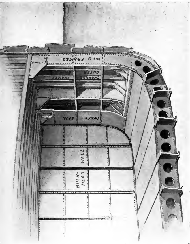
THIS DRAWING SHOWS HOW THE PLATING OF THE INNER BOTTOM OF SUCH A SHIP AS THE TITANIC MAY BE CARRIED UP THE SIDE FRAMES TO FORM AN INNER SKIN
