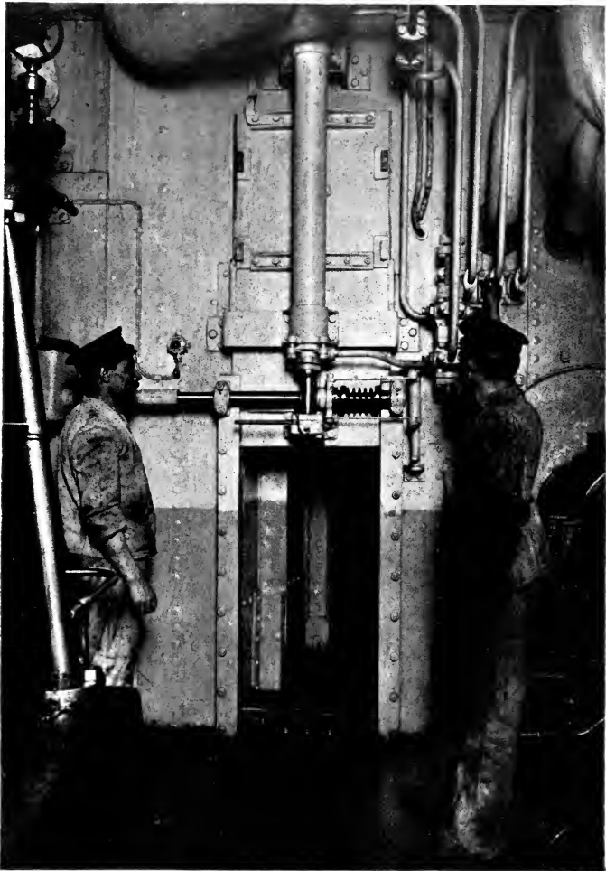
HYDRAULICALLY-OPERATED, WATERTIGHT DOOR IN AN ENGINE-ROOM BULKHEAD
