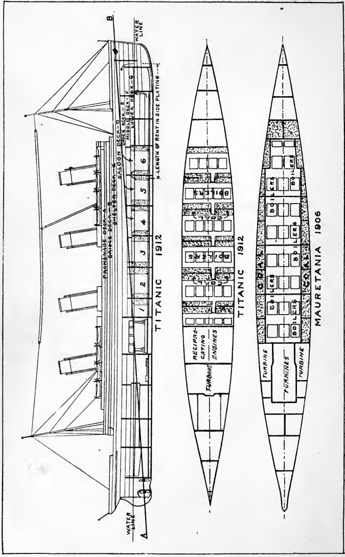
Titanic : Single skin, 16 compartments; Mauretania ; double skin, 34 compartments. COMPARISON OF SUBDIVISION IN TWO FAMOUS SHIPS
