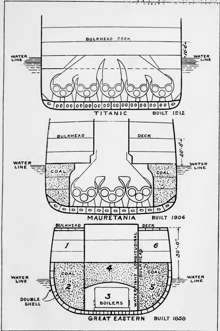
TWO EXTREMES IN PROTECTION, AND A COMPROMISE
