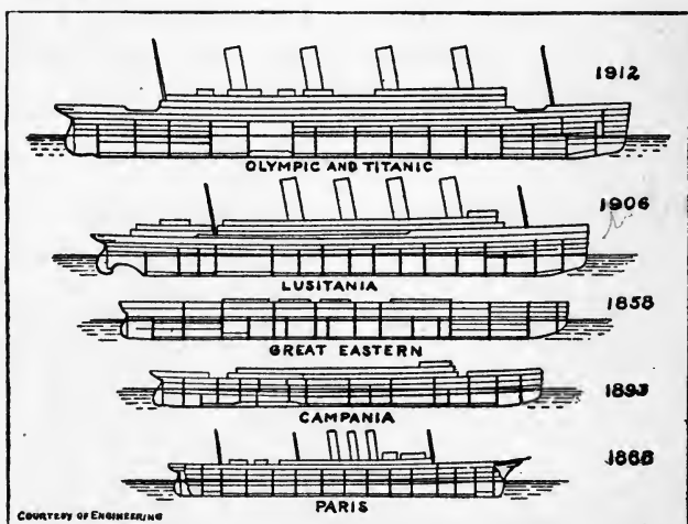
A COMPARISON OF BULKHEAD PROTECTION IN SOME NOTABLE SHIPS
