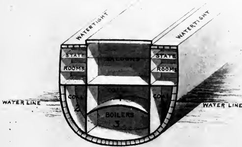
GREAT EASTERN 1858 FOUR WATERTIGHT COMPARTMENTS
