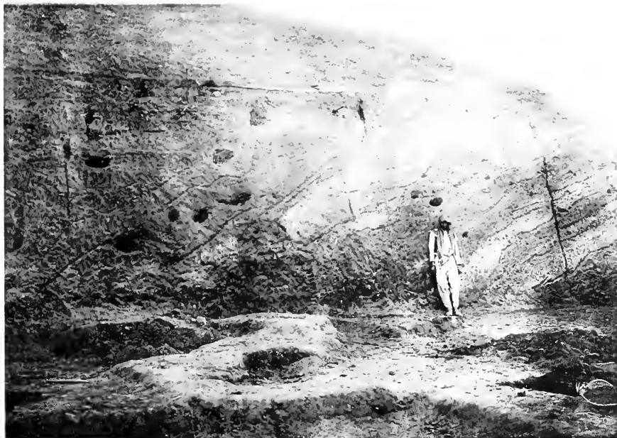
a. THE EARTH FACE OF THE SOUTH CORNER OF THE EXCAVATED AREA, SHOWING THE STRATIFICATION OF THE RUBBISH MOUNDS v. p. 220
