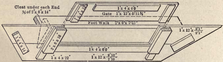
FIG. 42.—Border gate of wood used in Sacramento Valley, Cal.
