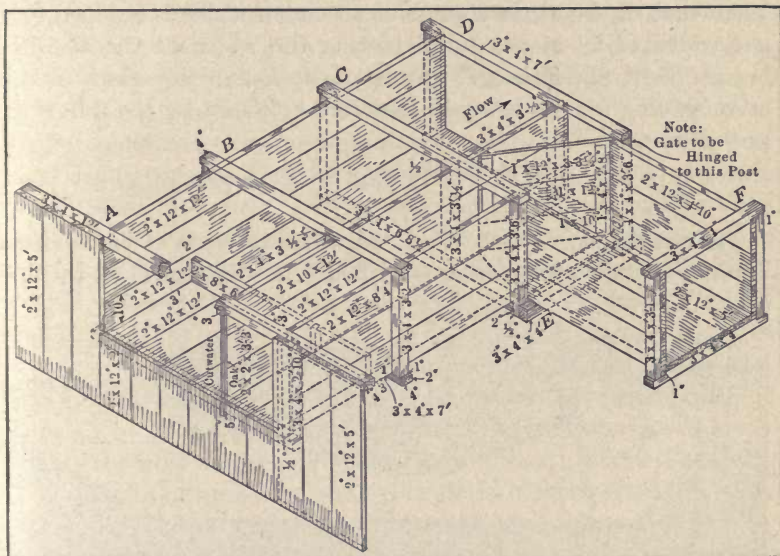
FIG. 52.—Design for proportional division box.
