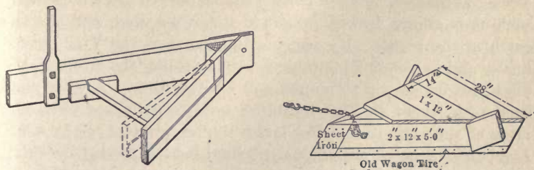
FIG. 5.—V-crowders used in building farm ditches.
