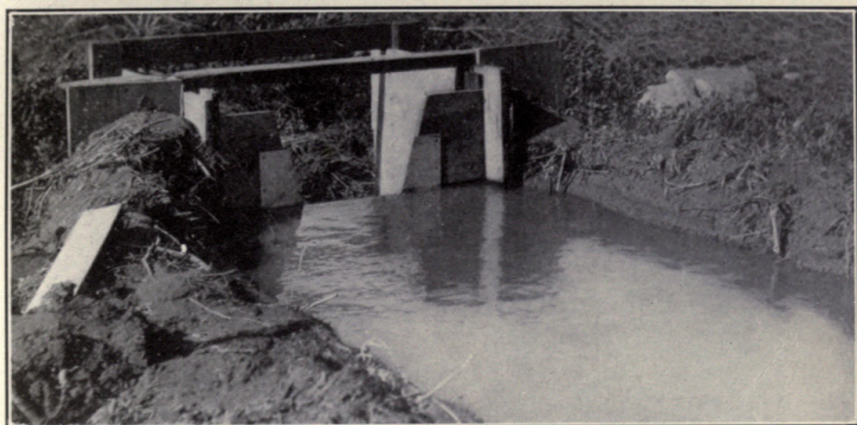
FIG. A.—Downstream view of trapezoidal weir wire in use.
