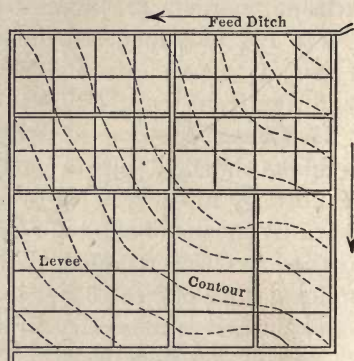
FIG. 46.—Rectangular checks on field shown in Fig. 45.
