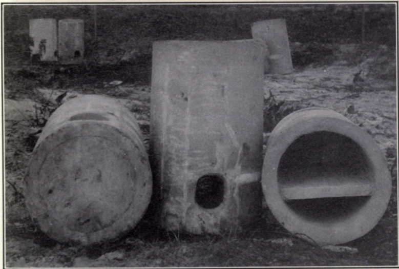
FIG. C.—Details of stop-boxes.
