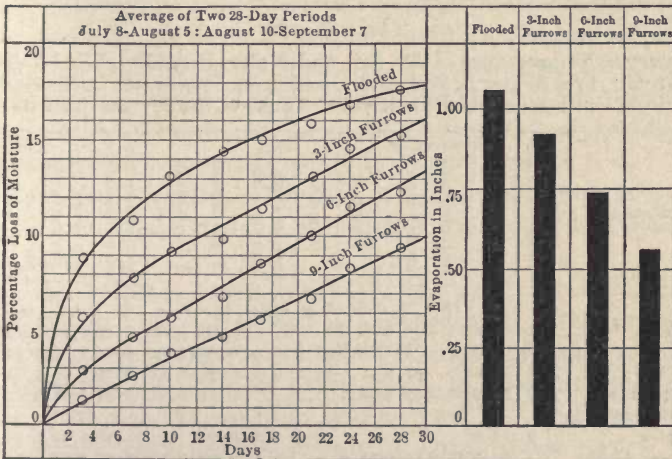
FIG. 59.—Average evaporation losses from tanks irrigated by flooding and with furrows of different depths at Reno, Nevada, July 8 to Aug. 5 and Aug. 10 to Sept. 7, 1909.
