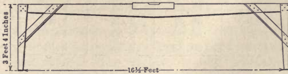
FIG. 4.—Home-made level for locating ditches.
