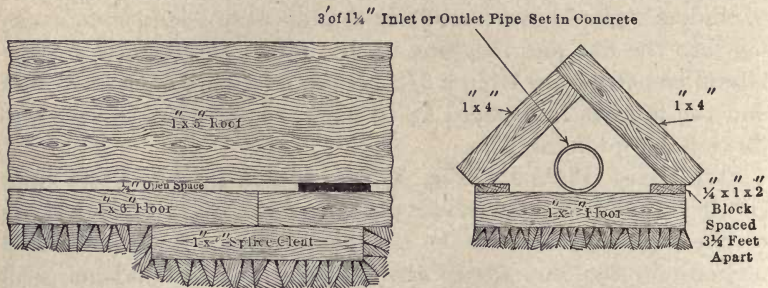
FIG. 49.—Wooden conduits for combined drainage and irrigation.
