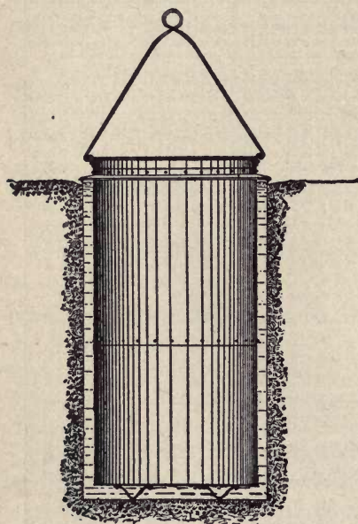
FIG. 55.—Design of tank used in evaporation experiments.
