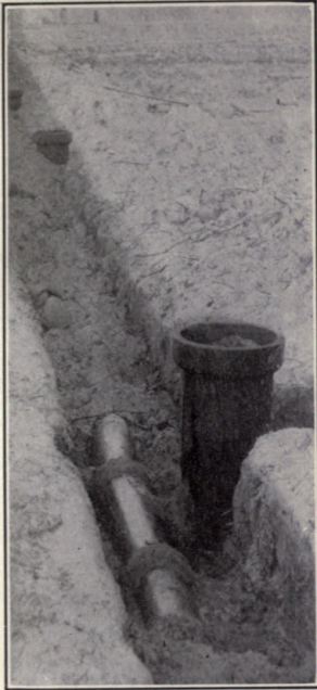
FIG. A.—Main line and stop-boxes for subirrigation systems
