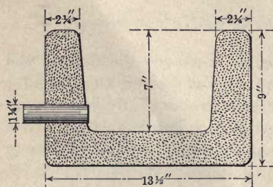
FIG. 30.—Concrete head flume with opening.
