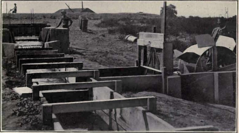
FIG. A.—Testing Australian meter against standard weir.
