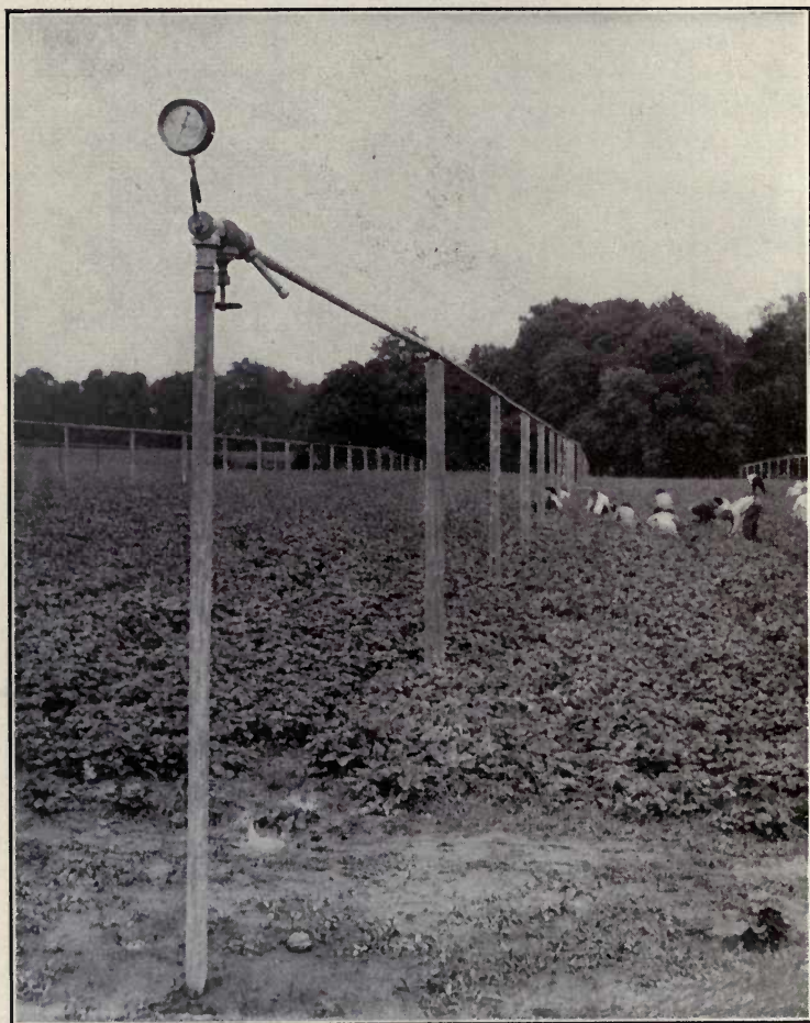
FIG. B.—Enlarged view of overhead nozzle line.
