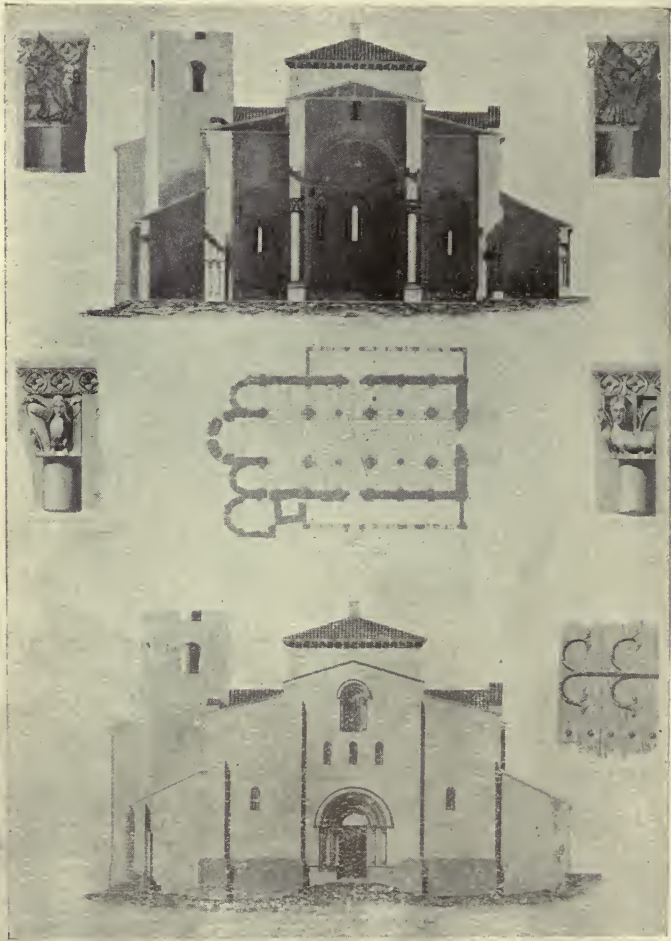
PLAN, AND DETAILS OF THE PARISH CHURCH OF SAN MILLÁN SEGOVIA
