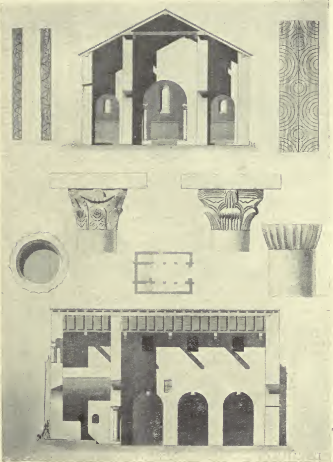
PLAN, SECTIONS, AND DETAILS OF SAN ADRIAN DE TUÑON (CONCEJO DE VILLANUEVA) PROVINCE OF OVIEDO
