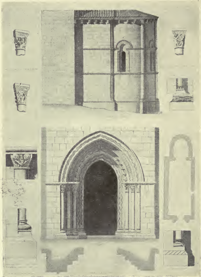
PLAN, PRINCIPAL ENTRANCE, AND DETAILS OF THE CHURCH OF SAN JUAN DE AMANDI (CONCEJO DE VILLAVICIOSA) PROVINCE OF OVIEDO
