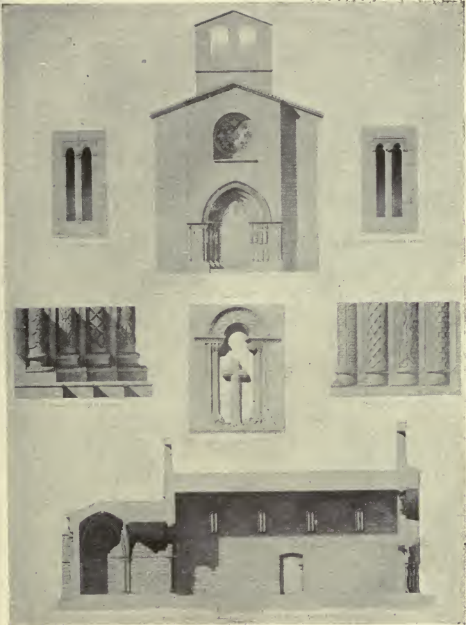
FRONT, LONGITUDINAL SECTION, AND DETAILS OF THE PARISH CHURCH OF VILLAVICIOSA (CONCEJO DE VILLAVICIOSA) PROVINCE OF OVIEDO
