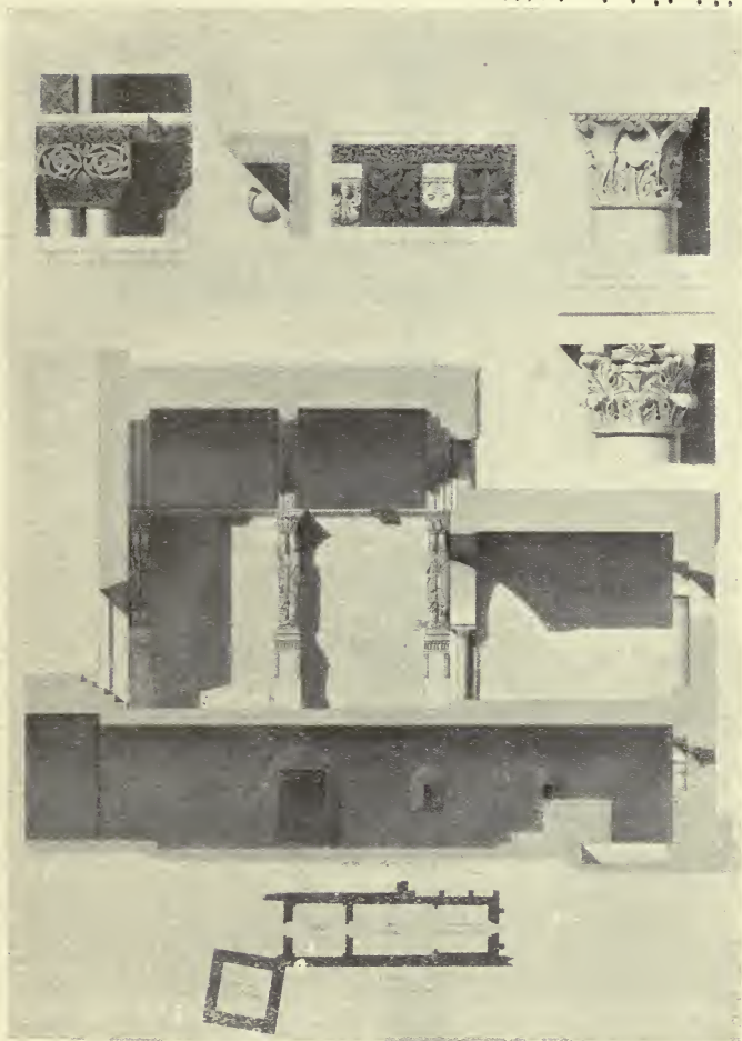
SECTION, PLAN, AND DETAILS OF THE CAMARA SANTA IN THE CATHEDRAL OVIEDO
