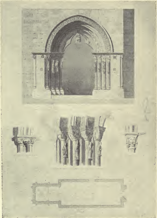
PLAN, PORCH, AND DETAILS OF THE PARISH CHURCH OF VILLAVICIOSA (CONCEJO DE VILLAVICIOSA) PROVINCE OF OVIEDO
