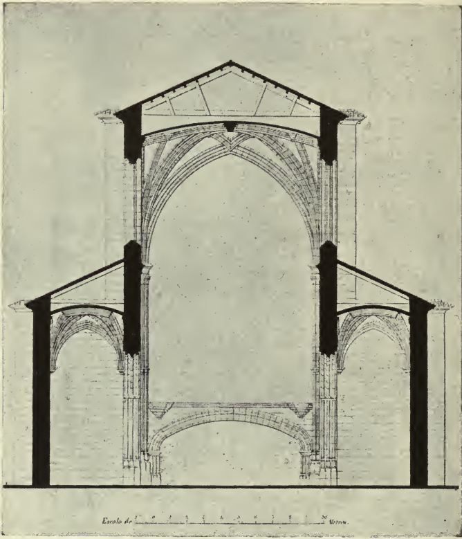
SECTION OF THE CONVENT OF SANTO TOMÁS AVILA
