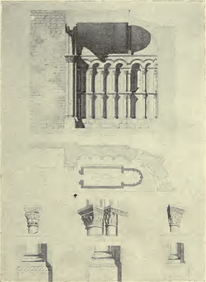
PLAN, LONGITUDINAL SECTION, AND DETAILS OF THE PARISH CHURCH OF SAN JUAN DE AMANDI (CONCEJO DE VILLAVICIOSA) PROVINCE OF OVIEDO
