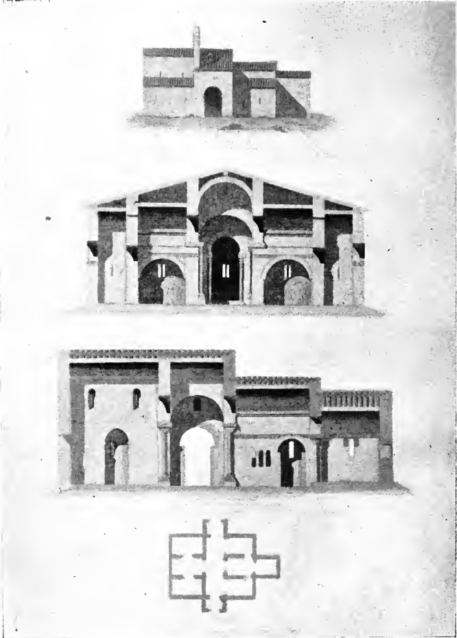
PLAN AND SECTIONS OF THE PARISH CHURCH OF ST. PETER ZAMORA
