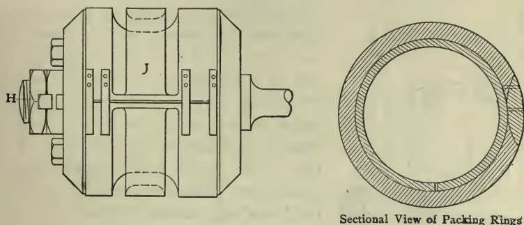
Sectional View of Packing Rings
