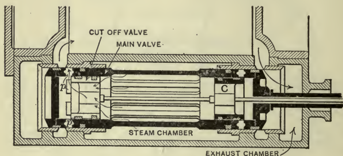
FIG. 101. — PISTON VALVE.
