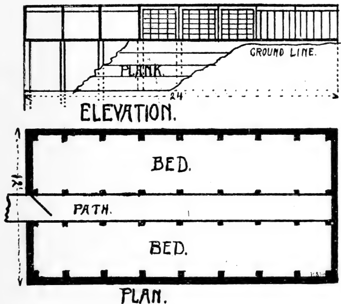
Figure 28.—Plan and elevation of hotbed greenhouse.
