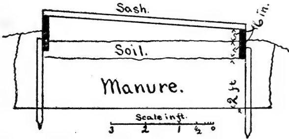
Figure 25.—Cross section of hotbed.
