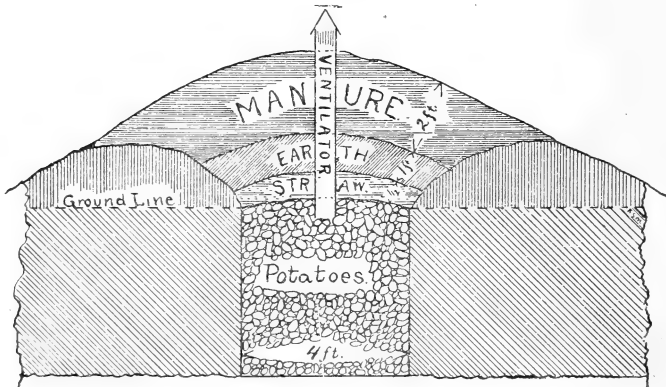
Figure 98.—Potatoes pitted for winter.
