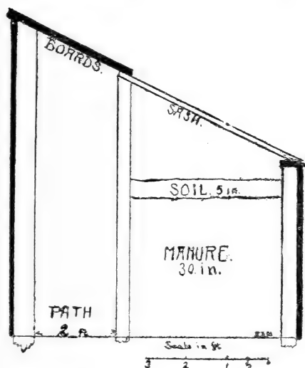
Figure 30—Cross section of lean-to greenhouse hotbed.
