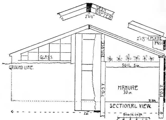
Figure 29.—Sectional view of hotbed greenhouse.
