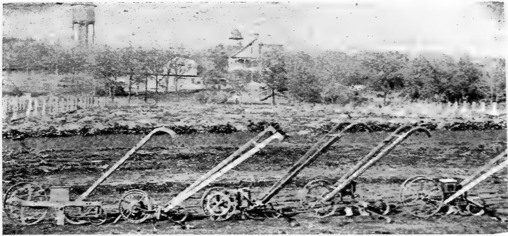
Figure 8.—Garden drills. (1) A. H. Mathews. (2) Planet Jr. combined drill. (3) Mathews combined drill. (4) New Model drill. (5) Planet Jr. Hill Dropping drill.
