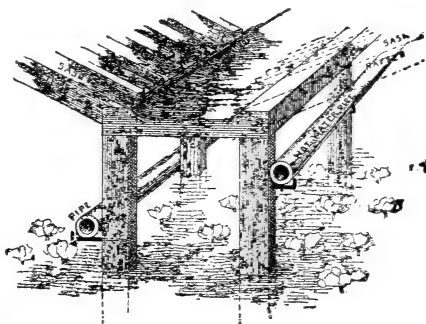
Figure 32.—Valley in market gardeners' greenhouse showing the way the sashbars are attached to the plate.
