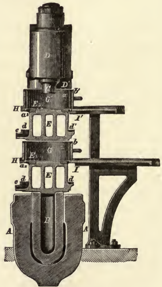
FIG. 32. Hydraulic Pan Press (Side View and Section).
