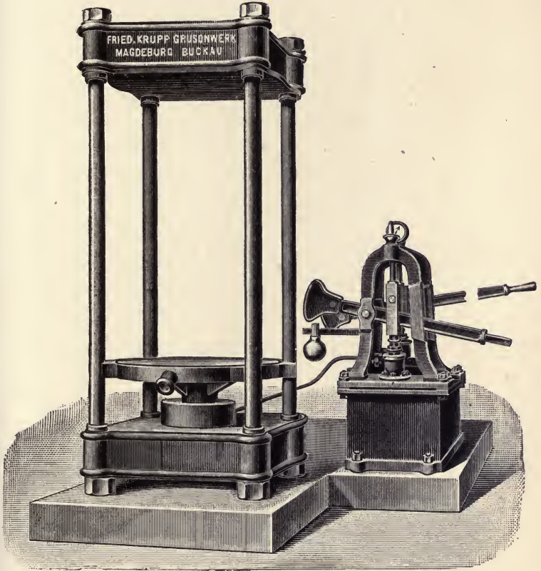
FIG. 39. Preliminary Press for Oil Fruits (Fr. Krupp).
