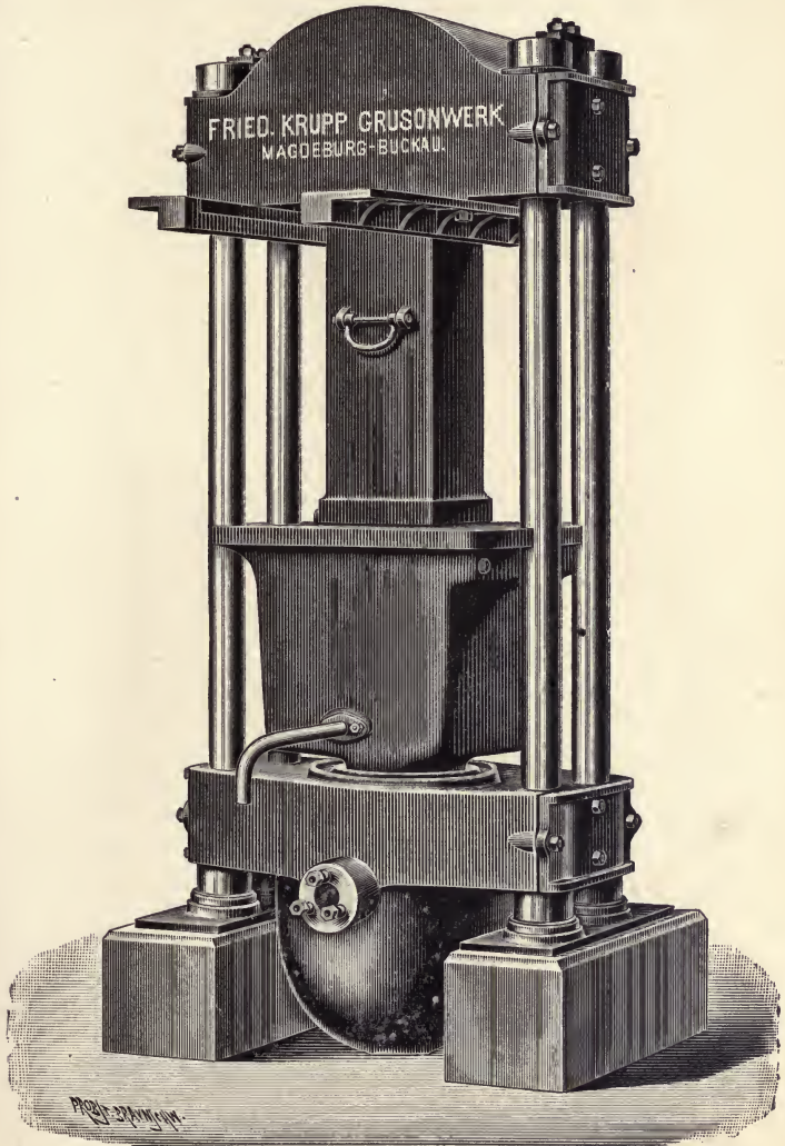
FIG. 37. Hydraulic Press for Round Cakes (Fr. Krupp).
