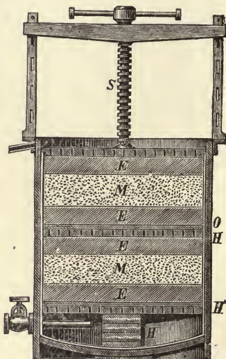
FIG. 92. Upward Filter.
