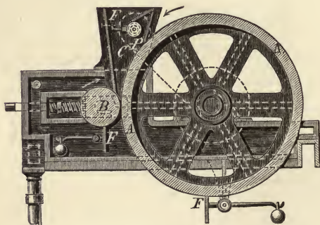
FIG. 20. Crushing Roller Mill (Section).
