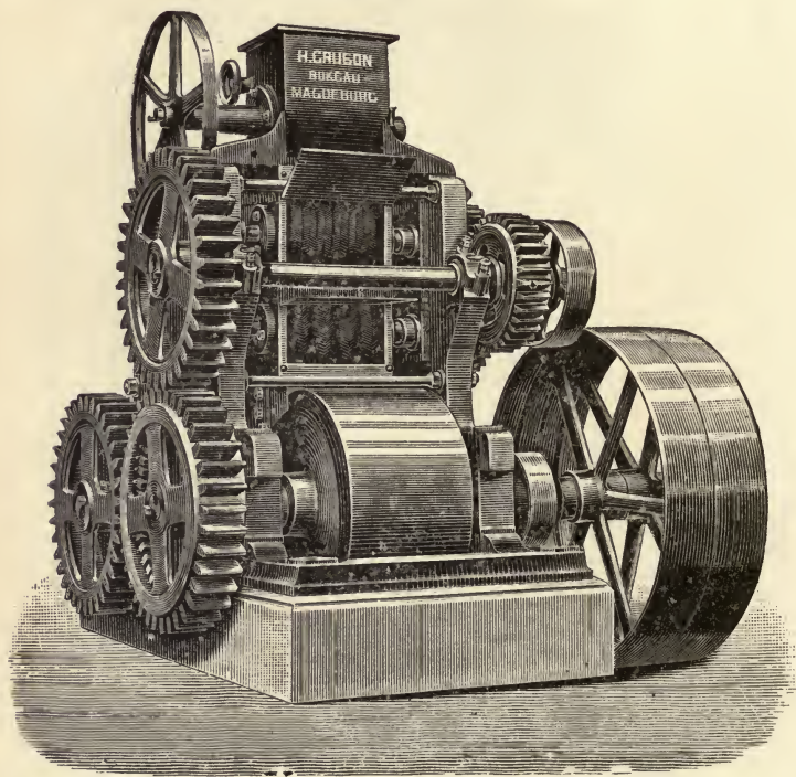
FIG. 22. Crushing Rollers for Palm Kernels and Ground Nuts (Fr. Krupp).
