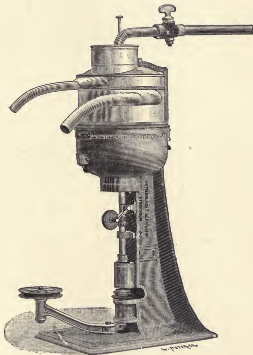
FIG. 80. Emulsifier with Centrifugal Pump (Elevation).
