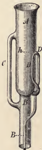
FIG. 1. Soxhlet Extractor.
