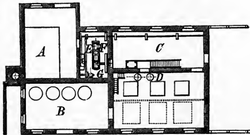
FIG. 63. Ground Plan of Works. A, Boiler House; B, Store and Refinery; C, Grinding Room, Elevator; D, Extraction House.
