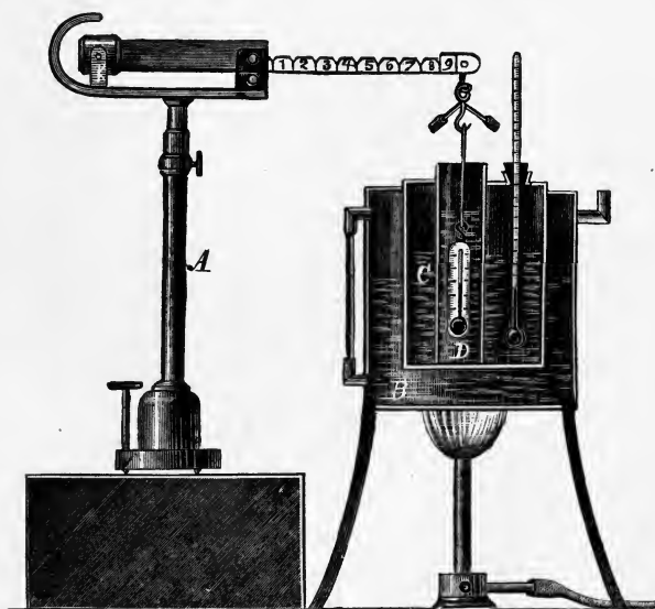
FIG. 94. Westphal Balance.
