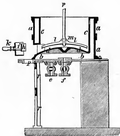
FIG. 25. Heating Pan for Oil Seed.
