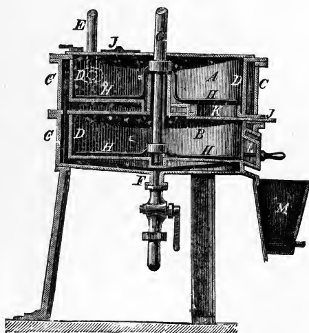
FIG. 26. Improved Heating Pan (Section).
