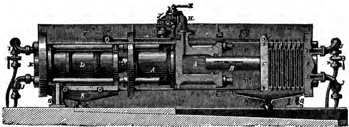
FIG. 44. Horizontal Four Cylinder Press.
