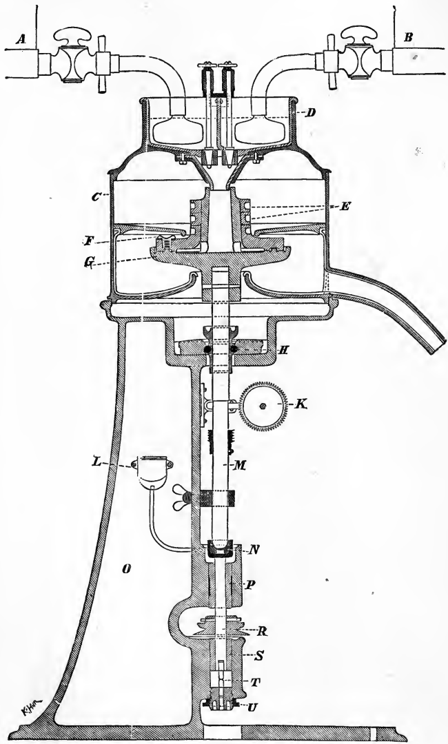
Fig. 81. Emulsifier (Section).
