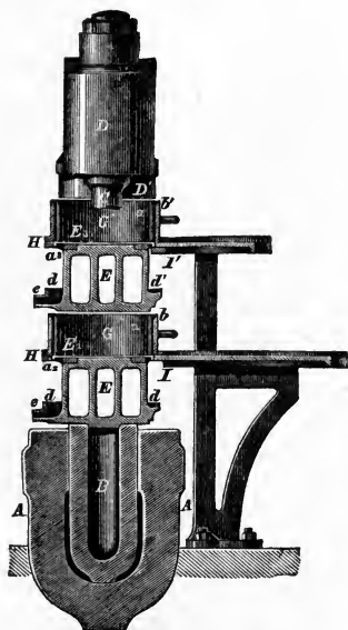
FIG. 32. Hydraulic Pan Press (Side View and Section).
