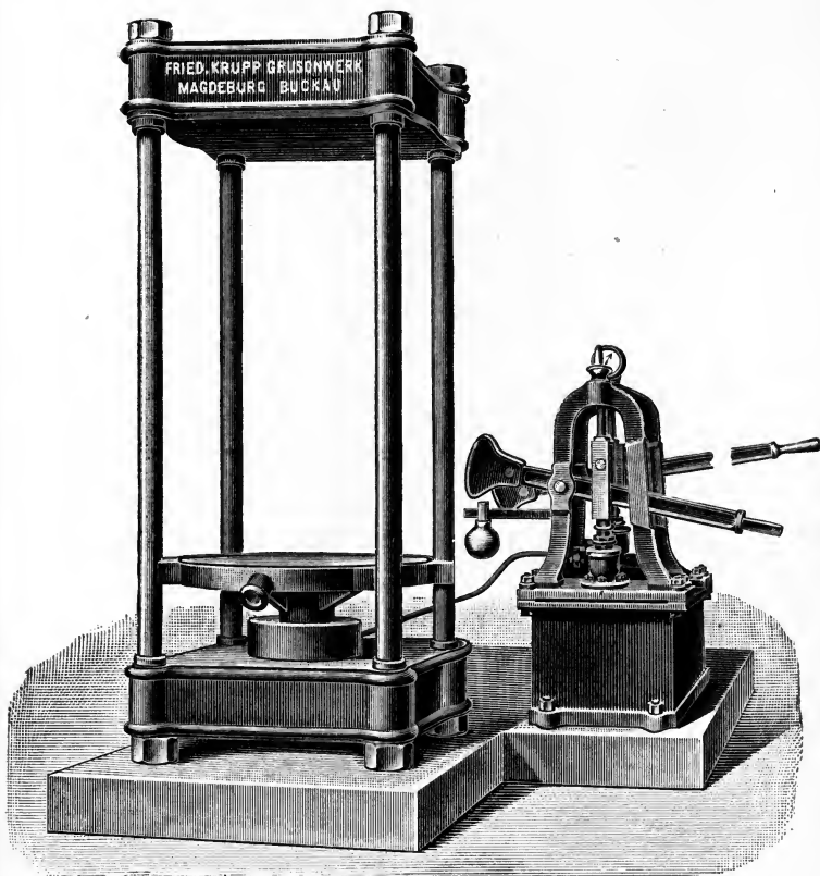
FIG. 39. Preliminary Press for Oil Fruits (Fr. Krupp).
