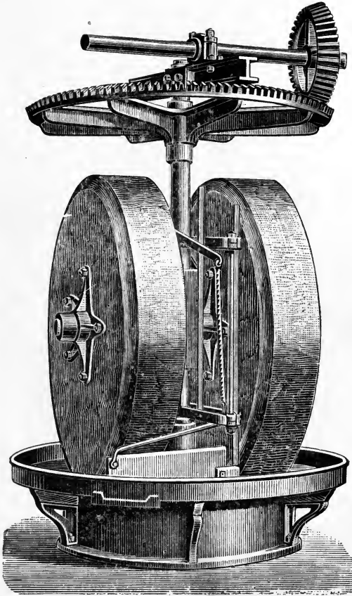
FIG. 17. Ordinary Edge-runner Seed Mill.
