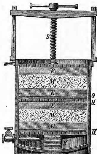
FIG. 92. Upward Filter.
