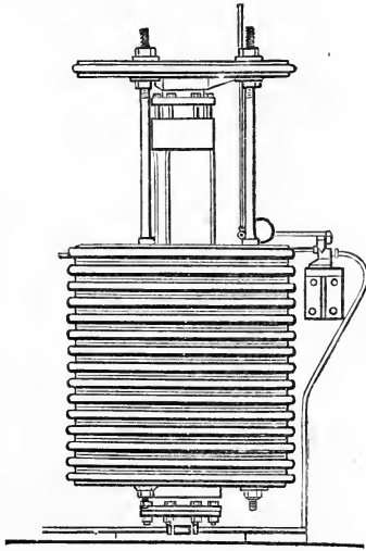
FIG. 33. Accumulator for supplying several Hydraulic Presses.
