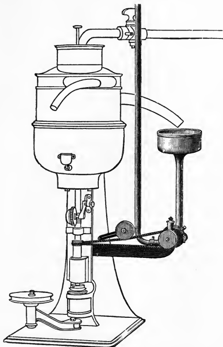
FIG. 79. Emulsifier with Centrifugal Pump (Section).
