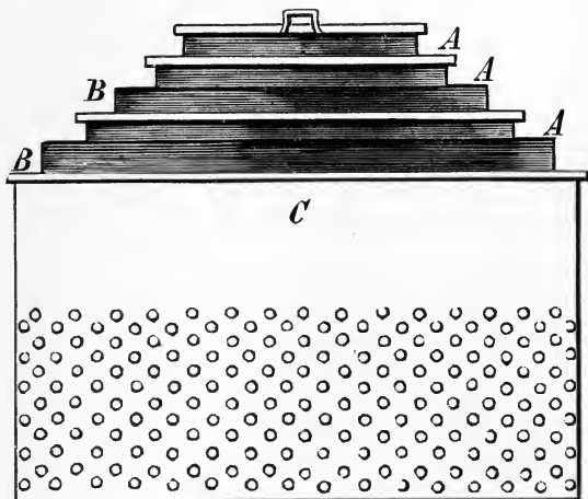
FIG. 87. Decantation and Filtering Apparatus. A, Decanting Boxes; B, Filters; C, Sifter; D, Slits in A; J, Supports (see Fig. 86).
