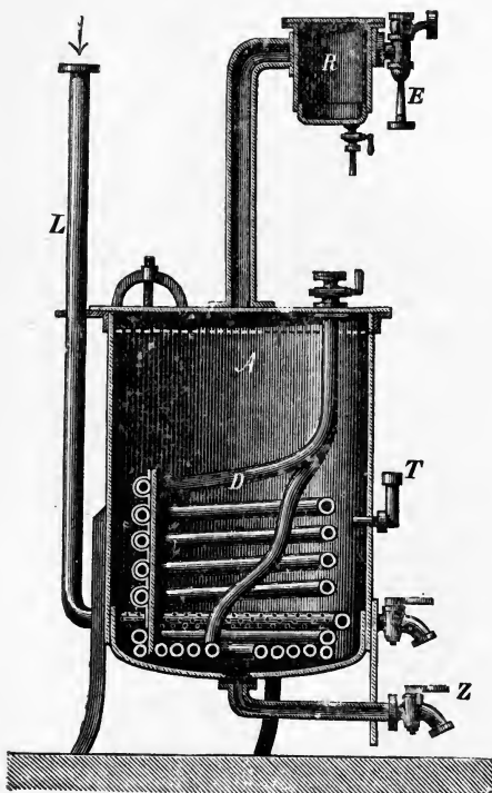
FIG. 85. Oil Refining Pan.
