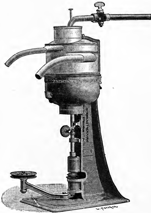
FIG. 80. Emulsifier with Centrifugal Pump (Elevation).
