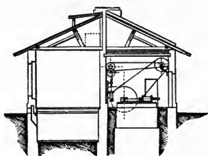
FIG. 64. Cross Section through Extraction House.
