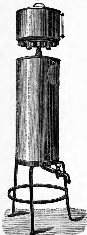
FIG. 88. Bag Filter.
