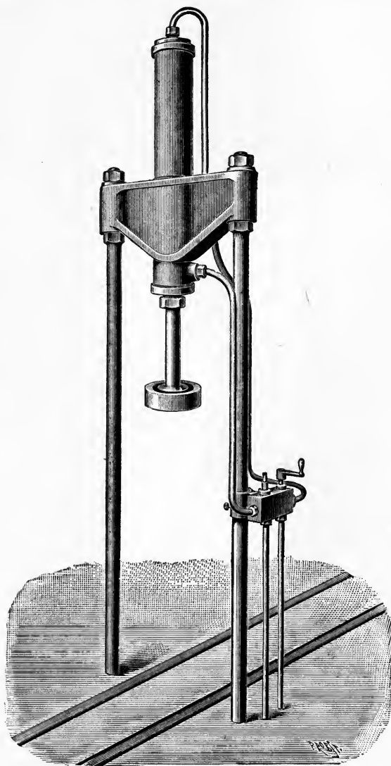
FIG. 38. Cake Discharger (Fr. Krupp).
