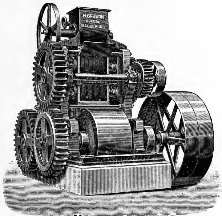
FIG. 22. Crushing Rollers for Palm Kernels and Ground Nuts (Fr. Krupp).
