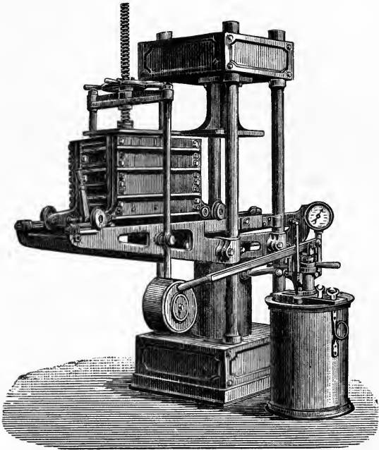
FIG. 45. Hydraulic Press with Movable Box.
