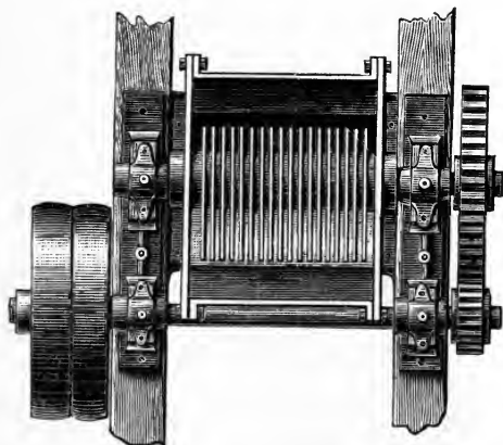
FIG. 14. Coconut Breaker (Viewed from above).
