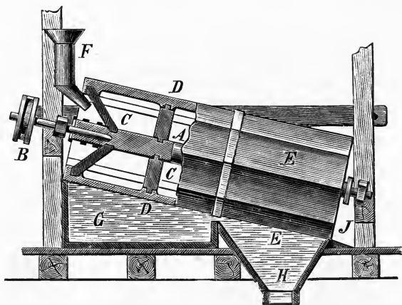
FIG. 9. Screening Cylinder (Elevation and Vertical Section).
