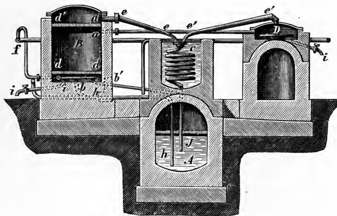
FIG. 55. Deiss's Extractor (Section).
