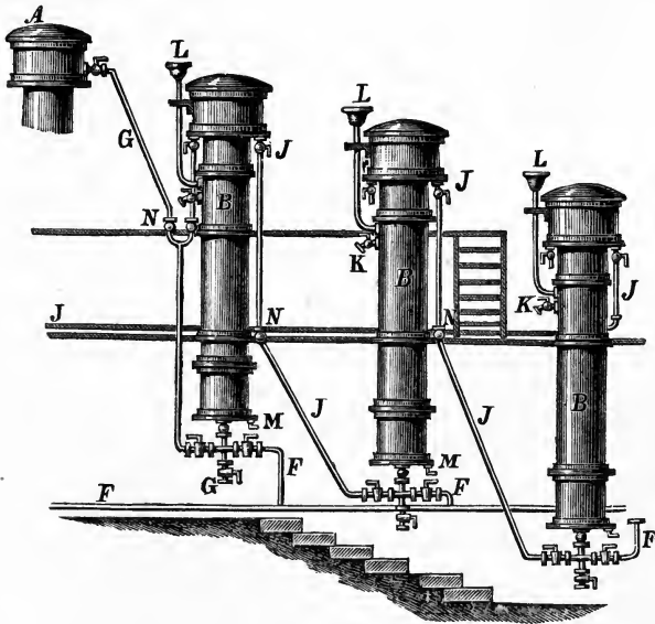
FIG. 90. Raymond-Combret Oil Purifying Apparatus.
