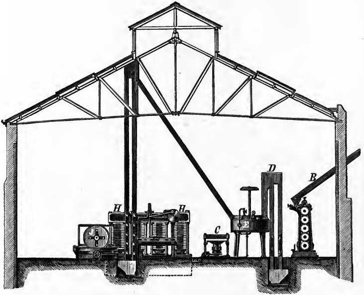
FIG. 48. Section of an Anglo-American Oil Mill.
