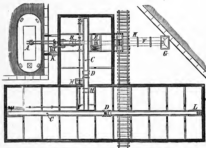
FIG. 6. Oil Seed Store (Rose, Downs & Co.).
