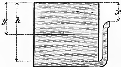
FIG. 78. Florentine Bottle.
