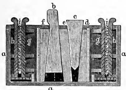
FIG. 30. Wedge Press.
