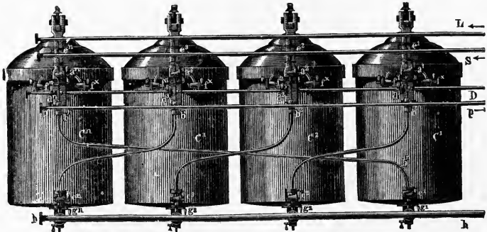
FIG. 57. Seiffert's Battery of Extractors.
