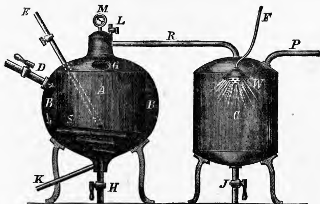
FIG. 58. Benzine Still.
