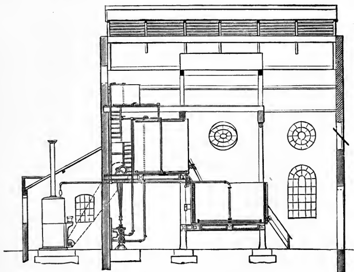
FIG. 70. Cotton-Seed Oil Refinery.
