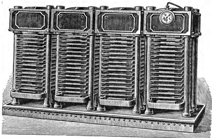
FIG. 47. Battery of Four Anglo-American Presses on Wrought-iron Case for the Reception of the Oil.
