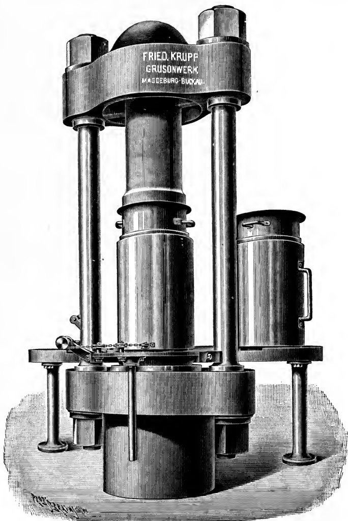
FIG. 36. Hydraulic Press for Coprah and Palm Kernels.
