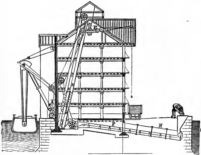
FIG. 7. Oil Seed Store (Rose, Downs & Co.).
