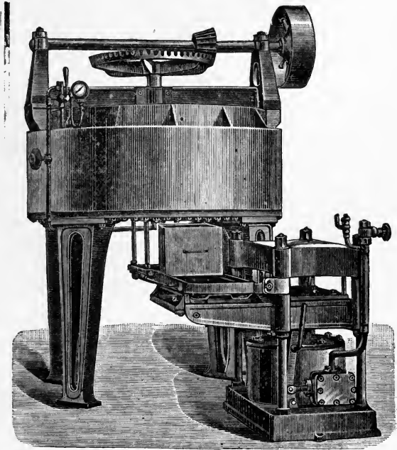
FIG. 28. Heating Pan with Steam Cake Mould.
