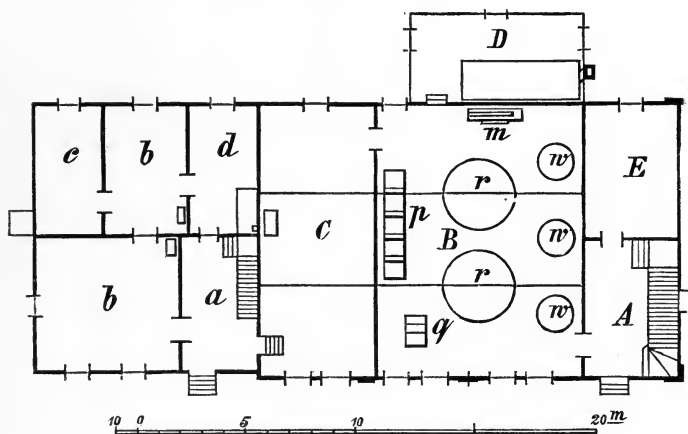
FIG. 53. Ground Plan of an Oil Factory Building (Knäbel).
