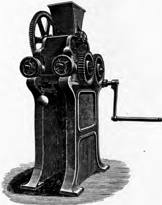
FIG. 13. Hand-power Decorticator for Castor-oil Seeds.
