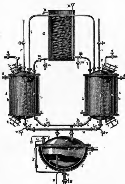
FIG. 56. Vohl's Extractor.
