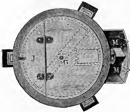
FIG. 27. Improved Heating Pan (Ground Plan).
