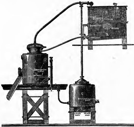
FIG. 60. Wegelin & Hübner's Extractor.
