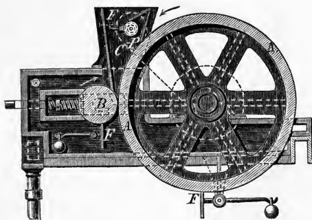
FIG. 20. Crushing Roller Mill (Section).
