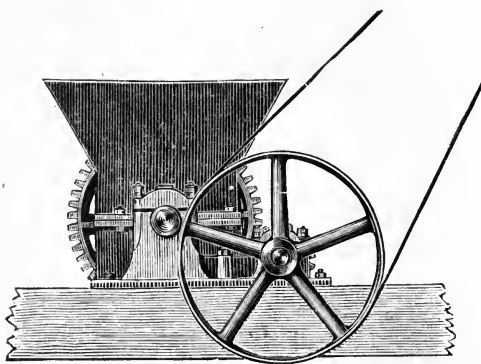
FIG. 15. Coconut Breaker (Front View).
