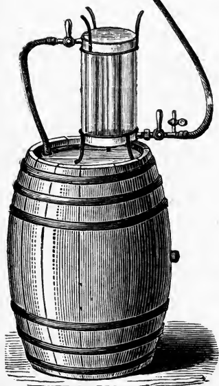
FIG. 91. Vollmar's Rapid Filter.
