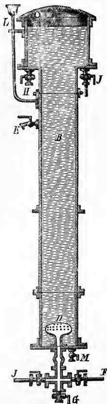
FIG. 89. Raymond-Combret Oil Purifier. Purifying Cylinder.
