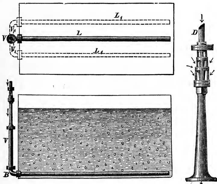
FIG. 83. Air Blast Agitator with Korting Injector.
