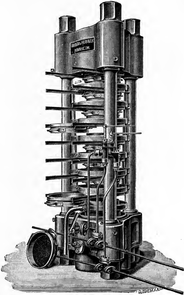
FIG. 42. Hydraulic Ring Press (Brinck & Hübner).
