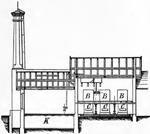
FIG. 62. Sectional View of Oil-Extracting Works.
