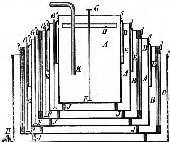
FIG. 86. Decantation and Filtering Apparatus for Palm Kernel Oil. E, Jacket Surrounding A; F, Effluent Valve; G, Valve Rods; H, Discharge Tap; K, Feed Pipe.
