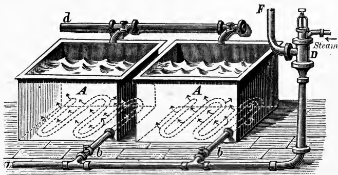
FIG. 84. Compressed Air Agitator.
