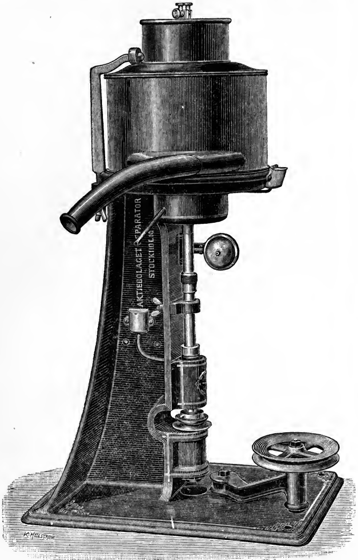
FIG. 82. Emulsifier (Elevation).
