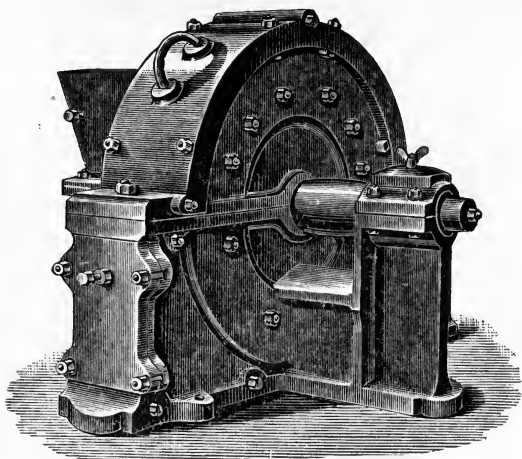
FIG. 16. Disintegrator for Coconuts.
