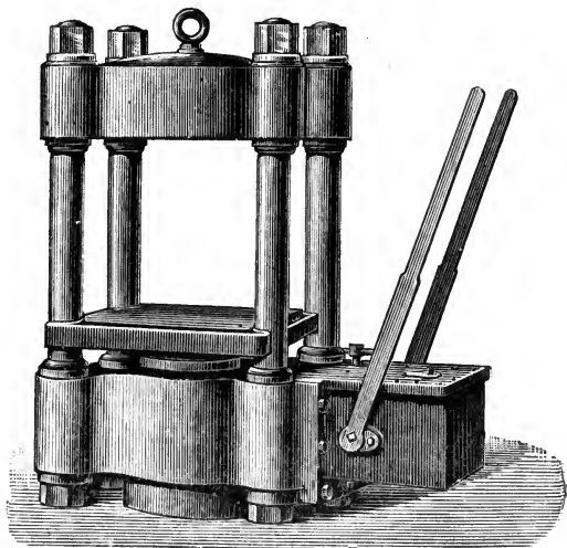
FIG. 46. Hydraulic Press for Oil Fruits.
