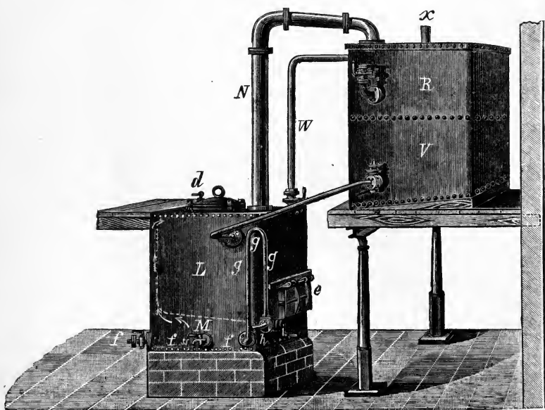
FIG. 59. Lindner & Merz's Universal Extractor.
