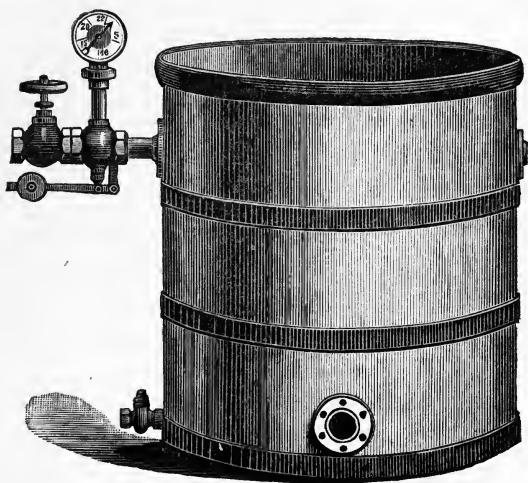
FIG. 75. Jacketed Refining Pan.
