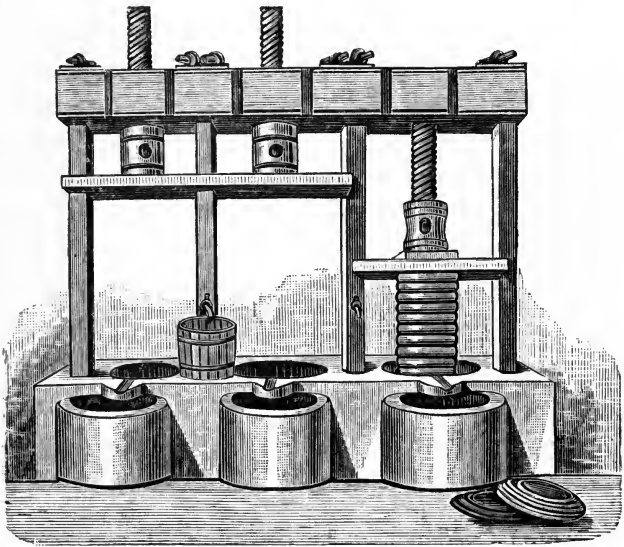
FIG. 72. Olive Oil Press from the Rizza District.
