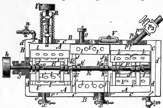
FIG. 93. John H. Filbert's Deodorising Apparatus.
