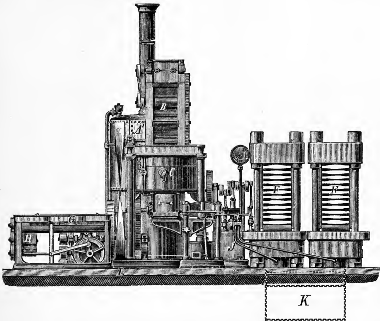
FIG. 51. Combined "Economic" Oil Mill.
