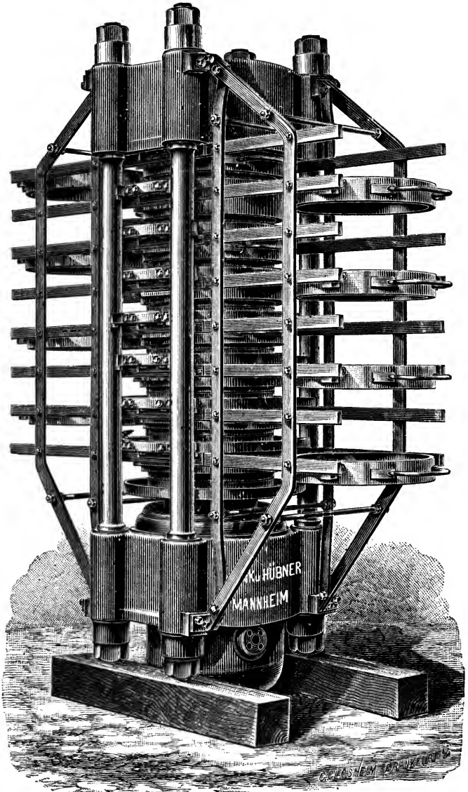
FIG. 41. Hydraulic Ring Press.
