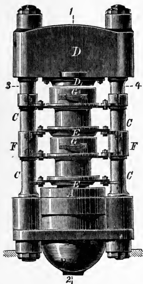
FIG. 31. Hydraulic Pan Press (Front View).
