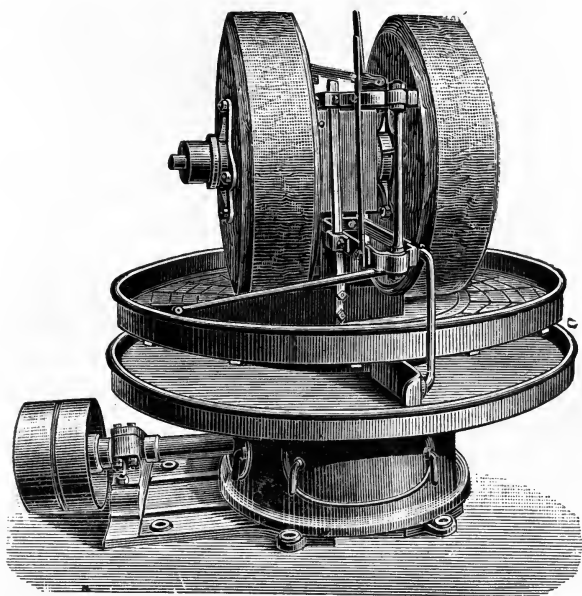
FIG. 18. Edge-runner Seed Mill (Anglo-American Pattern).
