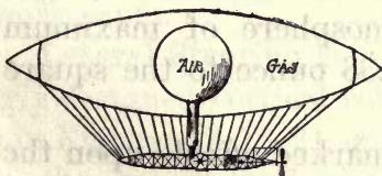
FIGURE 13.—Internal Balloon, used to keep envelope of dirigible taut without filling it so full of gas that some must escape in case of expansion. With this construction, expansion of the gas simply compresses the air bag, which is kept tightly inflated by the blower in the car.
