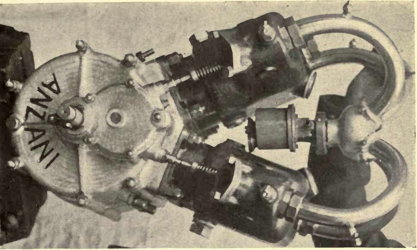
FIGURE 113.—Four-Cylinder—“Double-Twin”—Anzani Motor.
