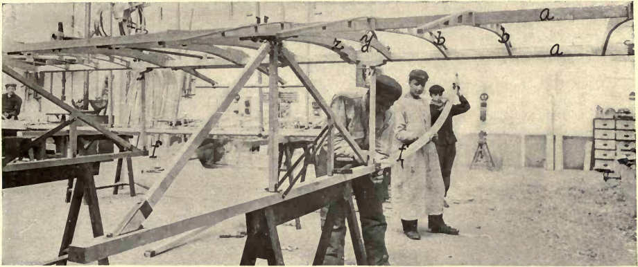
FIGURE 193.—The Wright Runner Construction. The solid ribs yz serve to support the motor, operator, etc. The other ribs bb are so built up as to enclose the wing bars aa between the double surfacing of fabric. The attachment of the forward curved members of the runners at f is clearly apparent upon close examination.
