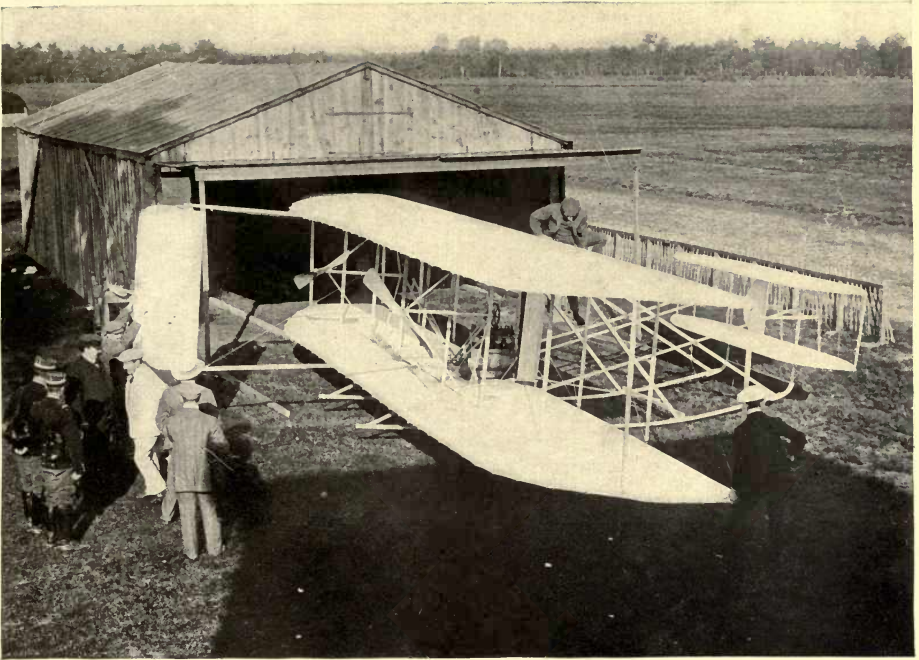
FIGURE 186.—Side View of Wright Machine.
