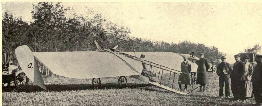
FIGURE 77.—Bleriot Monoplane VIII. The feature of this machine was the control of lateral balance by the pivoted ailerons aa .
