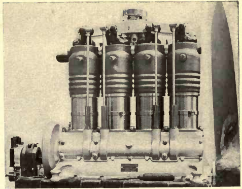
FIGURE 115.—Fiat and Panhard Aeronautical Motors. These are remarkable examples of refined construction, the Fiat developing 50 horsepower with a weight of only 110 pounds, and the Panhard weighing 176 pounds for 45 horsepower.
