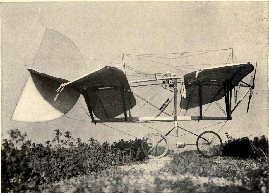
FIGURE 227.—Side View of Small, Power-Propelled Montgomery Double Monoplane. This machine has a wing spread of 26 feet, an area of 250 square feet, and weighs from 400 to 450 pounds, including the weight of the operator and the fuel. It flies at a speed of over 30 miles an hour with less than six horsepower, and employs more deeply cambered curves than have been successfully used in any other machine. Its stability is inherent in the form of its surfaces rather than dependent upon the manipulation of balancing devices, so that if dropped upside down it will invariably right itself and commence gliding with a fall of not over four or five times the span of its wings. The large vertical surface at the rear has no movement sidwise, being a stabilizing fin, not a rudder.
