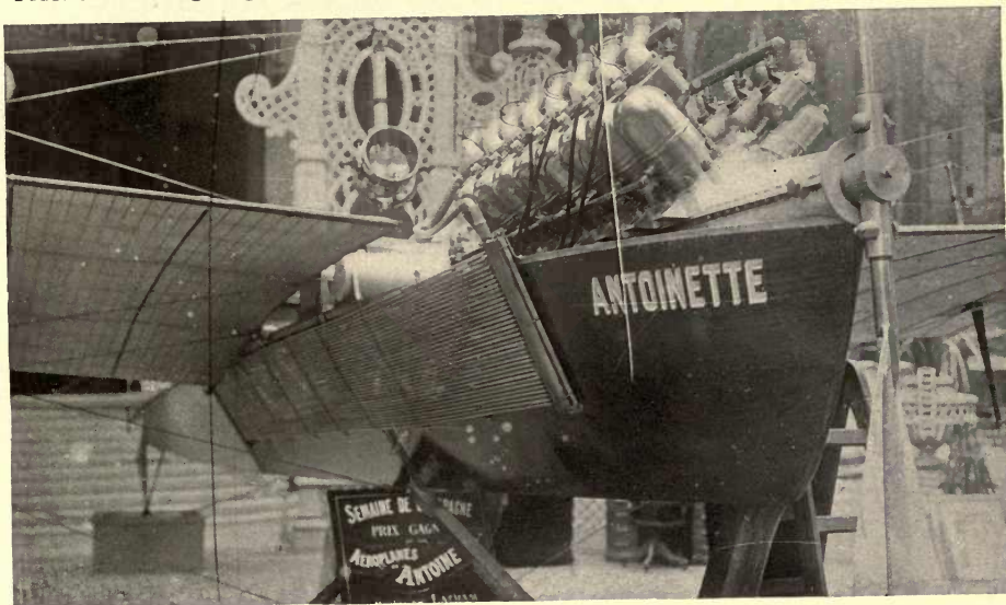
FIGURE 175.—Boat-like Body of Antoinette Monoplane. This machine, which is equipped with a hundred horsepower motor, will run on the land, in the water, and in the air.
