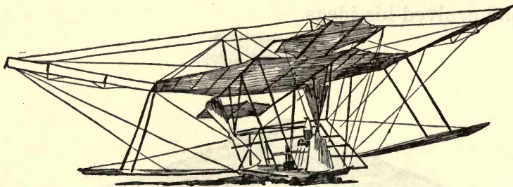
FIGURE 236.—Maxim Multiplane. When run on rails at Baldwin's Park, England, July 31, 1894, at 36 miles an hour, this machine lifted so much more than its weight that it broke a set of rails provided to hold it down and thus demolished itself.
