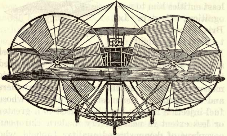
FIGURE 37.—Moy's Aerial Steamer. Tested on a track in the Crystal Palace, London, in June, 1875. Six-foot propellers. Steam engine, 2\frac{1}{4} \times 3 -inch cylinder, developing three horsepower at 550 revolutions a minute. Engine weighed 80 pounds, with boiler. Car ran on three small wheels. Speed of 12 miles an hour proved insufficient to lift.
