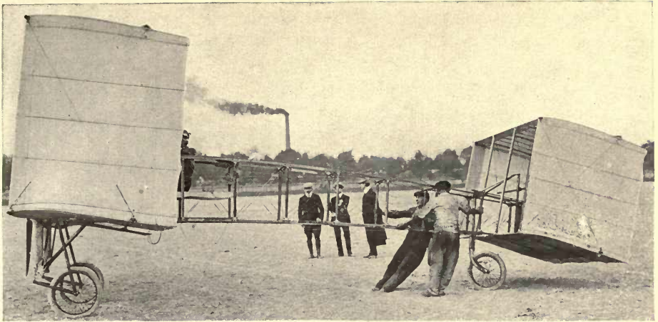
FIGURE 203.—Latest Model Voisin Biplane—With tractor screw and no front elevator.
