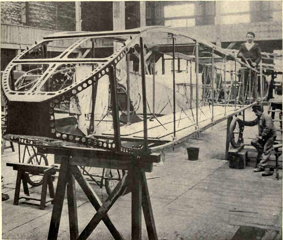
FIGURE 89.—Fuselage of Bolotov Monoplane. In the finished machine this frame is covered over with fabric while the boarded floor comes beneath the operator's seat, motor, etc.
