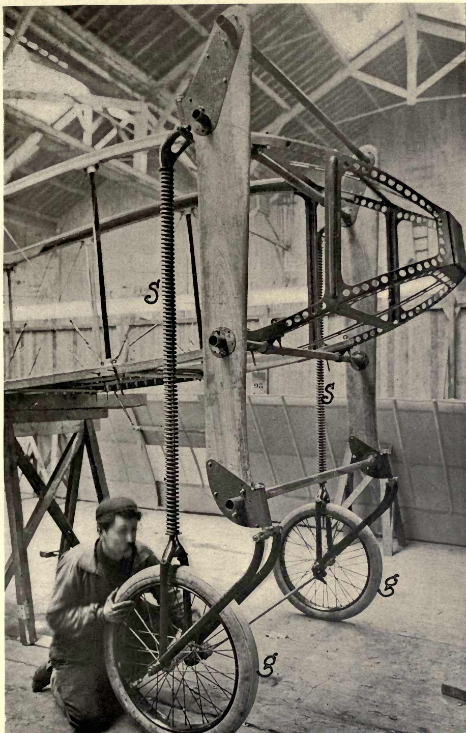
FIGURE 170.—Typical Alighting Gear. In this the upward swing of the wheels g g on their link connections is cushioned by the helical springs s s .
