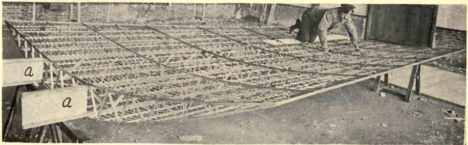
FIGURE 72.—Framing of Antoinette Wing Inverted. The load is supported on the two main girders aa , which are connected by a maze of crossbraces to the transverse ribs and secondary longitudinal members.
