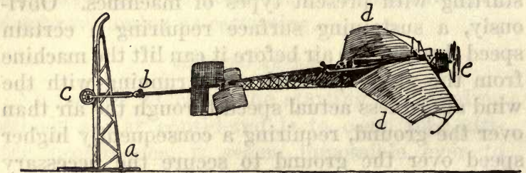
FIGURE 169.—Bleriot Starting Device. The aeroplane is hooked by the rope b to the pulley c , which runs along the rear edge of the pillar a . By starting the propeller the back draft of air thrown under the wings d d is expected to lift the machine until c runs off the top of a .
