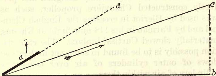
FIGURE 96. Angle of Propeller-Blade to Angle of Travel. With the blade moving in the direction of the large arrow, it is obvious that to produce a thrust in the direction of the small arrow the blade a must be inclined to the pitch, or line of travel.
