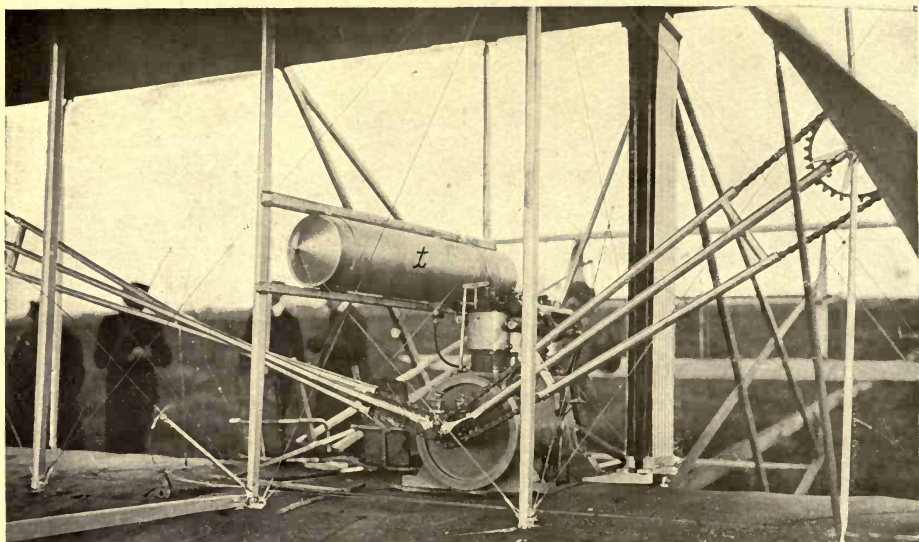
FIGURE 139.—Chain Transmission of Wright Biplane. Note the crossing of tubular chain-guides at the left—also the placing of the fuel tank t at the center of gravity.
