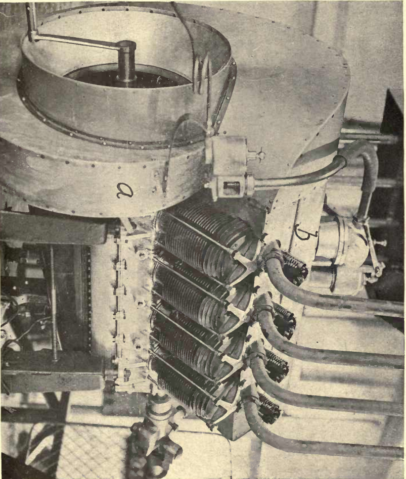
FIGURE 114.—Renault Eight-Cylinder V-Sharp ed Motor. Cooled by air forced through the pipe b by the blower a .
