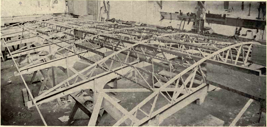
FIGURE 71.—Internal Framing of Antoinette Monoplane Wing.
