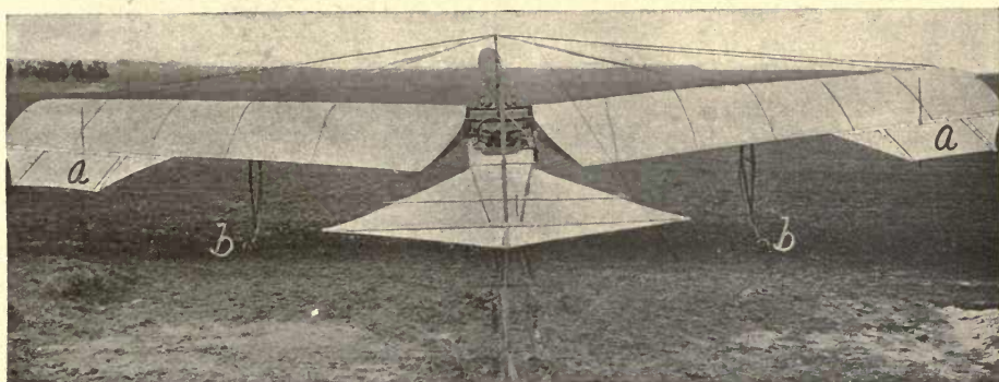
FIGURE 214.—Rear View of Antoinette V. In this view the ailerons a a and the balancing rollers b b are well shown.
