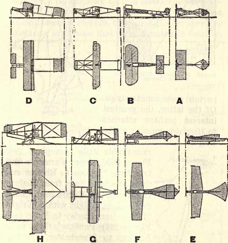
FIGURE 264.—Diagrammatic Comparisons of Modern Aeroplanes. A , Santos-Dumont Monoplane; B , Bleriot Monoplane; C , Curtiss Biplane; D , Voisin Biplane; E , R. E. P. Monoplane; F , Antoinette Monoplane; G , Wright Biplane; H , Cody Biplane.
