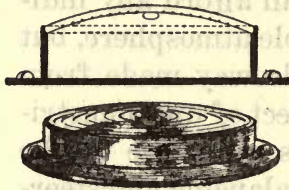
FIGURE 224. — Universal Level. This consists of a metal cup with a curved glass top, beneath which a bubble floats in a liquid. The direction of its movement from the center shows the direction of its tilting, while the amount of its movement over the graduated rings on the glass is a measure of the extent of the tilting.
