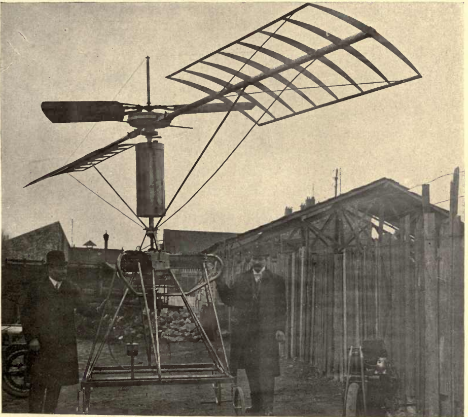
FIGURE 31.—Bertin Helicopter.
