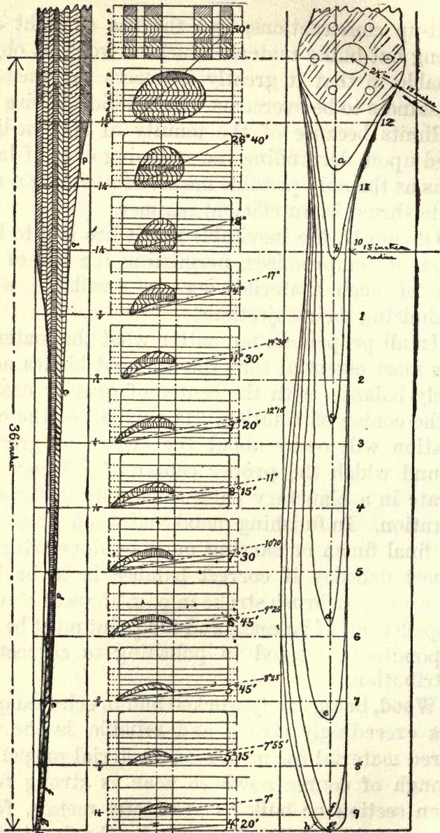
FIGURE 108.—Working Drawings of a Wooden Propeller.
