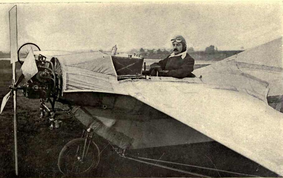
FIGURE 252.—Cockpit and General Details of R. E. P. Monoplane.
