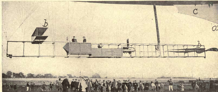
FIGURE 22.—Nacelle of the French Dirigible "Zodiac III."
