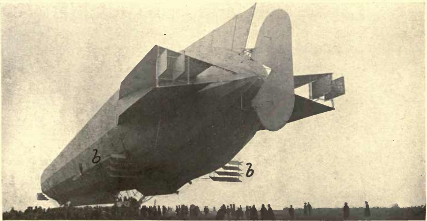
FIGURE 17.—The latest Zeppelin Dirigible. The upper picture shows the rigid construction very clearly, while in the different views the stabilizing fins c , the dipping planes bb , and the rear rudder a , are clearly shown.
