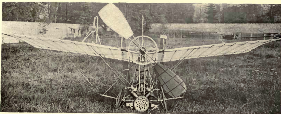
FIGURE 218.—Front View of Santos-Dumont's Belt-Driven Monoplane.
