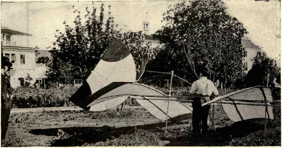
FIGURE 226.—Side View of Montgomery Double Monoplane Glider. This machine was probably built on more scientific principles than any other so far constructed. On at least three occasions operators have deliberately turned side somersaults with it, besides which many descents have been safely made from heights ranging up to 4,000 feet, at speeds said to have ranged as high as 68 miles an hour. Its equilibrium is so positive that it automatically rights itself when released upside down in the air.
