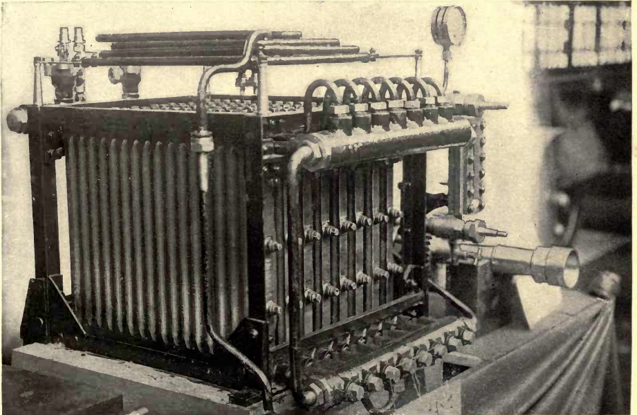
FIGURE 132.—Water-Tube Boiler for Aeronautical Use. This boiler closely resembles the steam "generators" used in steam automobiles. Its light weight, efficiency, capacity for the rapid production of steam at extremely high pressure, and its freedom from scaling and corrosion are the chief merits of this construction.
