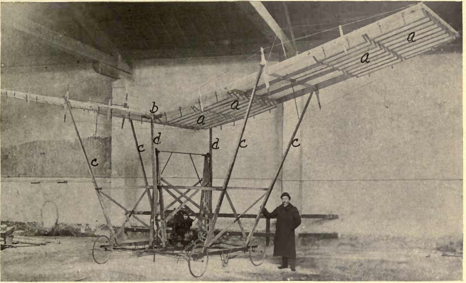
FIGURE 27.—Collomb Ornithopter. This machine is of the direct, orthogonal flapping-wing type, provided with valvular flaps at a a a a . The two wings, which pivot at the upper extremities of the links c c c c , are reciprocated by the vertical reciprocation of the arms d d .
