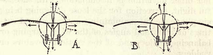
FIGURE 106.—Effect of Gyroscopic Action of a Single Propeller on Steering. With the directions of rotation shown, effort to steer in the direction of the solid arrows results in deviation in the direction of the dotted arrows, to an angular extent varying with the magnitude of the gyroscopic effect. This tendency can, of course, be allowed for by a practised operator. In both views the machine is to be regarded as approaching the observer.
