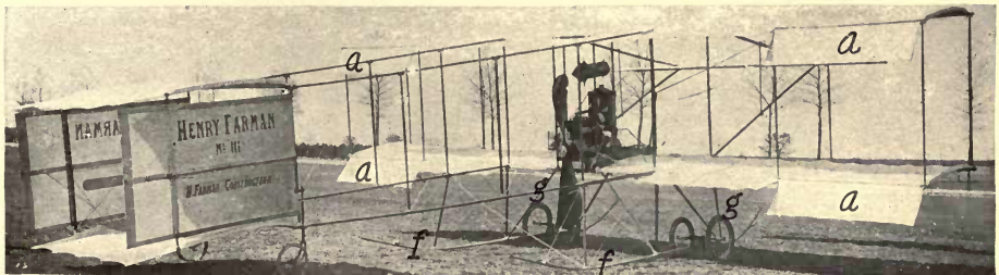
FIGURE 81.—Aileron Control of Farman Biplane. The four hinged ailerons are shown at aaaa .
