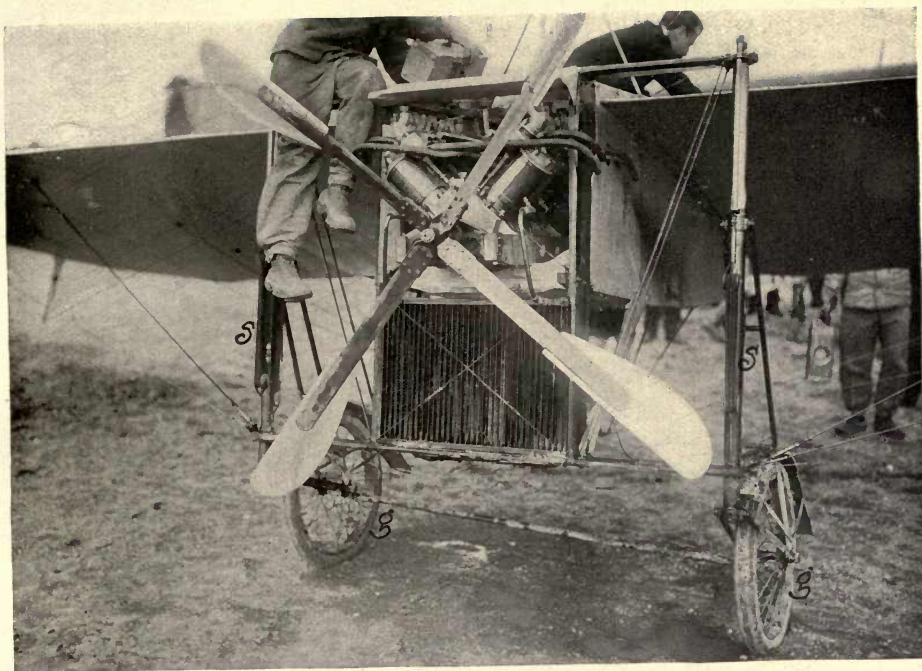
FIGURE 171.—Details of Bleriot Monoplane. This is one of the earlier machines of the “Bleriot XI” type, and is provided with an eight-cylinder, water-cooled motor, with radiator immediately beneath it. The wheels g g and the rubber springs s s are characteristic of the Bleriot alighting gear, but in the case of the latter the multiplication of the movement as shown in this view by passing over rollers has been abandoned.
