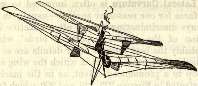
FIGURE 70.—Langley's 25-Pound Double Monoplane, With Wings at Dihedral Angle. This model on May 6, 1896, flew for more than half a mile over the Potomac River, at a speed of about 20 miles an hour. Subsequently, on November 28, 1906, with a similar model weighing about 30 pounds, a three-quarter mile flight at about 30 miles an hour was achieved. This was at the end of a three years' period of experimenting that had for its object the ultimate production of a man-carrying machine. The size of the heavier model was a little over 12 feet from tip to tip, with a length of about 16 feet. The whole power plant, which consisted of a 5-pound boiler and a 26-ounce non-condensing steam engine that developed 1\frac{1}{2} horsepower, weighed about 7 pounds. Propulsion was by bevel-gear driven, two-bladed twin screws, rotating in opposite directions behind the forward surfaces at about 1,200 revolutions a minute. The hull was metal sheathed to protect the burner from the wind, and the vessel between the forward surfaces was a float to keep the machine up when it alighted upon the water. In conjunction with the experiments with a man-carrying machine, which terminated with the unsuccessful launching on December 8, 1903, a model similar to the above, but weighing 58 pounds and having 66 square feet of sustaining surface—it being a one-fourth size copy of the large machine—was successfully flown with its 3-horsepower motor.
