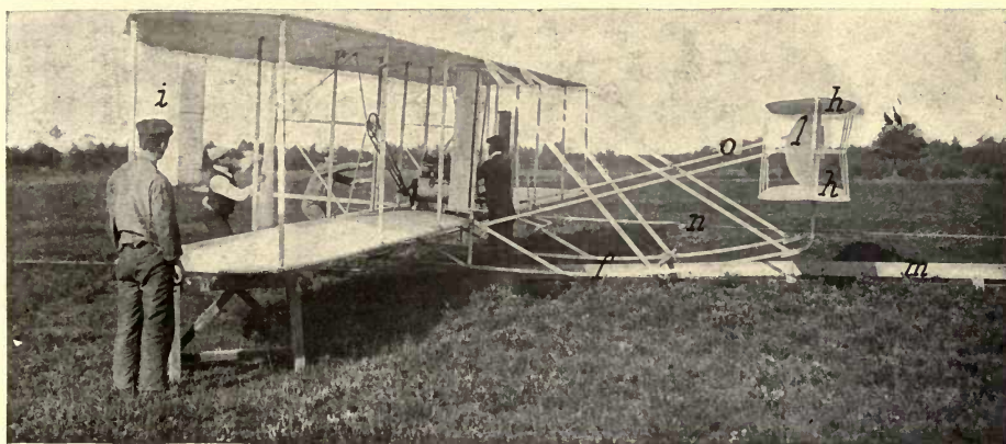
FIGURE 163.—Wright Machine on Starting Rail. The starting rail is at m , n is the connection of the rope by which the starting impulse is given, f are the runners, h is the elevator, o is the elevator control rod, i is the rudder, and l is one of the steadying planes peculiar to this machine.
