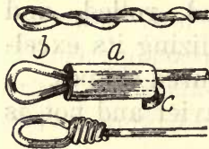
FIGURE 181. — Methods of Fastening Wire Ends. If the loop is made like the upper view, it will either come loose or draw into the shape that is shown in the lower view, which therefore is a proper form to use at the beginning. Another common method is to use the flattened piece of steel tubing shown at a in the middle view, the wire being simply bent as at b and c , which will hold it securely.
