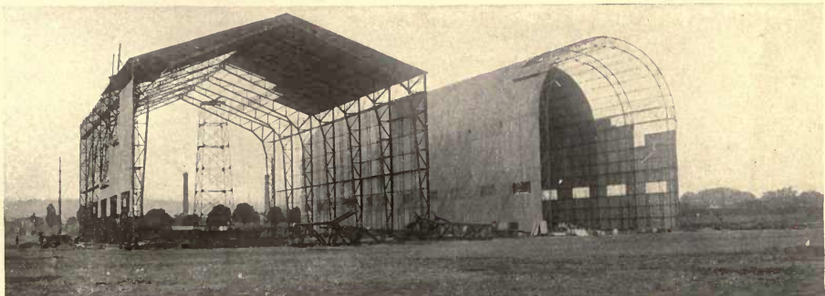
FIGURE 16.—Balloon Houses Nearing Completion.
