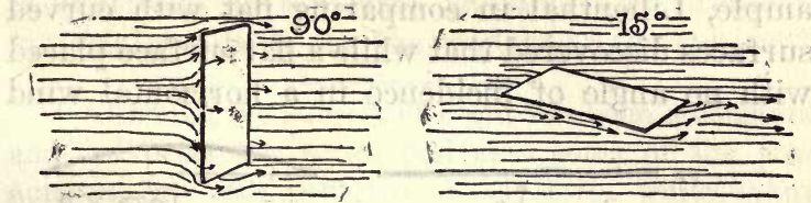
FIGURE 42.—Pressure on Vertical and Inclined Surfaces. In an air current of 25 miles an hour the surface at 90^\circ receives a pressure of 3.24 pounds to the square foot, while the surface inclined 15^\circ from the direction of the current receives a pressure of only .33 pounds, and at the same time affords an upward lift of 1.5 pounds.
