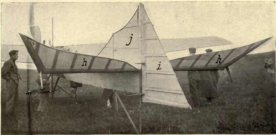
FIGURE 85.—Rear Controls of Antoinette Monoplane. In this hh are horizontally-pivoted surfaces for steering up or down; l is a vertically pivoted surface for steering sidewise; and j is a vertical fin used for its stabilizing effect.
