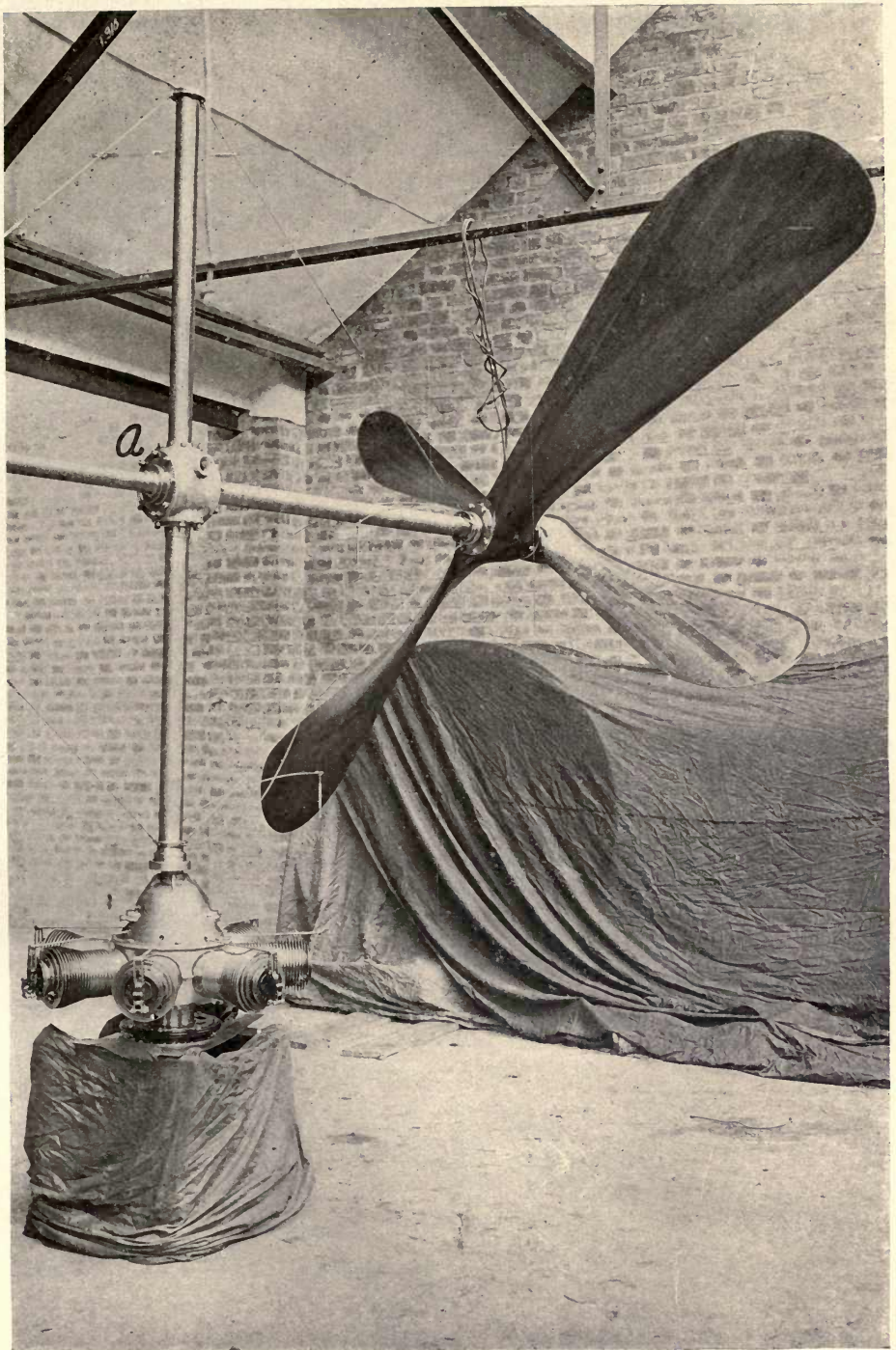
FIGURE 107.—Twin Wooden Propellers on Single Shaft, for the propulsion of a dirigible balloon. These propellers are driven by a Gnome engine mounted to revolve in a horizontal plane. The power is transmitted to the propeller shafts through bevel gears in the housing a .
