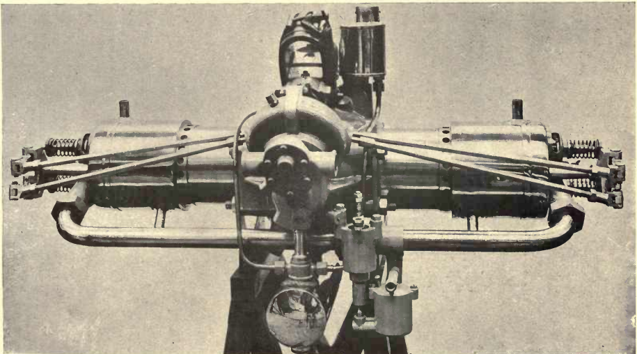
FIGURE 116.—Darracq and Dutheil-Chalmers Aeronautical Motors. The Darracq—in the lower view—is the engine with which Santos-Dumont achieved his recent successful monoplane flights. It weighs 66 pounds and develops 35 horsepower. Of particular interest in the other motor is the flywheel a , with steel rim and wire spokes.
