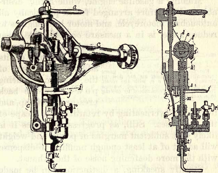
FIGURE 127.—Mietz and Weiss Fuel Pump. The gasoline comes from the tank through the pipe v , attached by the coupling u , and enters the cavity in the pump block s through the valve t . Its flow is caused by the plunger l , driven by the eccentric d through the strap g , and retracted by the spring m , and it passes out through the valve q and the pipe p to the engine cylinder. The stroke of l is regulated by the regulator handle a , mounted on the regulating shaft b , which forces down the plunger-guide sleeve i and thus retracts l from the eccentric. Priming is effected by pushing down on the pump handle j , which is forced up after each stroke by the spring k . At r is an air cock, to clear the system of possible air locks. A governor weight f on the shaft e is used to control the speed automatically, the whole running in the frame c .
