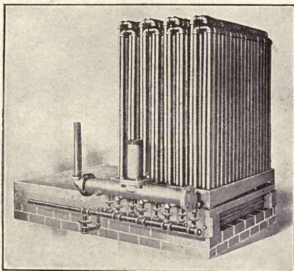
Fig. 67—Mounting and Connecting Pipe Heater
