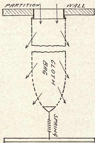
Fig. 70—Bag Filter
