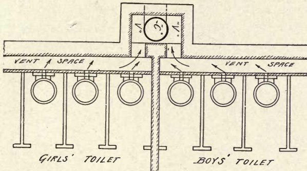
Fig. 111—Obtaining Draft Without Fans
