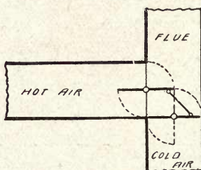
Fig. 38—A Double Mixing Damper
