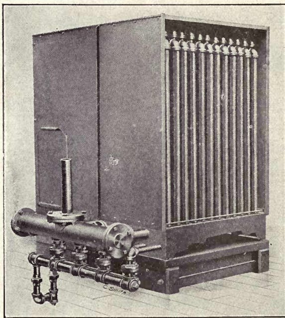
Fig. 68—Steel Plate Casing for Pipe Heater
