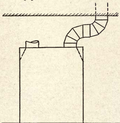
Fig. 133—Furnace Casing Connection
