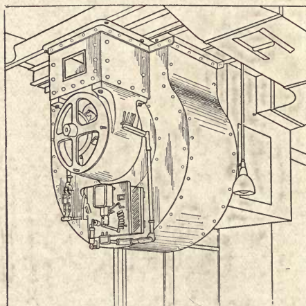
Fig. 140—Exhaust Fan and Motor Suspended from Overhead Construction
