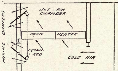
SECTIONAL VIEW.
