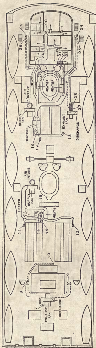
Fig. 146—Boat Deck (Mid-Ship)
