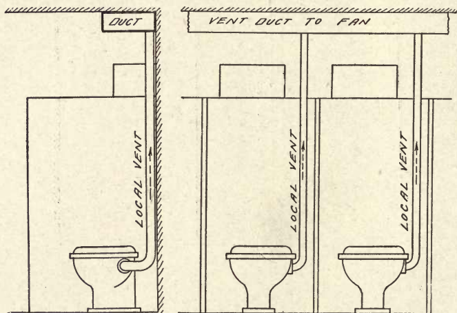
Fig. 104—Connecting Exhaust Duct with Local Vent
