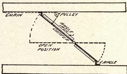
Fig. 47—Simple Form of Single Damper
