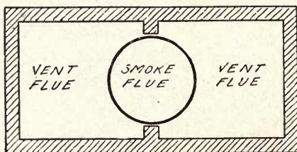
Fig. 25—Heating Two Vents in Schoolhouse
