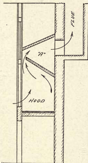
Fig. 114—Hood for Removal of Chemical Fumes
