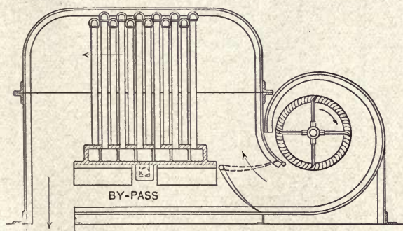
Fig. 139—Heater with Air- and Water-Tight Casing
