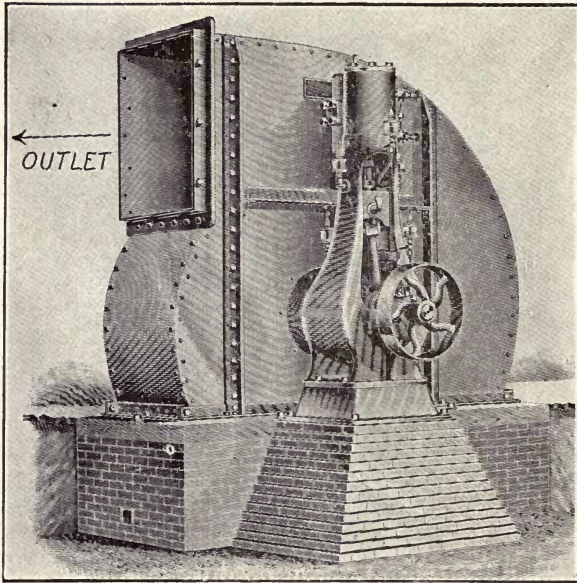
Fig. 52—Casing and Drive of Centrifugal Fan
