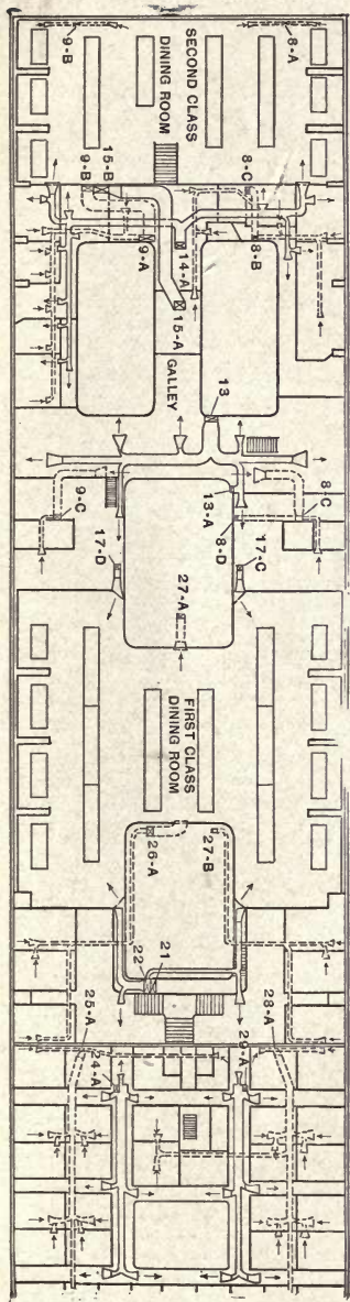
Fig. 149—Main Deck (Mid-Ship)
