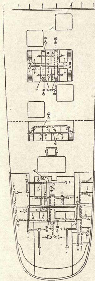
Fig. 143—Upper Deck (Stern)
