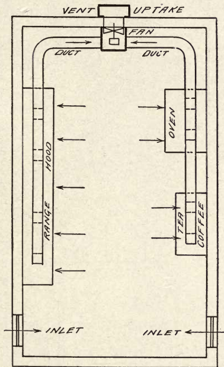
Fig. 81—Disk Fan Placed at Bottom of Flue
