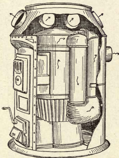
Fig. 116—Indirect Draft Furnace
