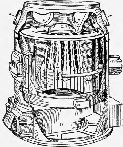
Fig. 117—Furnace with Large Amount of Heating Surface
