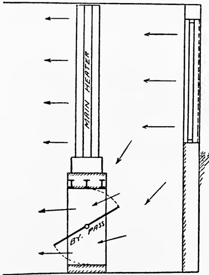
Fig. 44—A By-Pass Damper for Use in Fan Work
