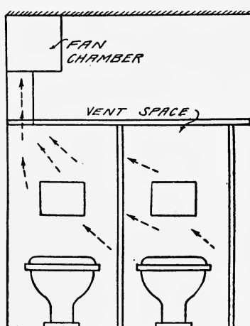
Fig. 106—Closed Ventilation Chamber of Slabs. Fig. 107—Set of Fixtures to Allow for Closed Ventilation Chamber
