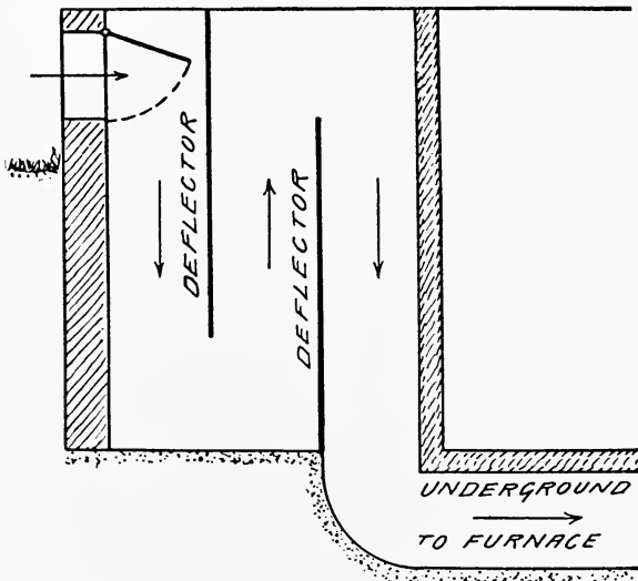
Fig. 8—Another Form of Mixing Chamber
