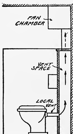
Fig. 106—Closed Ventilation Chamber of Slabs. Fig. 107—Set of Fixtures to Allow for Closed Ventilation Chamber
