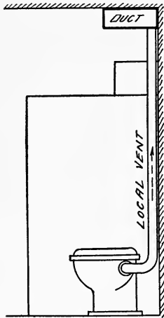
Fig. 104—Connecting Exhaust Duct with Local Vent
