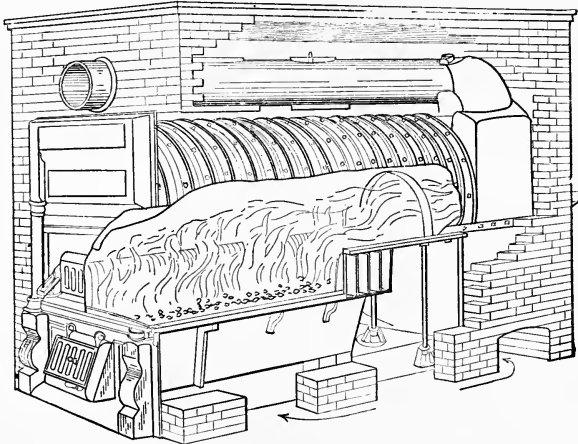
Fig. 131—Furnace and Casing
