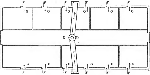
KING'S SYSTEM OF VENTILATION.
