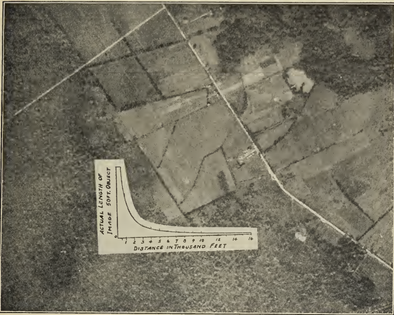
Fig. 100. — Illustrating the study of pattern for airplanes. The photograph was taken from an altitude of 10,000 feet. The insert shows the relative lengths (verticle scale) of an airplane of 50-foot spread at various distances below the observer.
