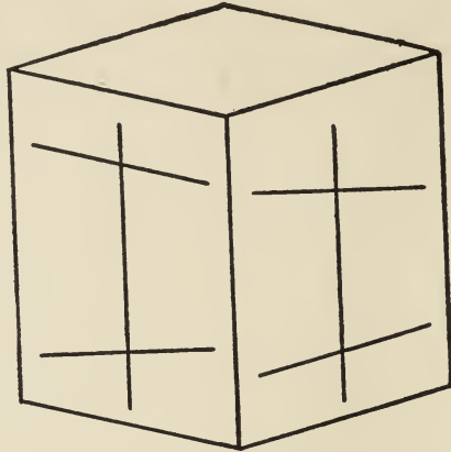
Fig. 21. — Owing to perspective the right angles appear oblique and vice versa.
