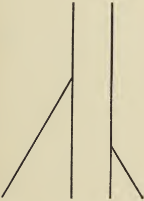
Fig. 45. — The two diagonals would meet on the left vertical line.
