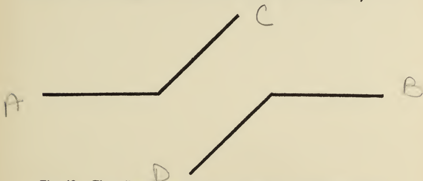
Fig. 42. The effect of two angles in tilting the horizontal lines.
