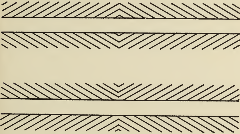
Fig. 38. — Parallel lines which do not appear so.
