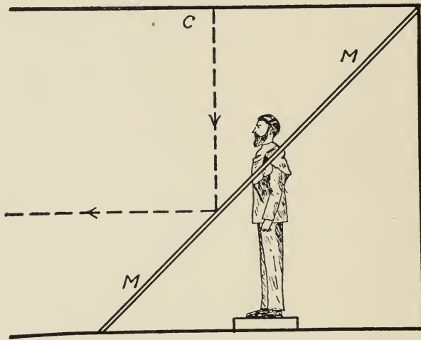
Fig. 91. — Another example of "mirror magic."
