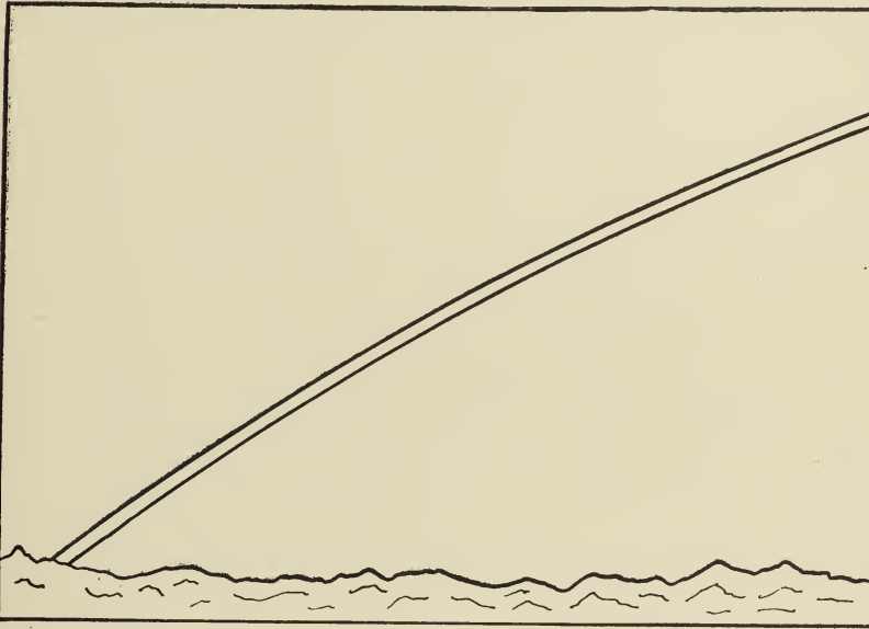
Fig. 78. — An accurate tracing from a photograph (continual exposure) of the moon rising.
