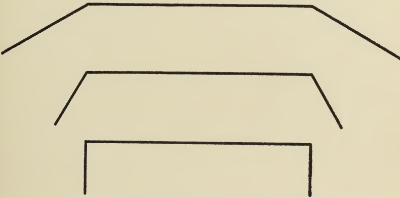
Fig.53. — Angles affect the apparent length of lines.
