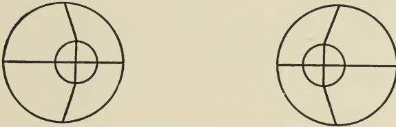
Fig. 2. — Stereoscopic pictures for combining by converging or diverging the optical axes.
