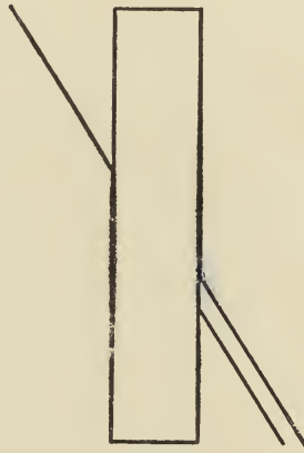
Fig. 46. — Poggendorff's illusion. Which oblique line on the right is the prolongation of the oblique line on the left?
