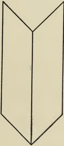
Fig. 31. — The reversible "open book" (after Mach).
