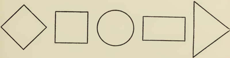
Fig. 60. — Five equal areas showing the influence of angles and contrasting lengths.
