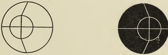
Fig. 69. — By combining these stereoscopically the effect of metallic lustre (similar to graphite in this case) is obtained.
