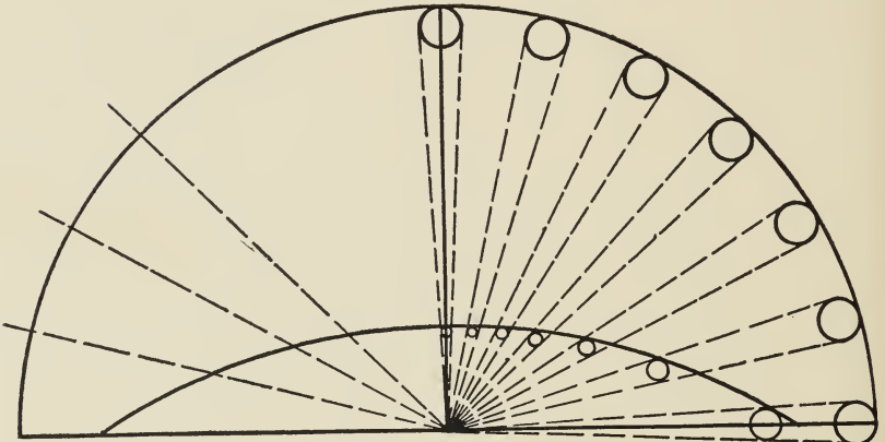
Fig. 80. — Explanation offered by Smith of the apparent enlargement of heavenly bodies near the horizon.
