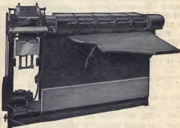
FIG. 7. — Machine for Sorting Cards.
