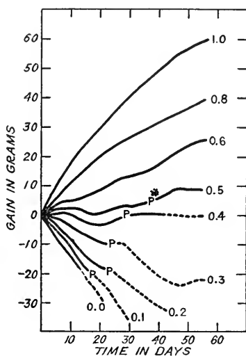
FIG. 5.—Average gain curves of rats on vitamin B-free diet (No. 513) plus daily supplements of ground whole wheat of 0.1, 0.2, 0.3, 0.4, 0.5, 0.6, 0.8, and 1.0 grams. Negative controls (marked 0.0) received basal diet only.
