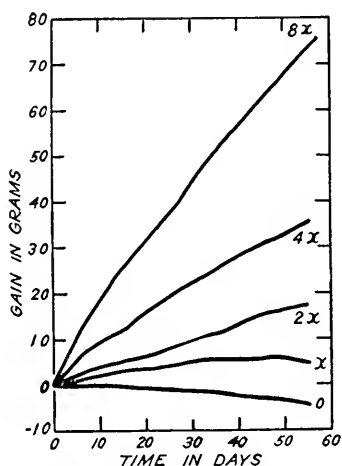
FIG. 6.—Average growth curves of rats receiving different amounts of vitamin G. The lowest curve shows the gradual loss of weight on the Bourquin basal diet alone; the others, the effects of feeding x amount per day of vitamin G in the form of milk, and 2, 4, and 8 times this amount. (Courtesy of Dr. Anne Bourquin.)
