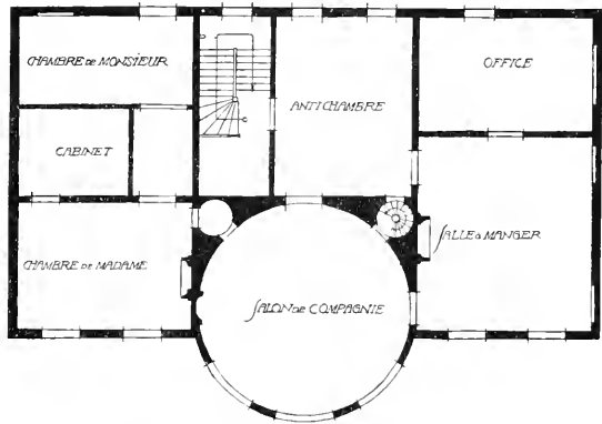
Abb. 203 Kleines Hotel in Paris Grundriß
