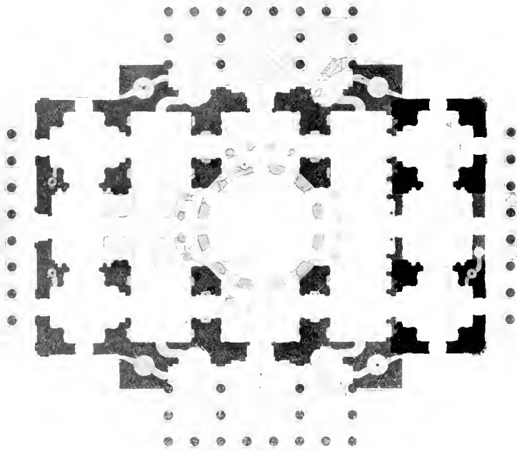
Abb. 19 Isaakskirche in Petersburg, Grundriß
