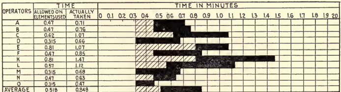
FIG. 23.—Comparison of Methods and Time on Pressing Shoulders.
