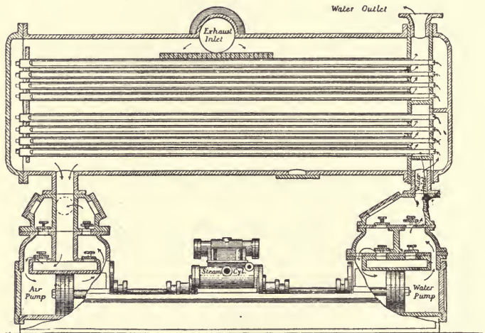
FIG. 36. WHEELER CONDENSER.
