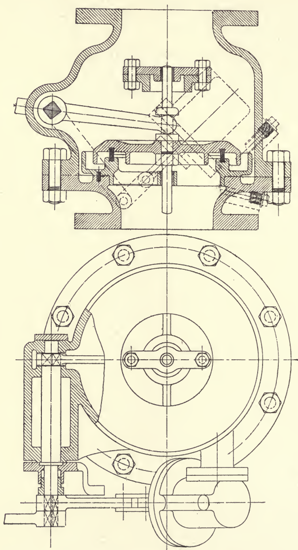
FIG. 45. ATMOSPHERIC VALVE.
