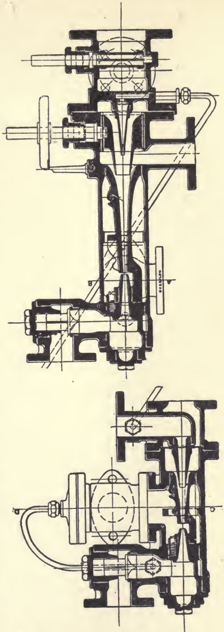
FIG. 90. COMBINED INJECTOR.
