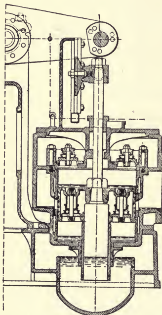
FIG. 55. VERTICAL AIR PUMP (Davey Paxman & Co.)
