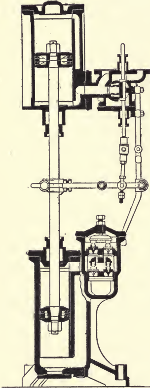
FIG. 86. WEIR FEED PUMP.
