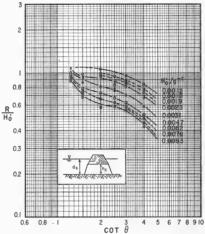
Figure E-3. Quarystone rubble-mound runup; d_s/H_0 = 8.0 ; H_0/k_p = 1.7 ; h_c/d_s \approx 0.75 (after Stoa, 1978a)
