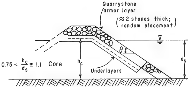
Figure F-1. Sketch of high-core rubble-mound structure.
