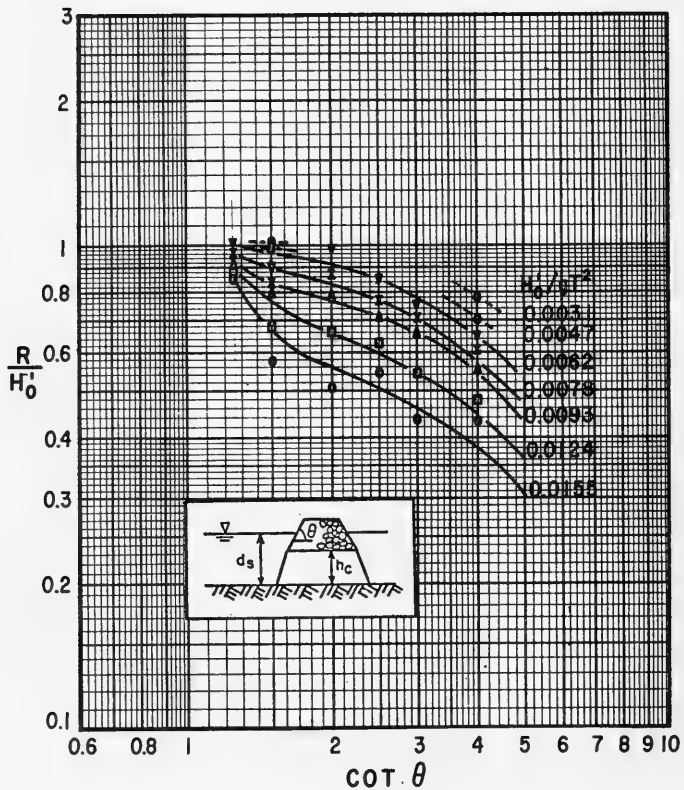
Figure E-1. Quarystone rubble-mound runup; d_s/H_0^1 = 3.0 ; H_0^1/k_r = 4.5 ; h_c/d_s \approx 0.75 (after Stoa, 1978a).
