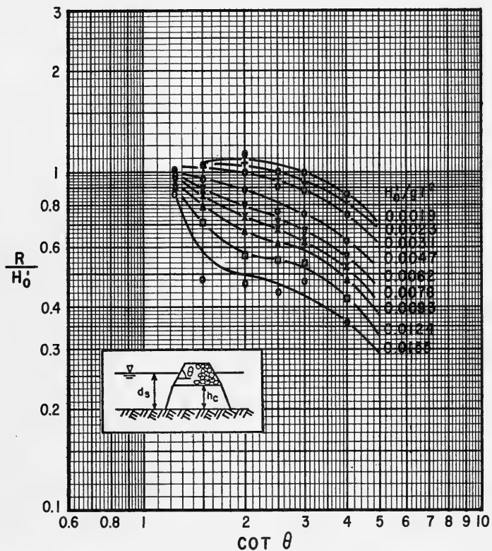
Figure E-2. Quarrystone rubble-mound runup; d_s/H_0 = 5.0 ; H_0/k_p = 2.7 ; h_c/d_s \approx 0.75 (after Stoa, 1978a).
