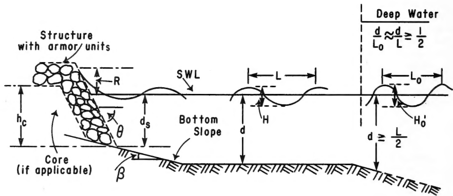
Figure 1. Definition sketch of variables applicable to wave runup.
