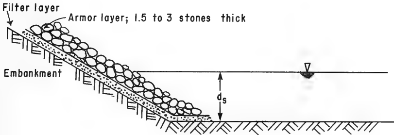
Figure A-1. Sketch of quarrystone embankment (riprap).
