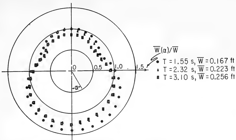
Figure 22. [\overline{W}(\alpha)/\overline{W}] patterns at 3-inch circular pile with identical incident wave height at three periods. Test conditions: \overline{H} = 0.34 foot, d = 1.00 foot, G = 25 feet.
