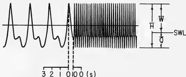
Figure 5. Water level record and measured wave dimensions: Wave height, H , crest height, W , and trough depth, Q .
