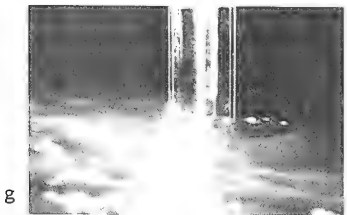
Figure 15. Photo sequence of wave crest incident into channel of 5x1 H-pile, with one-sixteenth second between successive frames.
