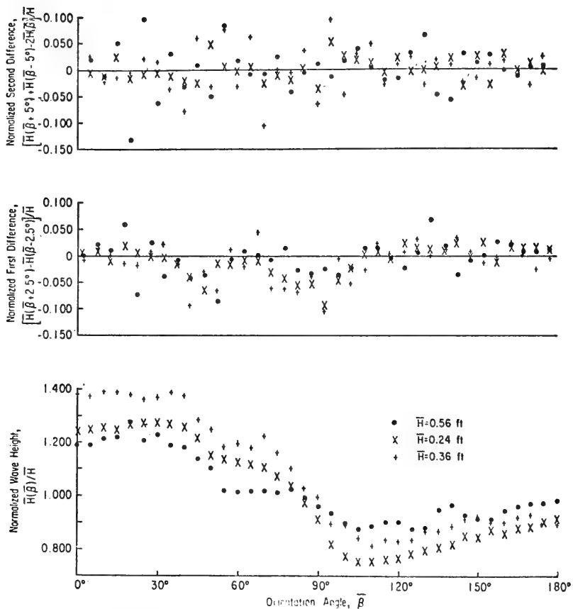
Figure 34. Normalized patterns of \overline{H}(\beta) and first and second angular differences for 2x2 H-pile in three situations; see Table 8 for test conditions.
