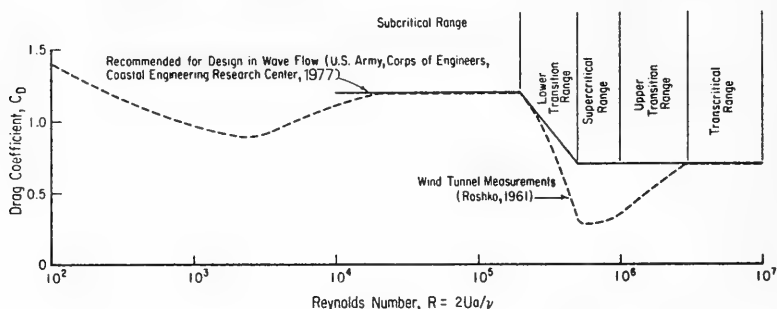
Figure 36. Flow regimes indicated by measured drag coefficient at a circular cylinder.
