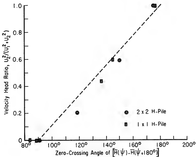
Figure D-4. Ratio of computed velocity heads of two orthogonal wave trains versus zero-crossing angle.
