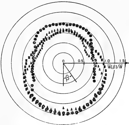
Figure 27. [\overline{W}(\beta)/\overline{W}] patterns for two H-piles and flat plate as \overline{W} increases. Test conditions: T = 2.32 seconds, d = 1.00 foot, G = 25 feet.
