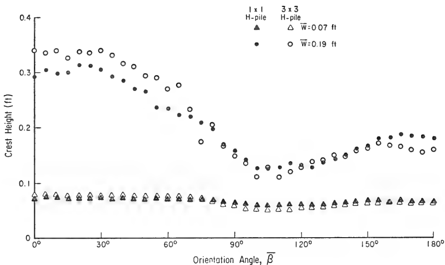
Figure 32. \bar{W}(\bar{\beta}) patterns for 1x1 and 3x3 H-piles. Test conditions: T = 1.55 seconds, d = 1.00 foot, G = 25 feet.
