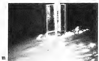
Figure 15. Photo sequence of wave crest incident into channel of 5x1 H-pile, with one-sixteenth second between successive frames. --Continued.
