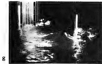
Figure 14. Photo sequence of wave crest striking side-by-side circular and finned circular piles, with one-eighth second between successive frames.
