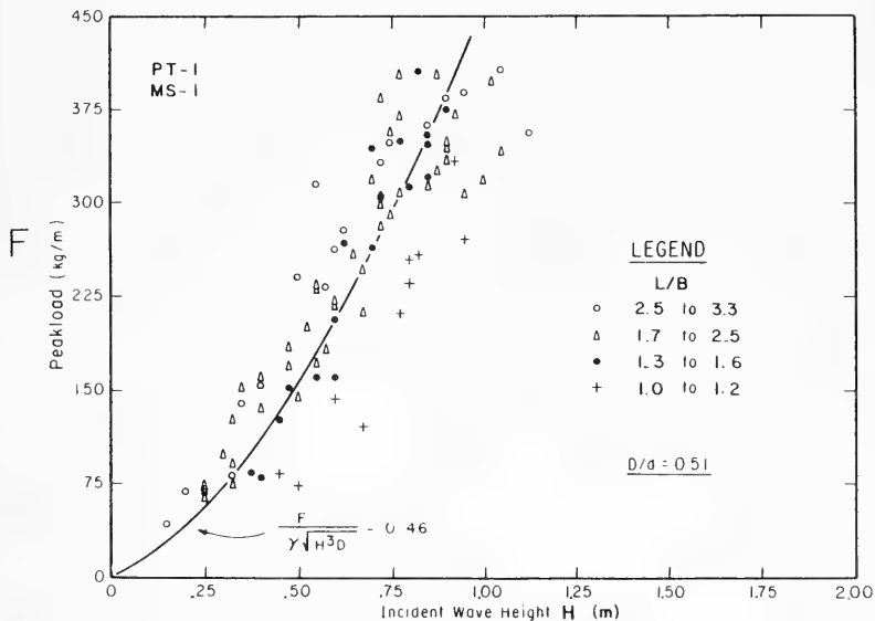
Figure 45. PT-1 peak mooring-force data (MS-1, d = 2.0 m).
