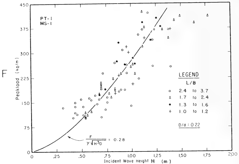
Figure 46. PT-1 peak mooring-force data (MS-1, d = 4.7 m).
