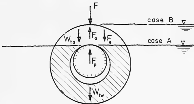
Figure 17. Forces on pipe-tire unit.
