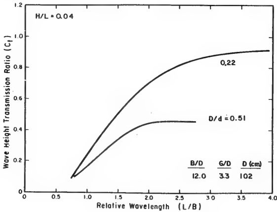
Figure 36. Wave transmission design curves for PT-1 breakwater.
