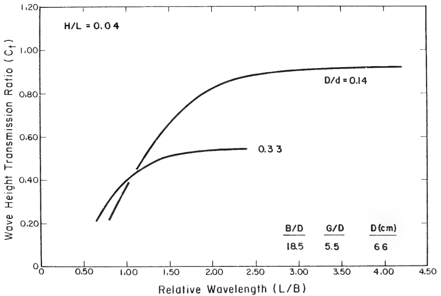
Figure 39. Wave transmission design curves for PT-2 breakwater.
