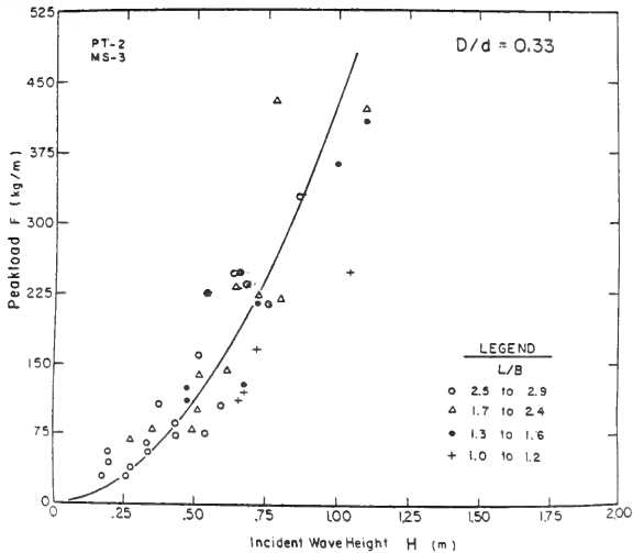
Figure 50. PT-2 peak mooring-force data (MS-3, d = 2.0 m).
