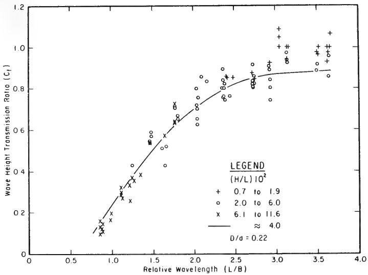
Figure C-1. PT-1 wave transmission data for MS-1.
