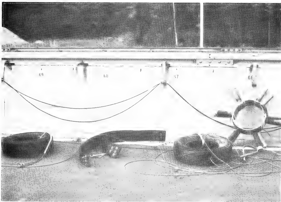
Figure 8. Breakwater and mooring-system components.
