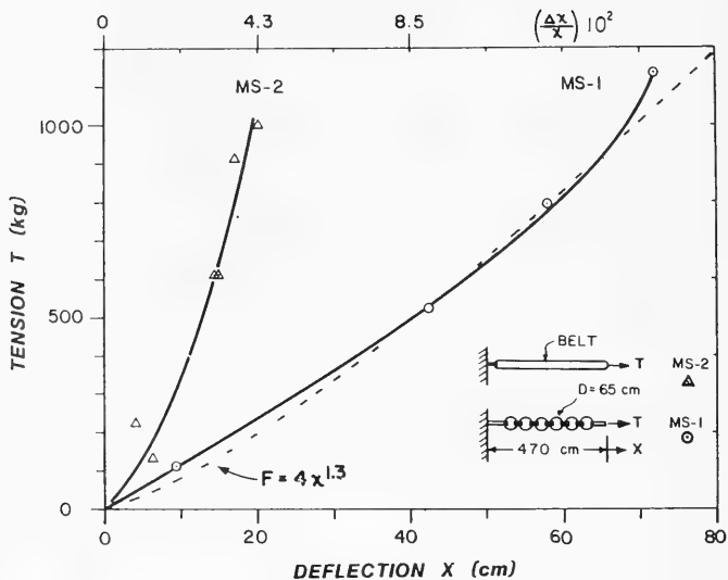
Figure 27. Load elongation curves for mooring-line inserts.
