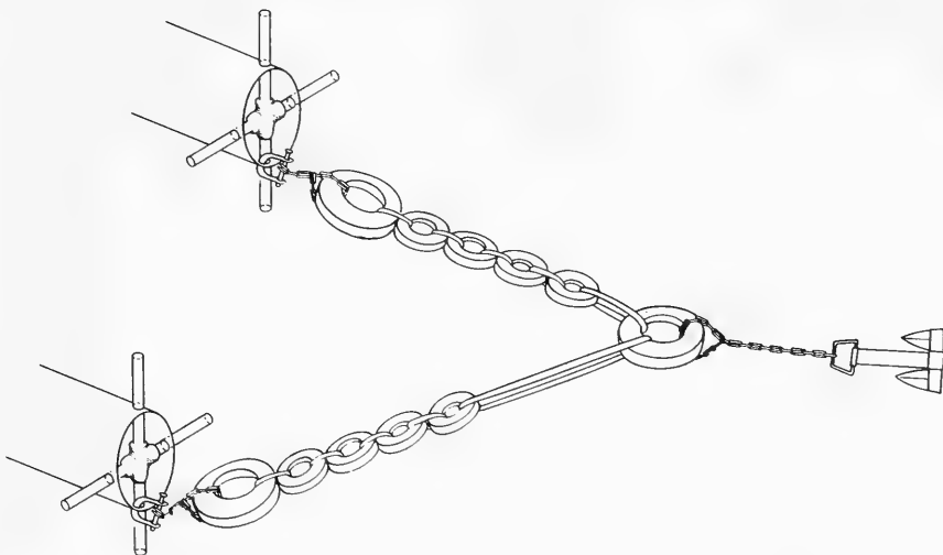
Figure 26. Mooring bridle used in field installation.
