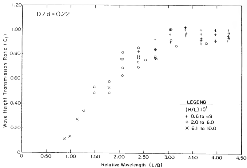
Figure C-3. PT-1 wave transmission data for MS-2.
