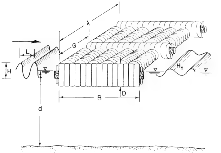
Figure 5. Definition sketch for PT-Breakwater.
