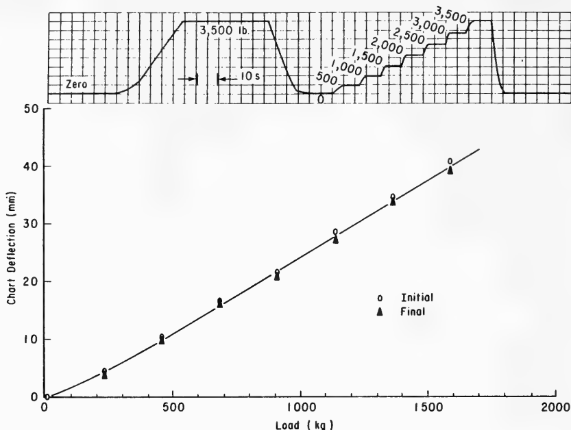
Figure 25. Force gage calibration record and curve.
