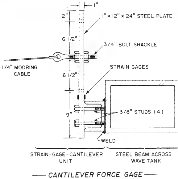
Figure 24. Strain-gage-cantilever force gage.
