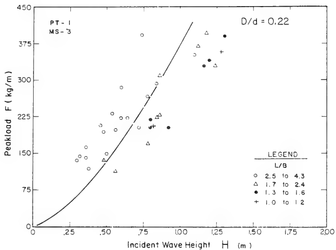
Figure 48. PT-1 peak mooring-force data (MS-3, d = 4.7 m).
