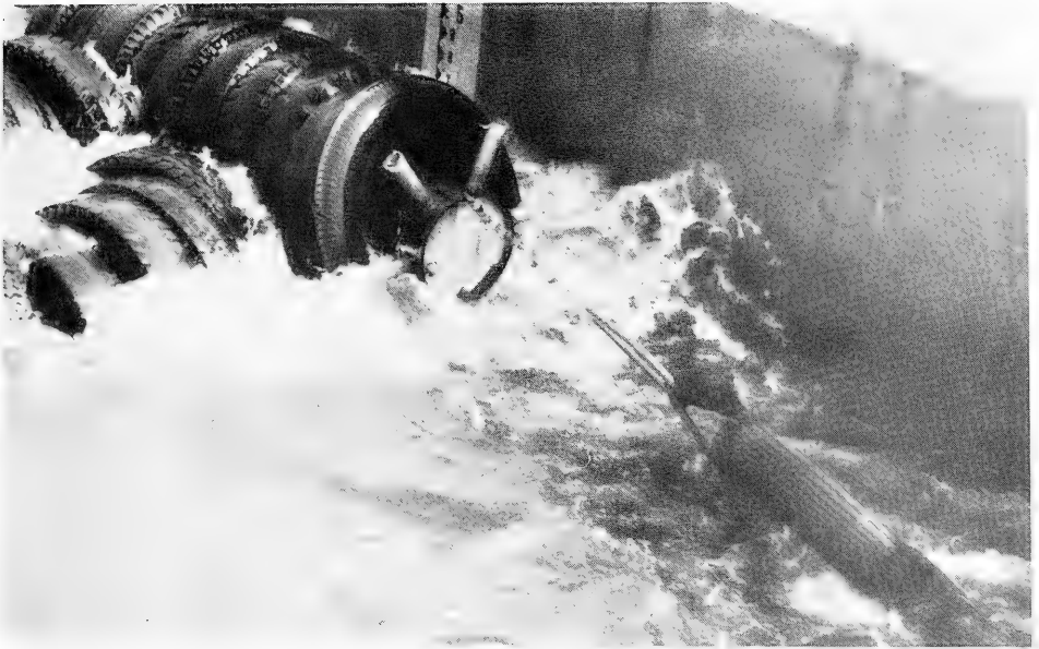
Figure 23. Attachment of seaward mooring line (MS-1 mooring system).
