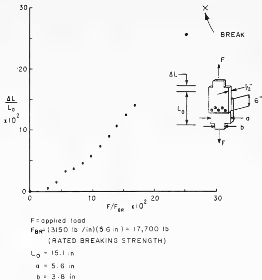
Figure 28. Stress-strain diagram for belt connection.
