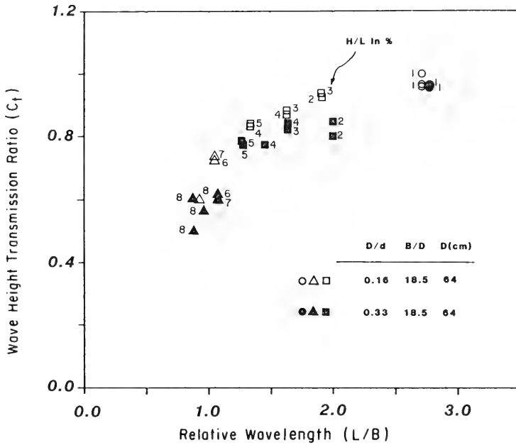
Figure 43. Influence of D/d on Goodyear wave attenuation.
