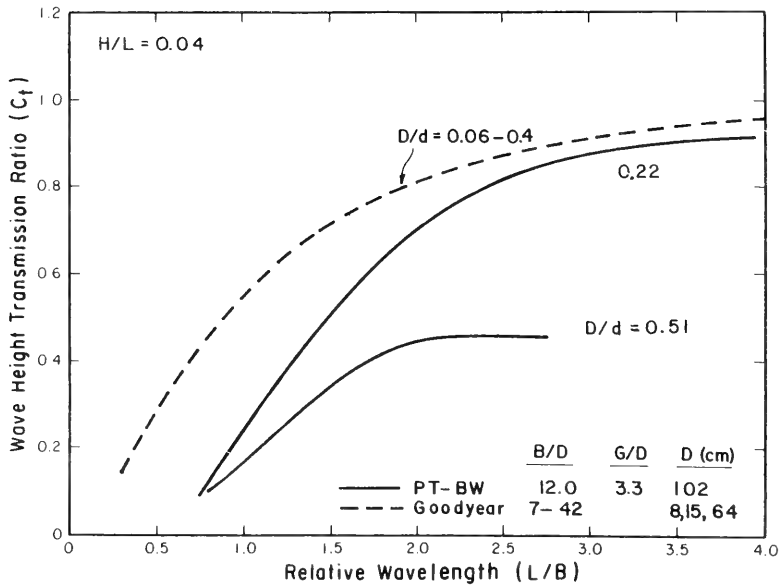
Figure 44. Wave transmission design curves for Goodyear and PT-Breakwater.
