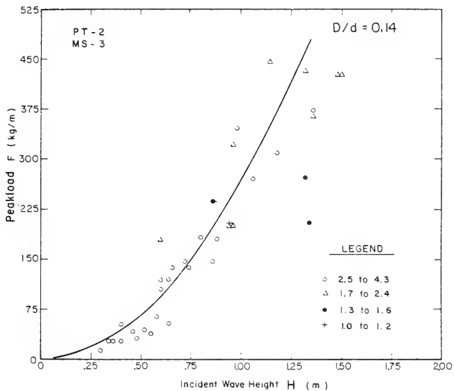
Figure 49. PT-2 peak mooring-force data (MS-3, d = 4.7 m).
