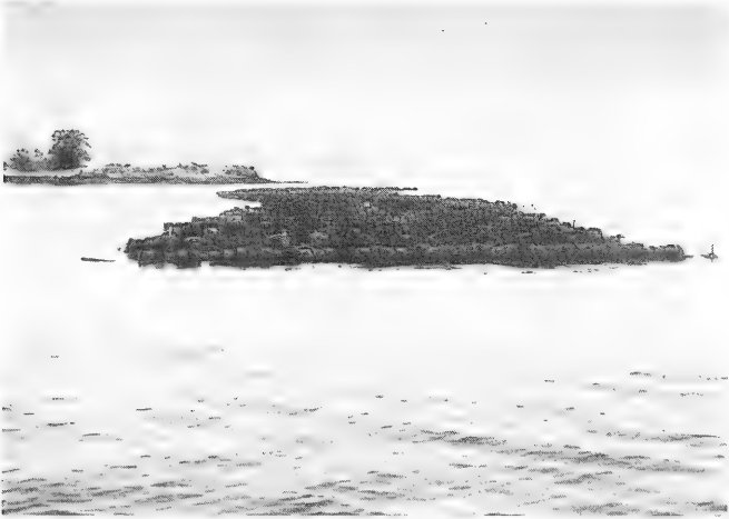
Figure 1. PT-Breakwater field installation (PT-1 modules; Mamaroneck, New York).
