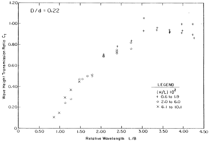
Figure C-5. PT-1 wave transmission data for MS-3.
