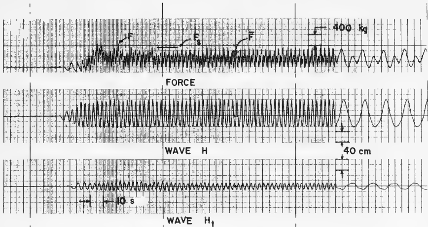
Figure 30. Wave and force record for short waves ( d = 4.7 m, T = 3.2 s).
