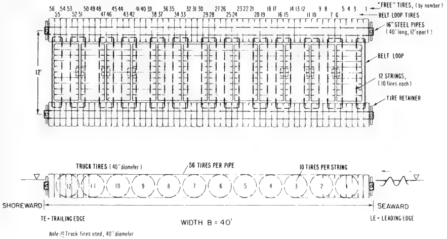
Figure 4. Schematic of PT-1 breakwater module.
