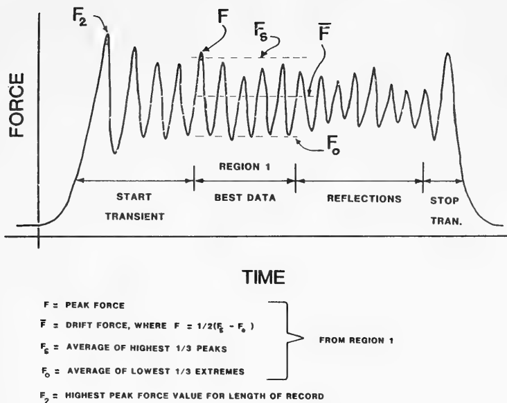
Figure 33. Definition sketch for force analysis.
