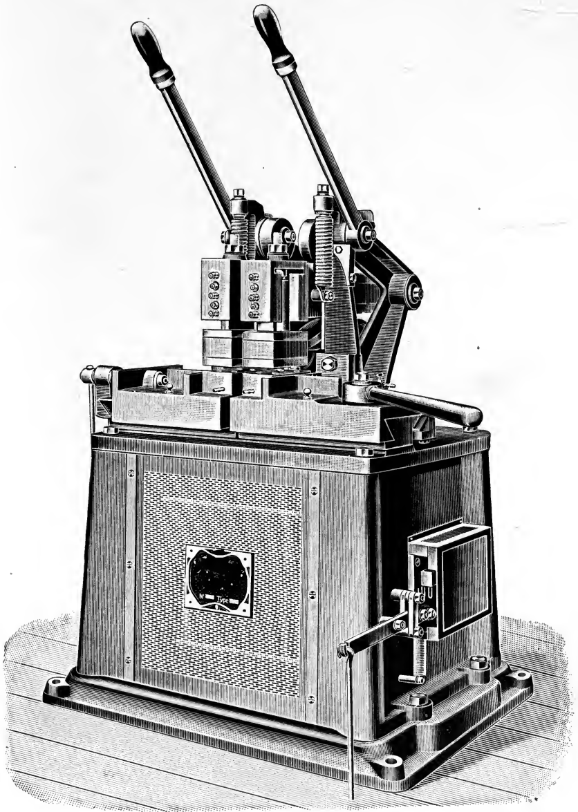
FIG. 33.—Universal Machine, Normal Pattern, without Swages.
