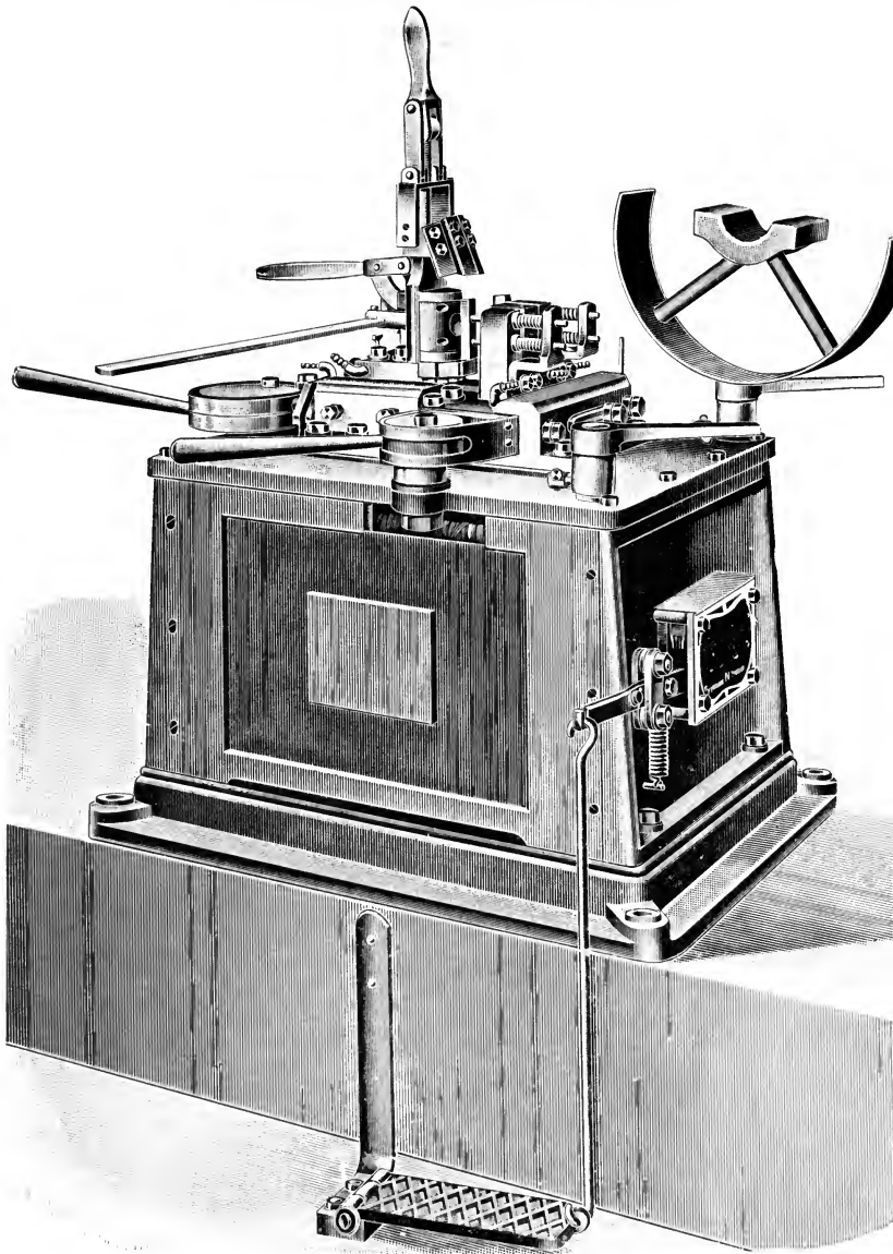
FIG. 45.—Machine for Welding Pulley-spokes to Rim and Hub.
