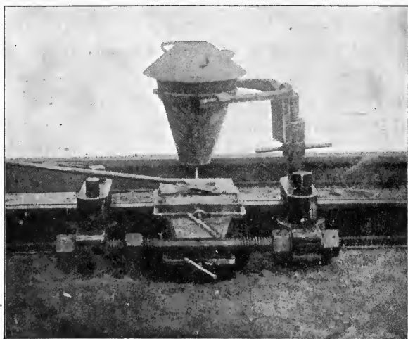
FIG. 22.—Complete Rail Welding Outfit.
