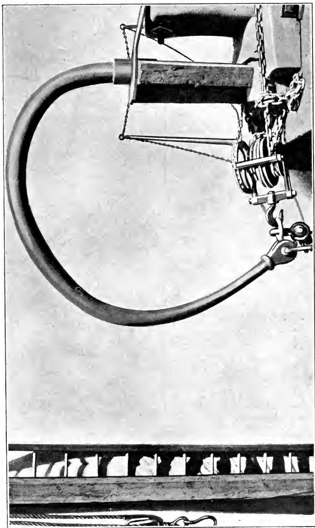
FIG. 94.—Binding Tests of Welded Boots Davits. The Imperial Arsenal, Dantzig.
