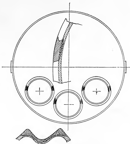
FIG. 102.—Repairs by Oxy-Acetylene Process.
