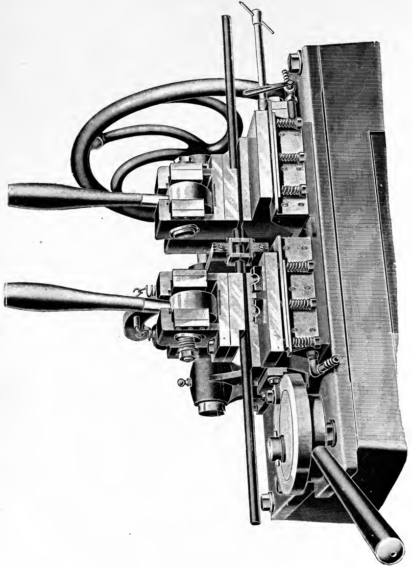
FIG. 32.—Universal Welding Machine for Welding or for Electrically Heating Pieces for Subsequent Working, with Swages, Hand-operated.
