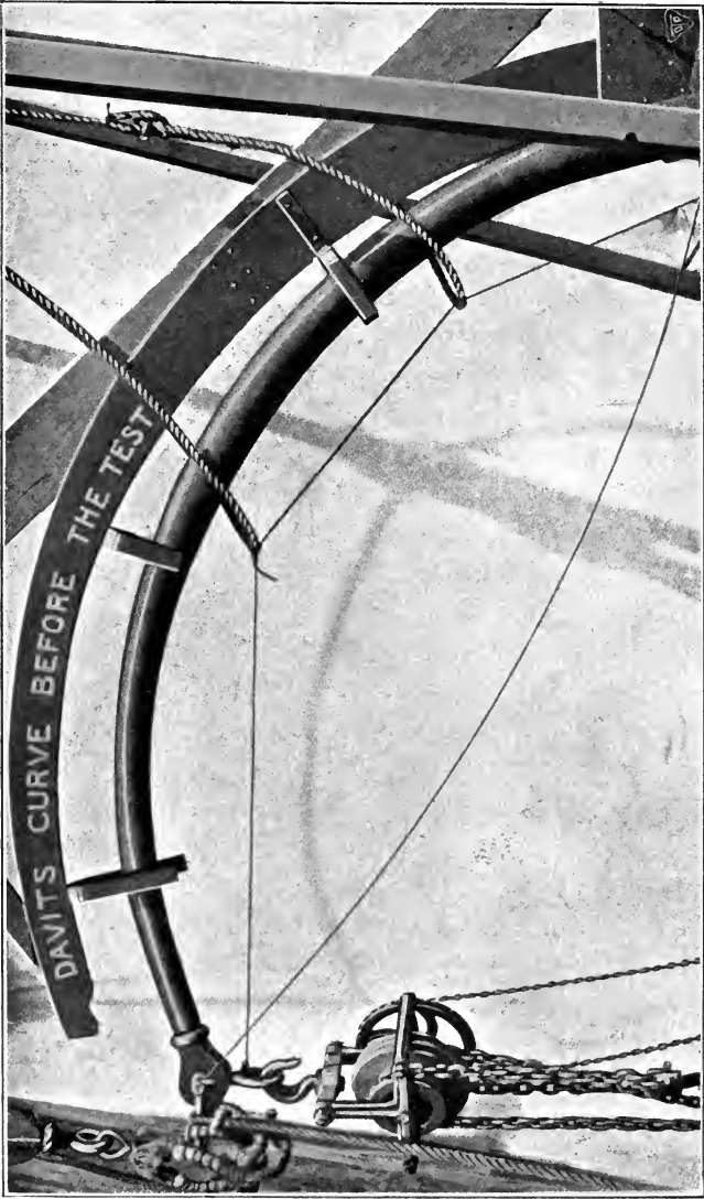
FIG. 93.—Bending Tests of Welded Bootsdavits. The Imperial Arsenal, Dantzig.
