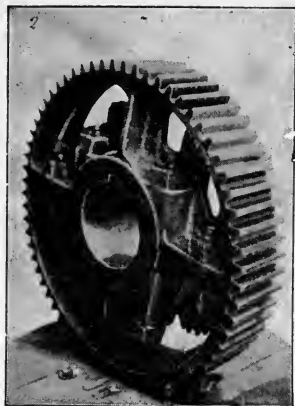
FIG. 25.—Finished Repair.
