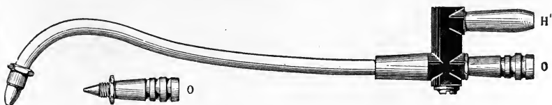
FIG. 29.—Oxy-Coal Gas Blowpipe.
