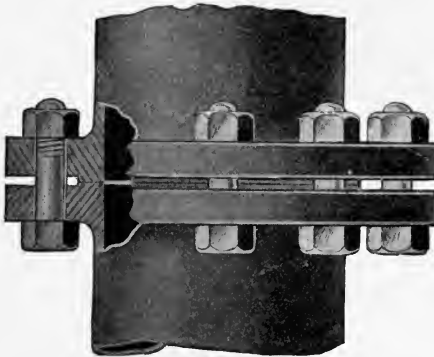
FIG. 59.—Facing Strips.
