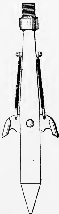
FIG. 19A.—EXPANDING TOOL FOR TRIMMING BORE-HOLE BELOW TUBES.
