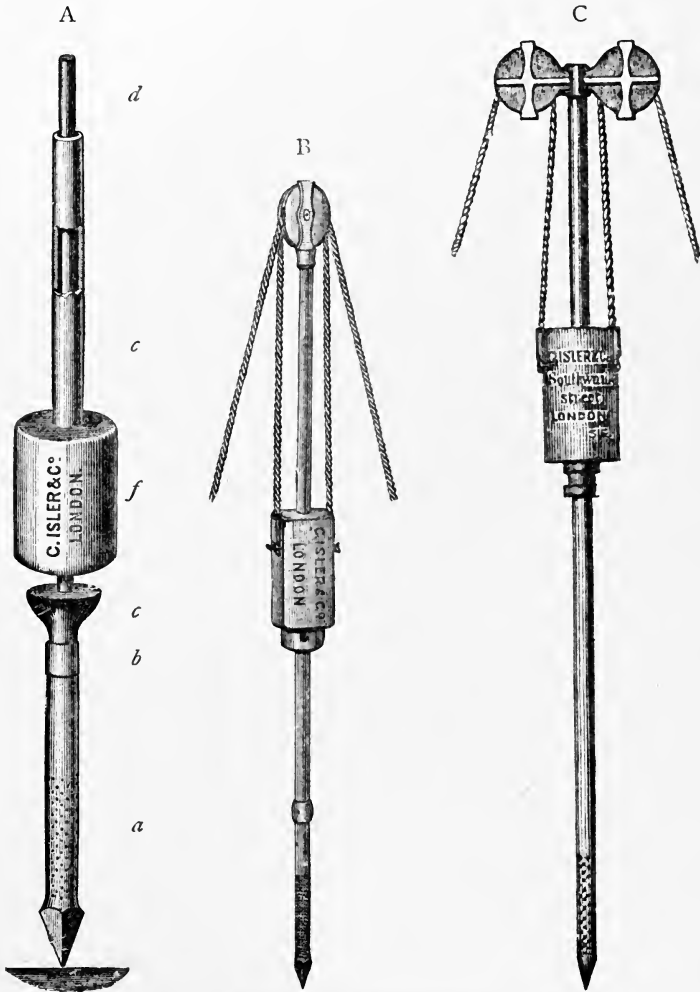
FIG. 8.—DRIVING TUBES.
