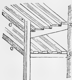
Fig. 25. Section showing the arrangement of the Shelves.
