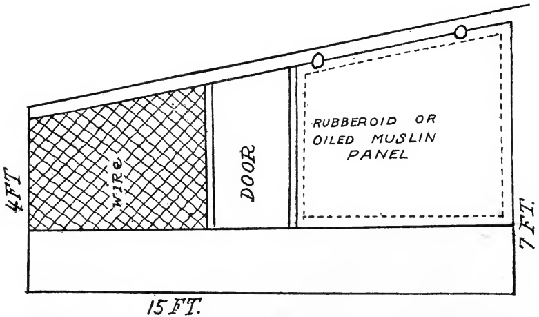
Hoffman's Combination Open Front House and Scratching Pen
