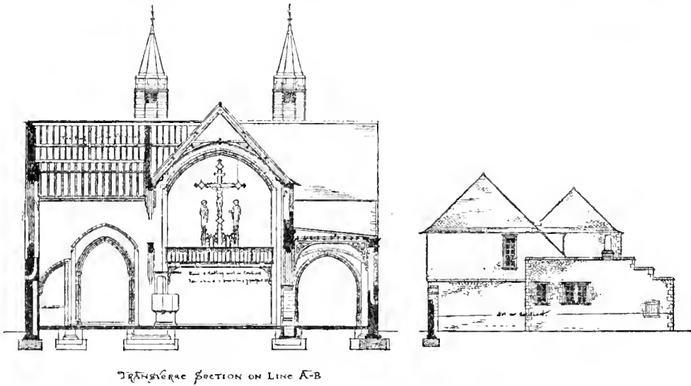
FIG. 39.—CHURCH OF THE HOLY ROAD, WATFORD: (1) LONGITUDINAL SECTION. 2. TRANSVERSE SECTION.
