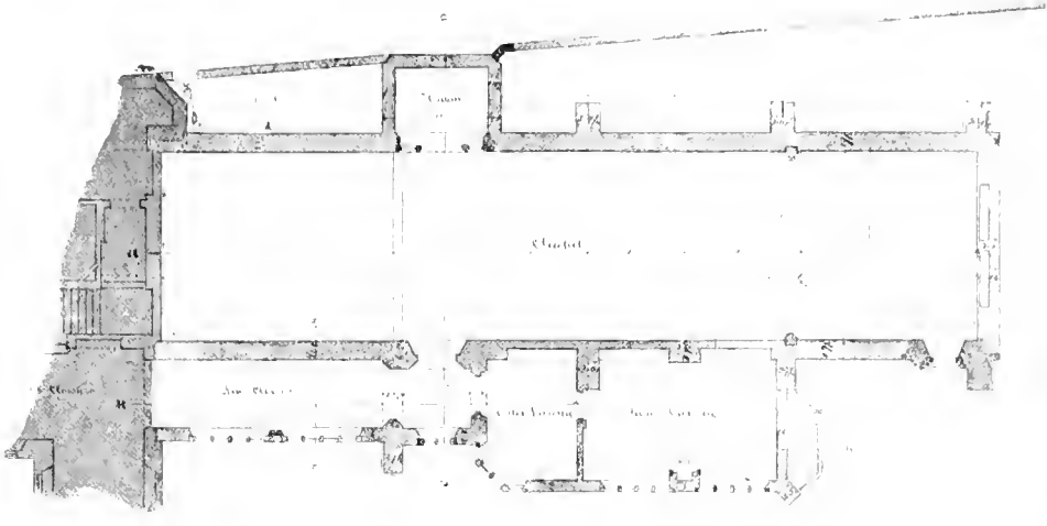
PLATE LXX.—S. THOMAS'S SEMINARY, HAMMERSMITH. A. ORIGINAL GROUND PLAN OF MAIN BUILDING. B. CHATEL PLAN SHOWING ADDITIONS TO ORIGINAL CLOISTER.
