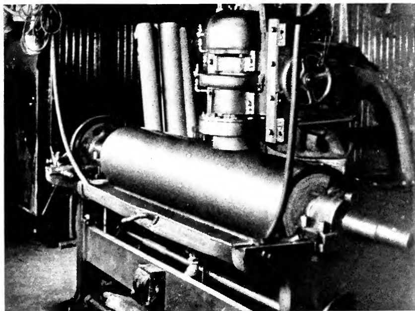
AFTER the COLORoto Magazine is printed, the copper cylinders are re-surfaced so that another set of pages may be etched. The cylinder was made by depositing copper on a steel core in an electrolytic bath.
