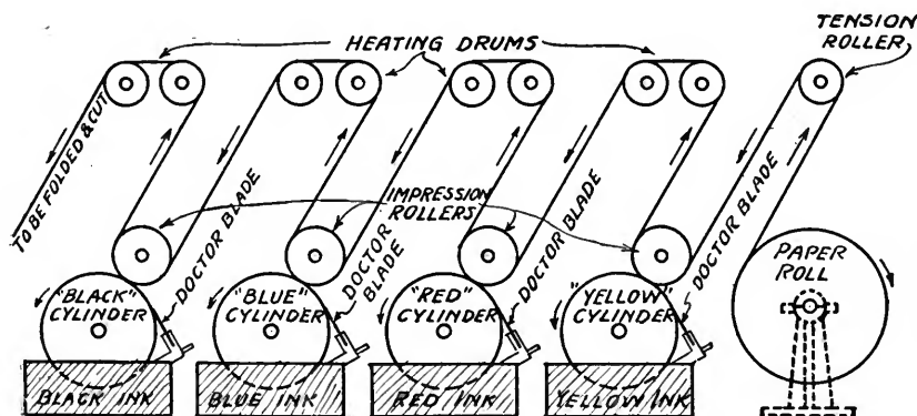
Diagram showing the passage of paper through the COLORoto press.
