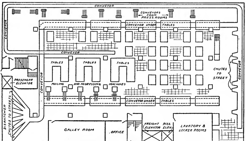
FLOOR PLAN of Mailing Room
