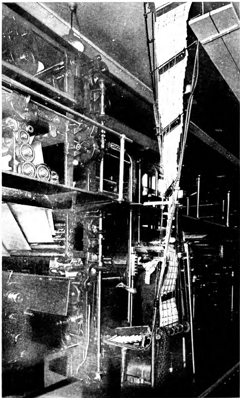
This pictures the peculiar conveyor which takes the folded Tribunes from the foot of the presses up through the ceiling to the mailing room on the floor above. From there they are swiftly distributed throughout Chicago and to more than seven thousand other towns and cities.
