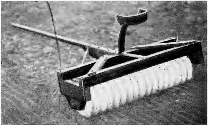
Fig. 18.—A successful cement, home-made roller.
